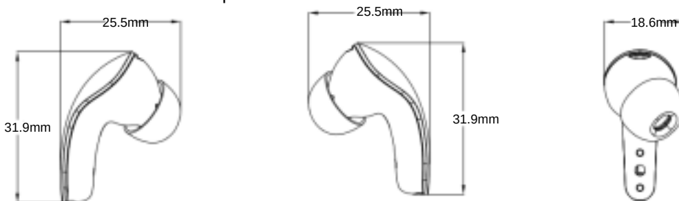
Earphone
