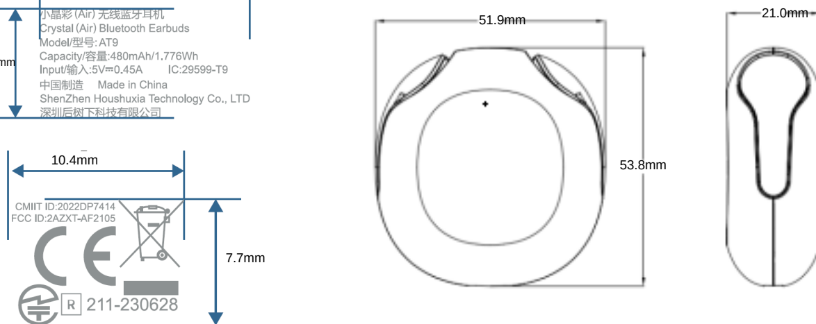
Charging case
