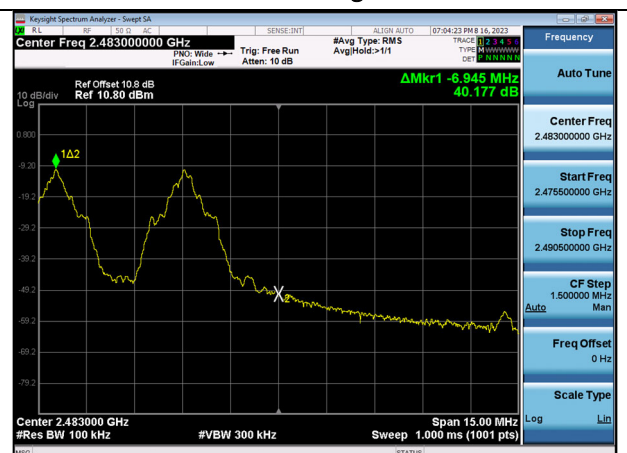
GFSK(with hopping) Band Edge
