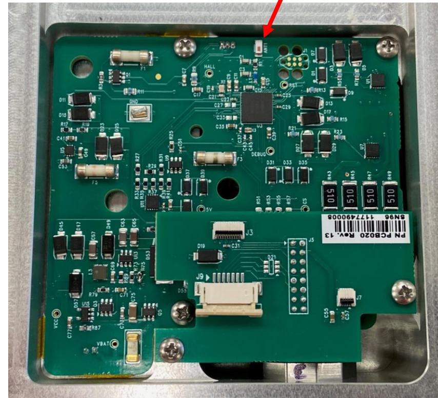
Circuit Boards as installed close-up (Plate and Cover unstalled for photo)
