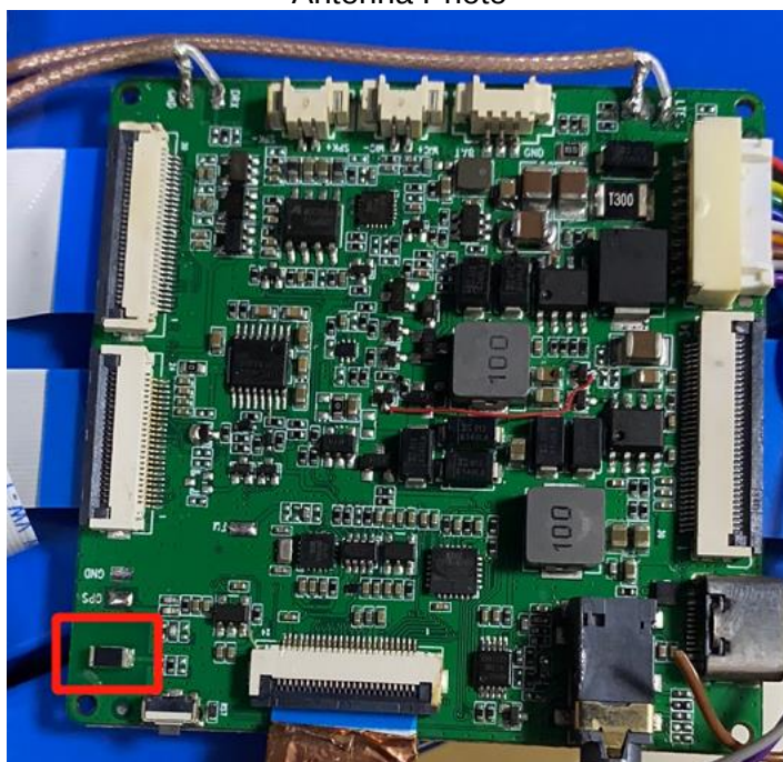
Antenna Photo
