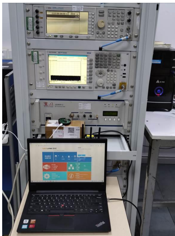
Test Setup Photo of Dynamic Frequency Selection Test
