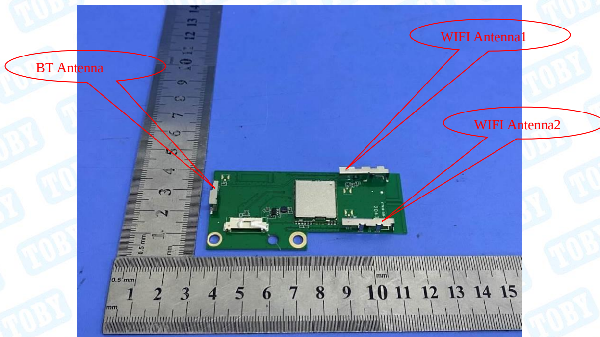
Photo 20 Appearance of PCB
