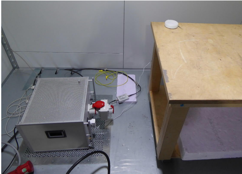
AC Mains conducted emissions setup for EUT1 with PA 1
