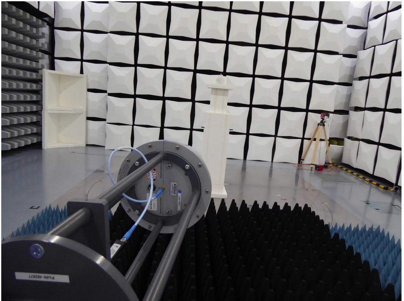
Test setup 1 – 4 GHz
