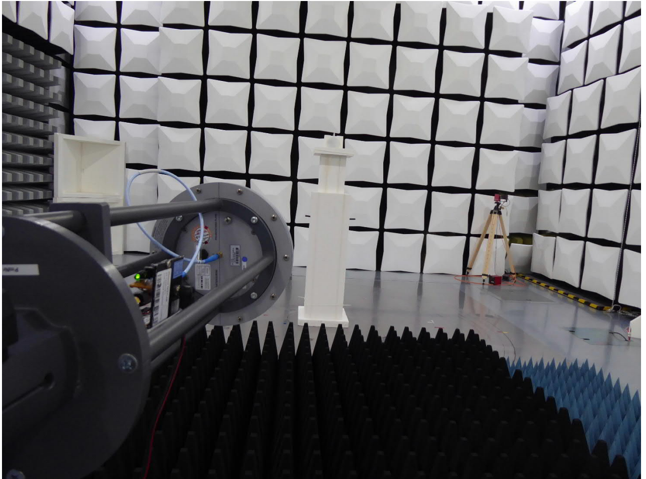
Test setup 4 – 10 GHz
