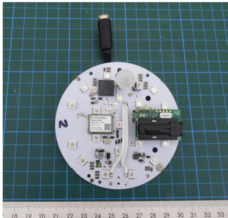
EUT 2 - PCB internal view
