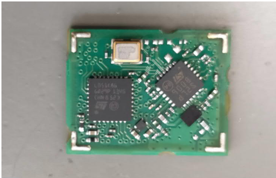
RF Modul without shielding provided by the applicant
