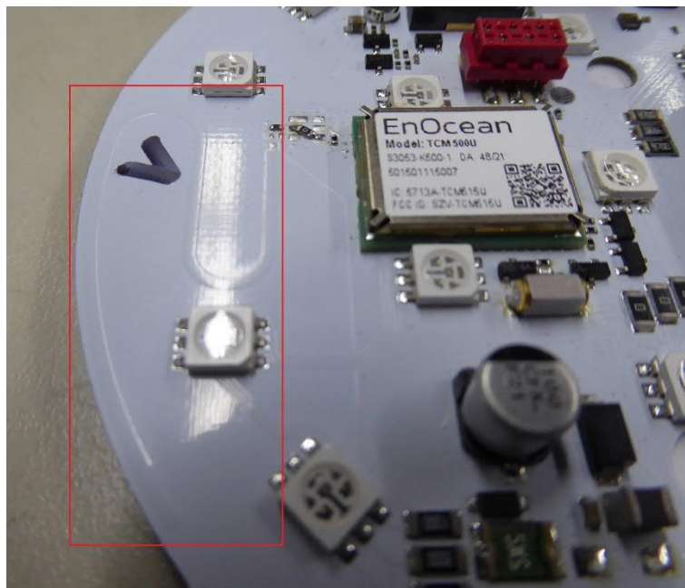
PCB Antenna
