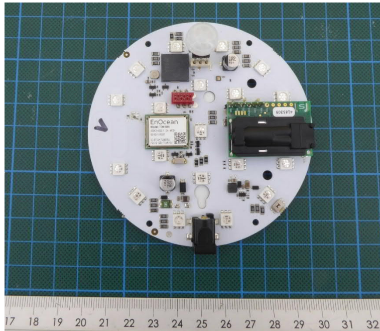
EUT 1 – PCB internal Top view
