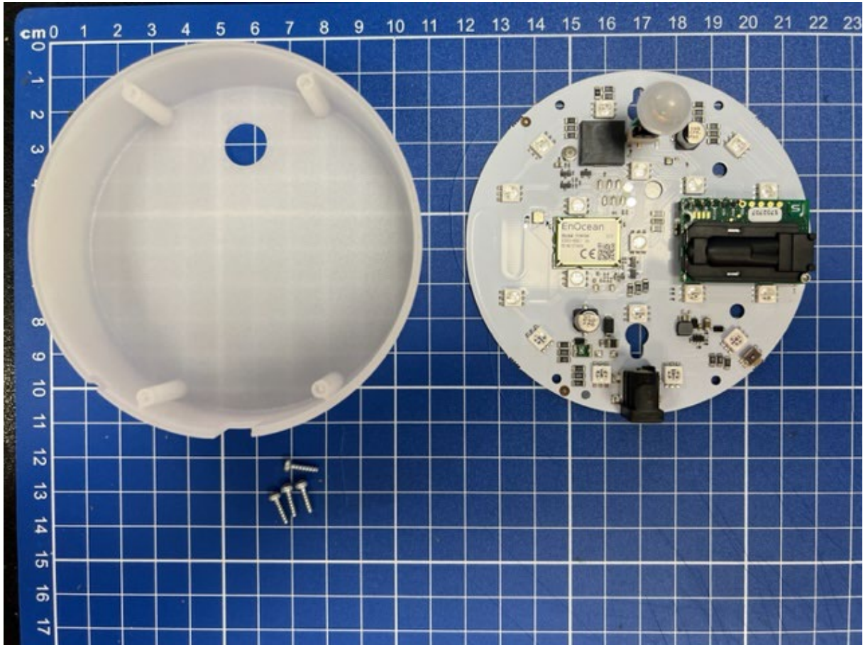
Figure 1: Internal, top view of PCB with housing
