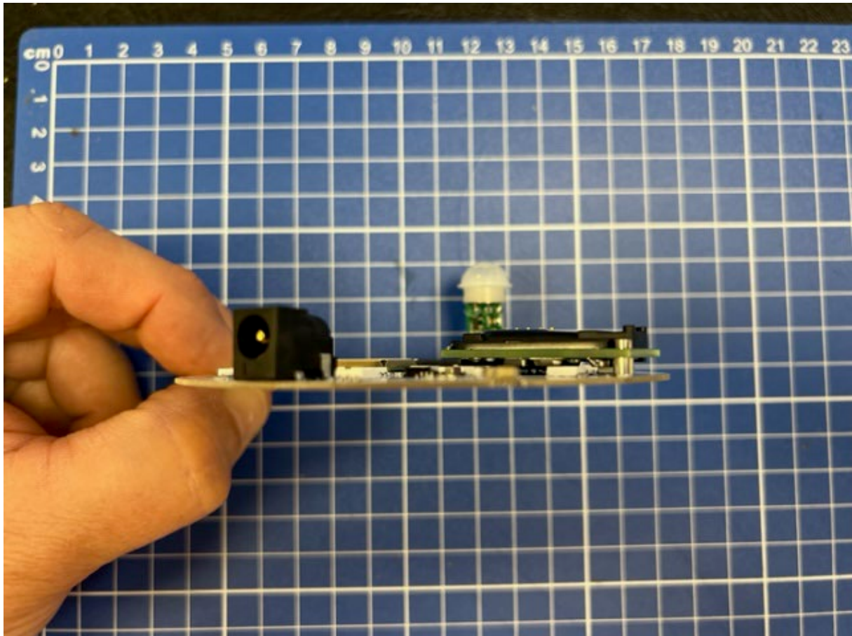
Figure 4: Side view of PCB, power connector
