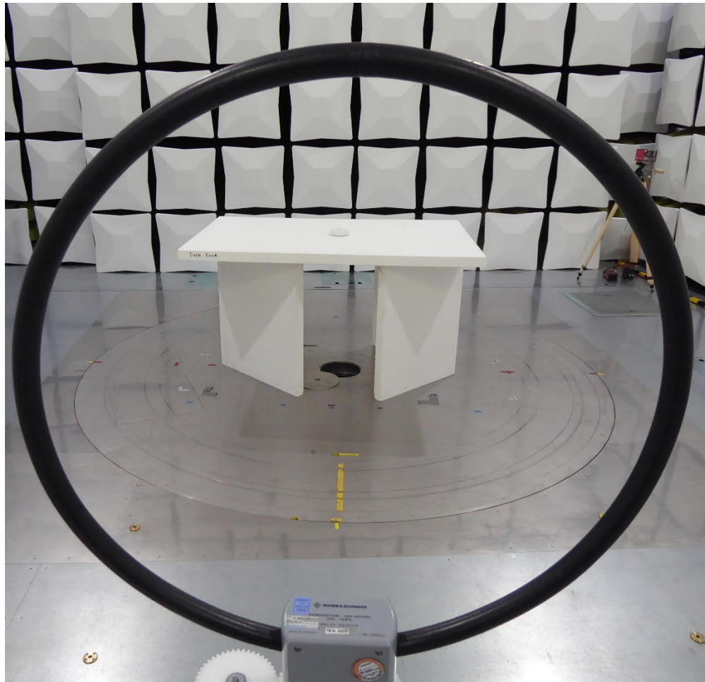
Test setup 9 kHz to 30 MHz
