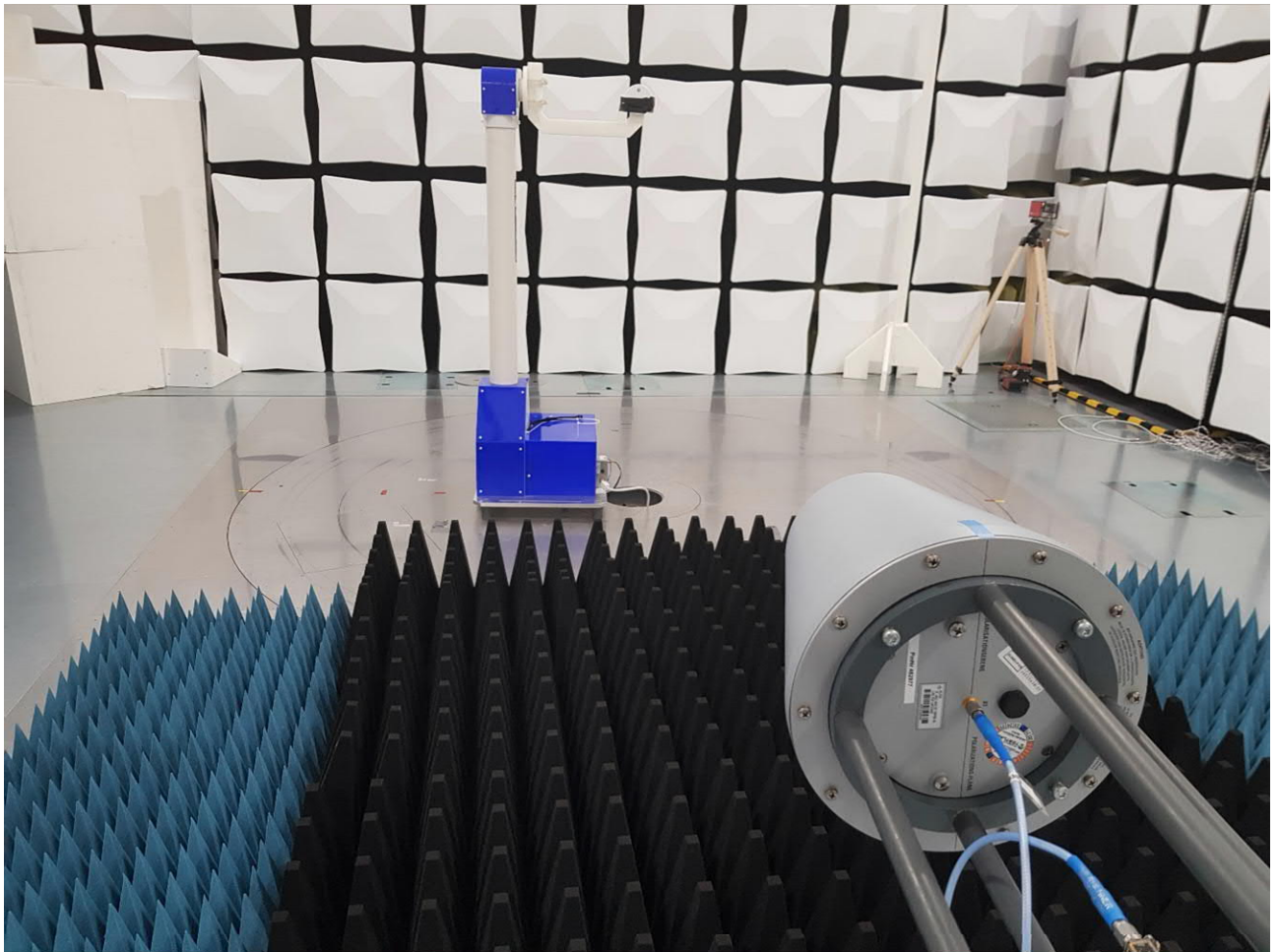
Test setup 1 GHz – 10 GHz
