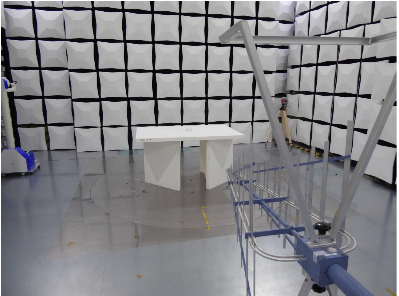
Test setup 30 MHz to 1 GHz
