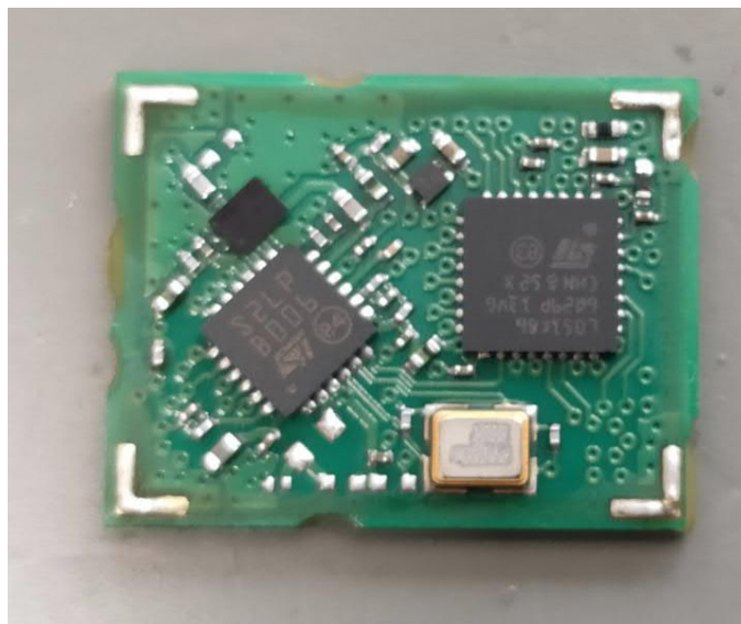
RF Modul without shielding provided by the applicant
