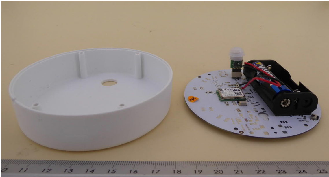
EUT Internal view
