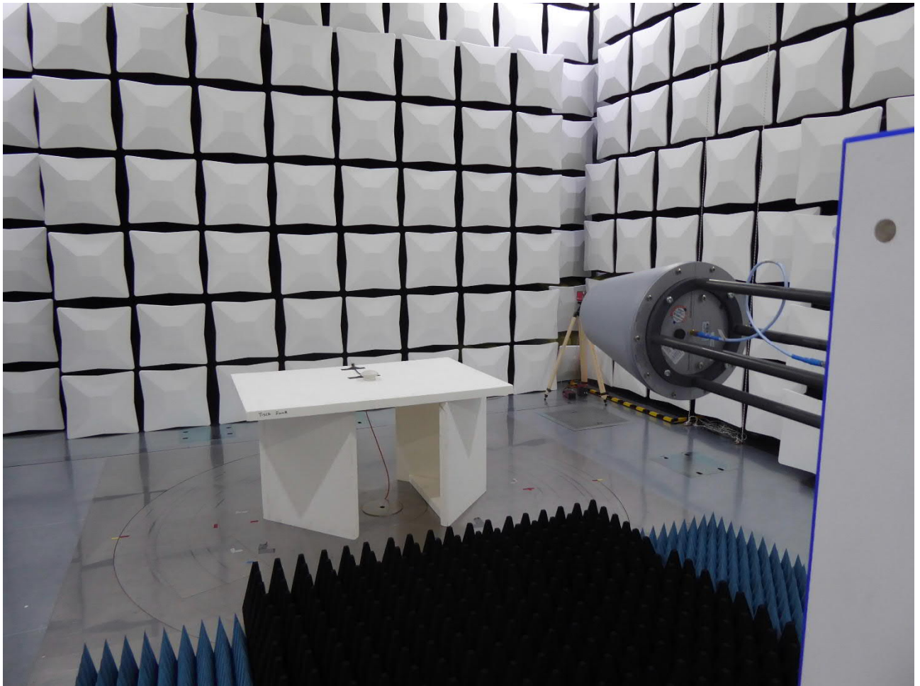
Test setup 1 – 5 GHz
