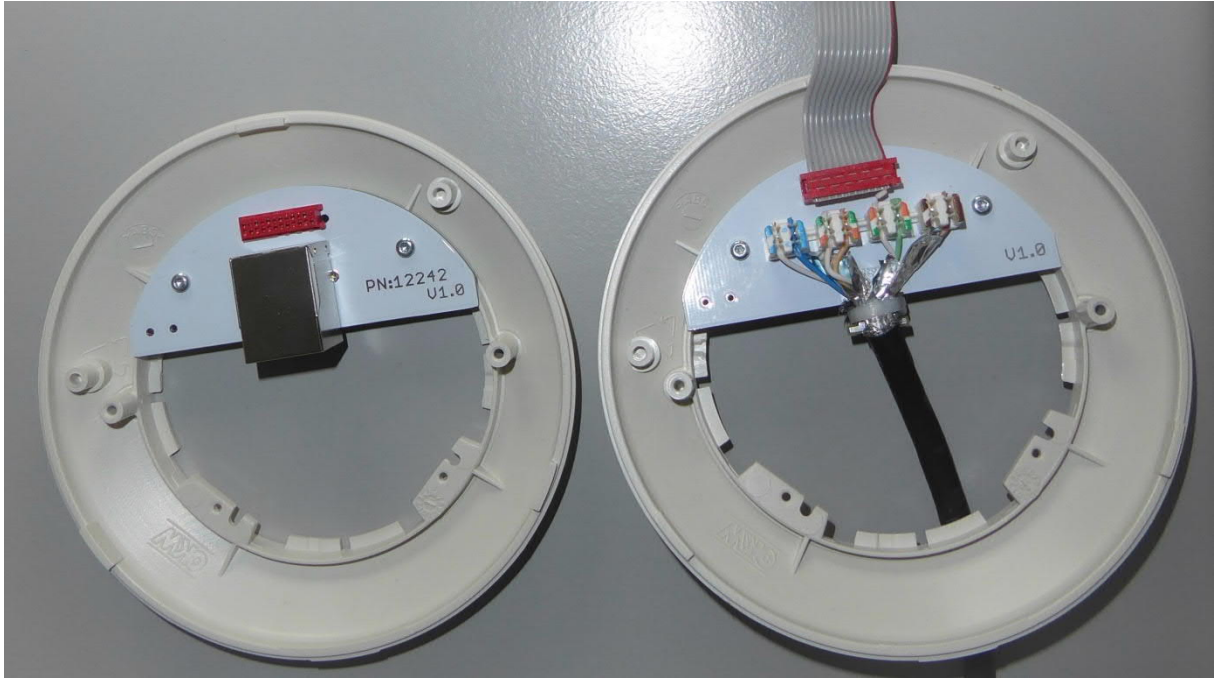
Bottom view of Connector boards
