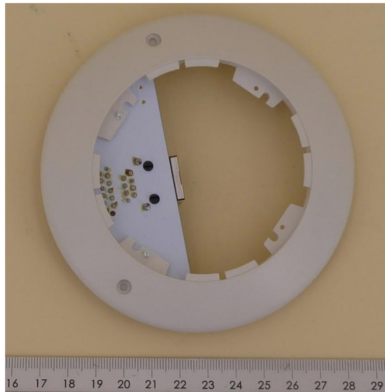
Top view of connector board
