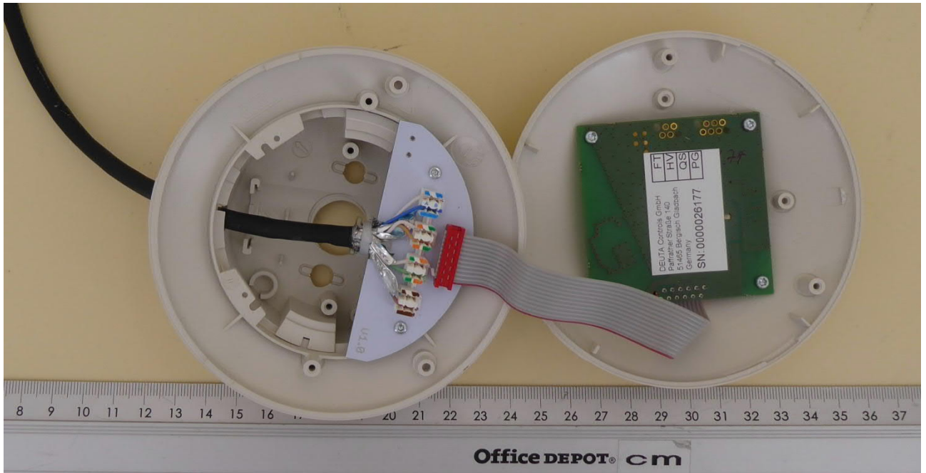
PCB internal view
