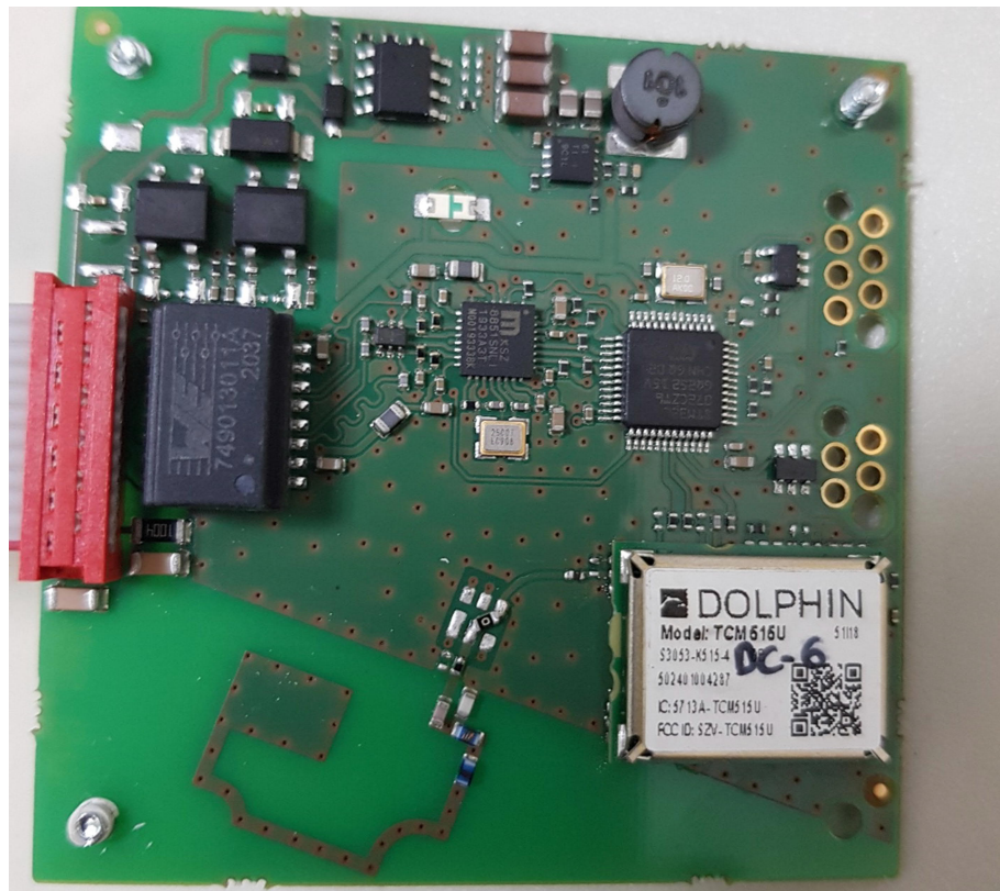
Controller board PCB Top view
