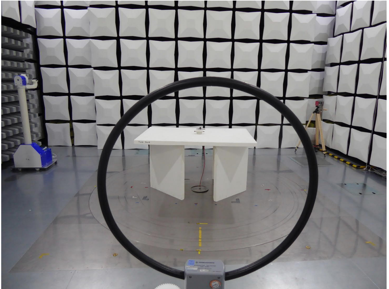
Test setup 9kHz to 30 MHz
