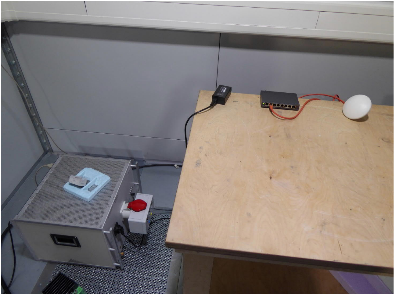
AC Mains conducted emissions setup for EUT with connector board 2
