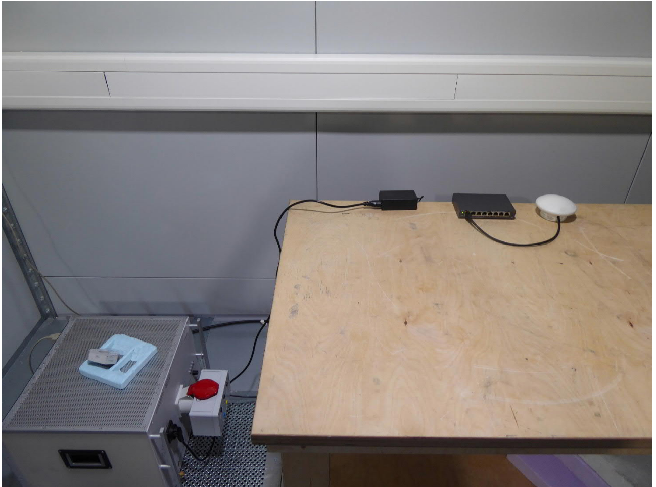
AC Mains conducted emissions setup for EUT with connector board 1
