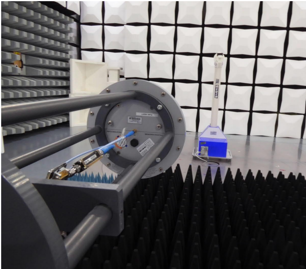
Test setup 4 GHz – 10 GHz
