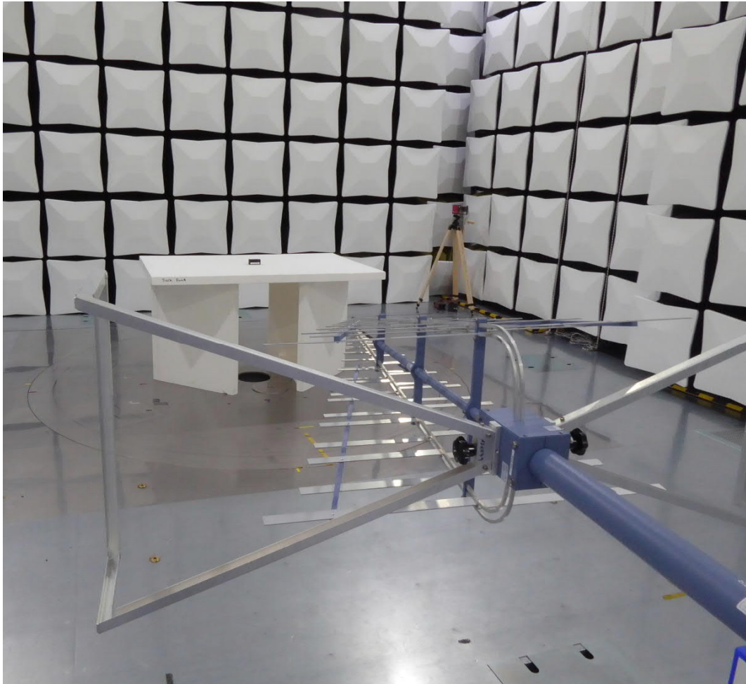
Test setup 30 MHz to 1 GHz
