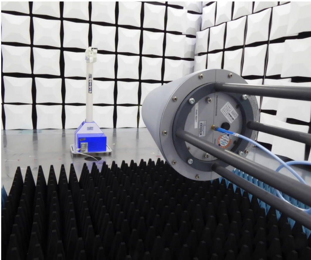
Test setup 1 GHz – 4 GHz
