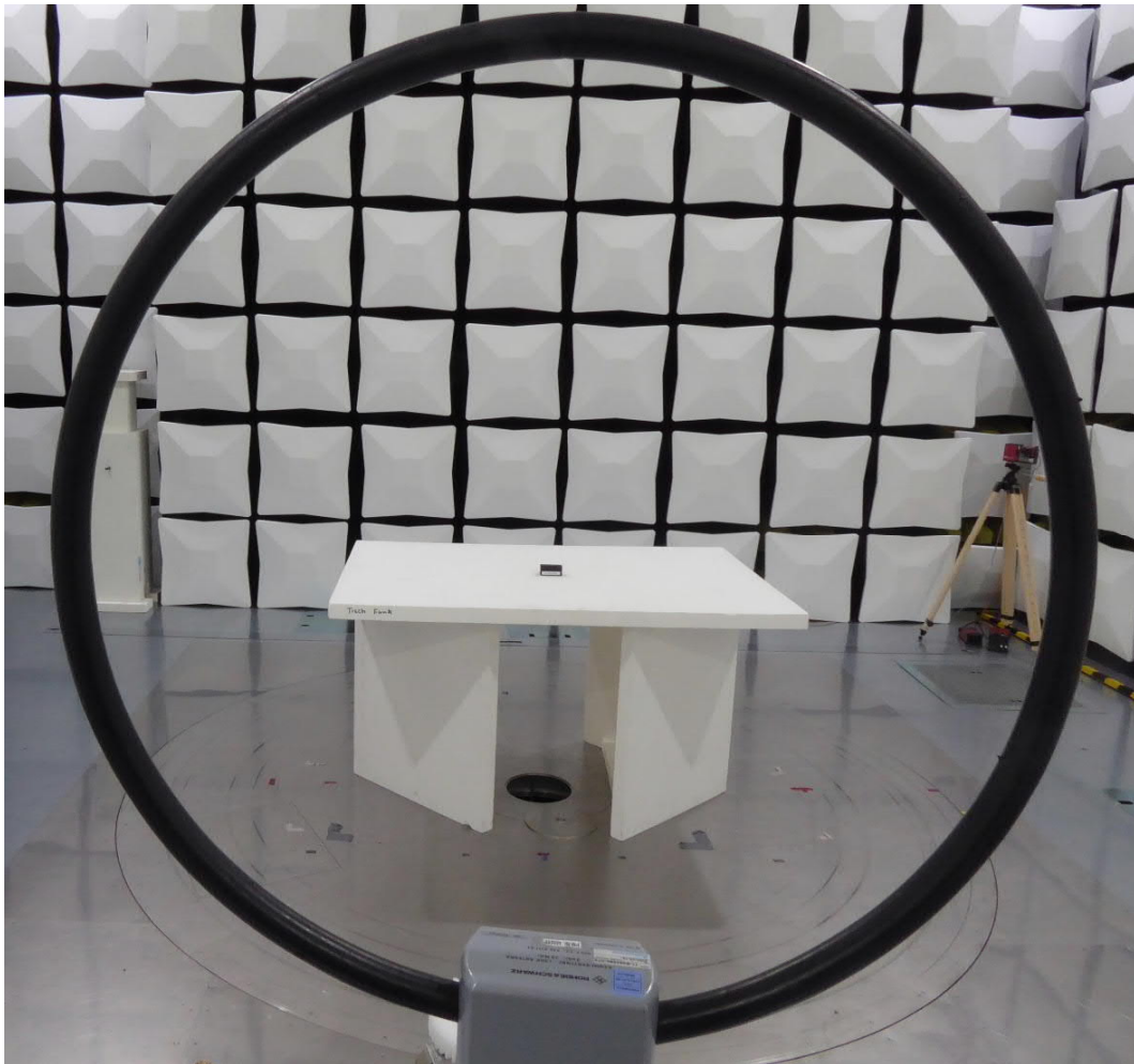
Test setup 9 kHz to 30 MHz
