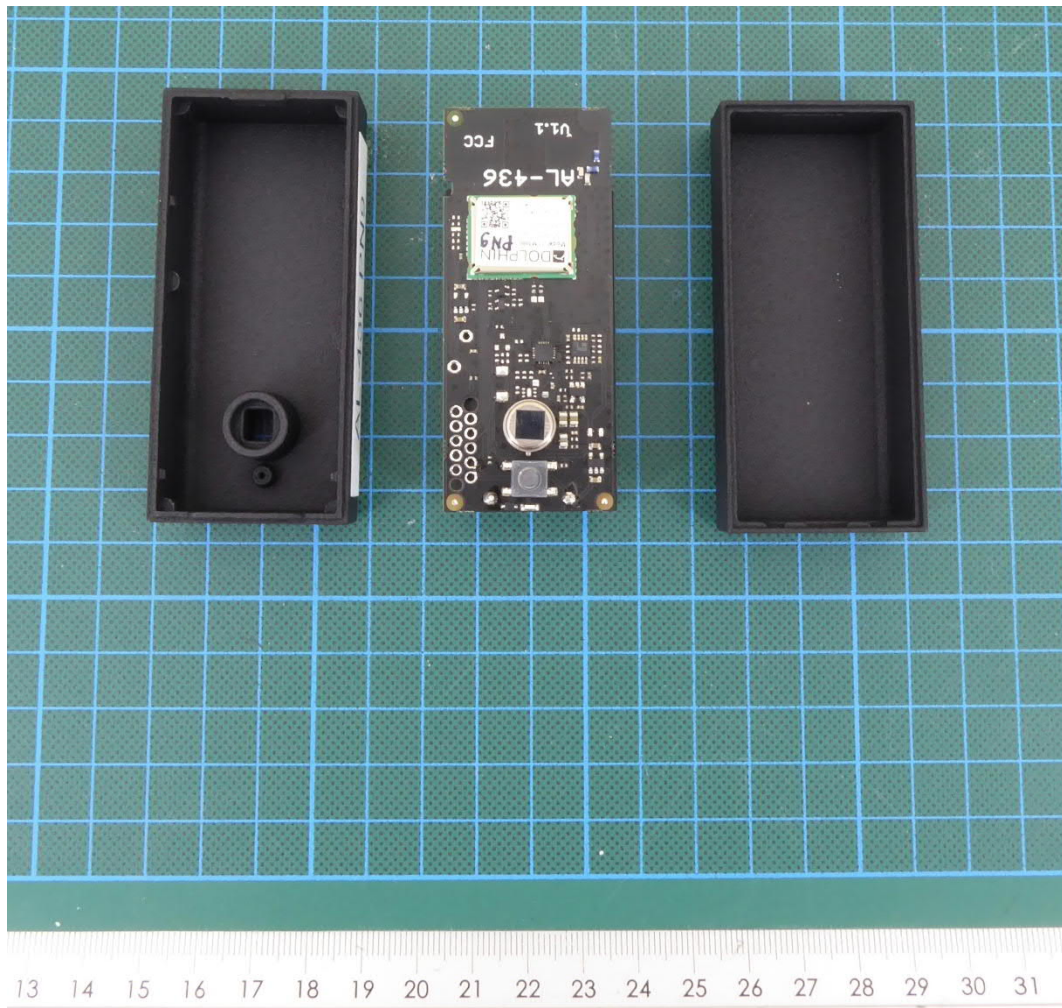
PCB top view
