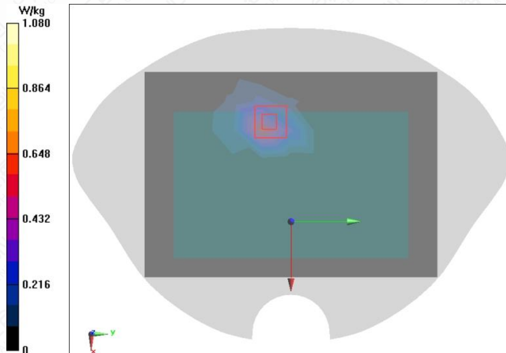
Figure A.1-5 Wi-Fi 5G 802.11a Left Side-2 Mode Middle 0mm
