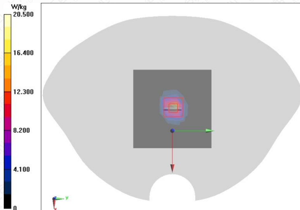
Figure A.2-5 System Check 5800MHz
