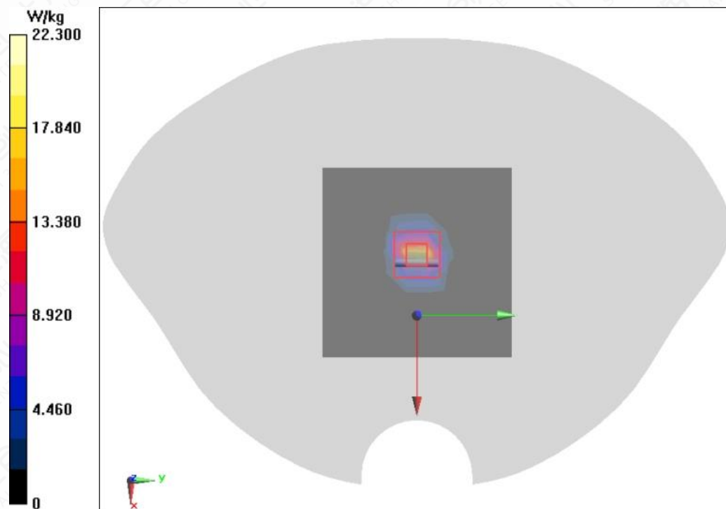
Figure A.2-4 System Check 5600MHz
