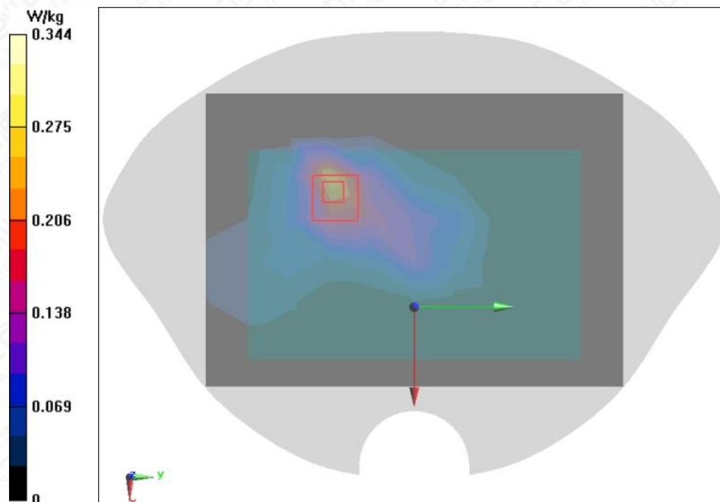
Figure A.1-1 Wi-Fi 2.4G 802.11b Left Side-2 Mode High 0mm
