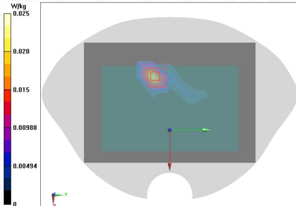
Figure A.1-6 BT 3DH5 Left Side-2 Mode High 0mm
