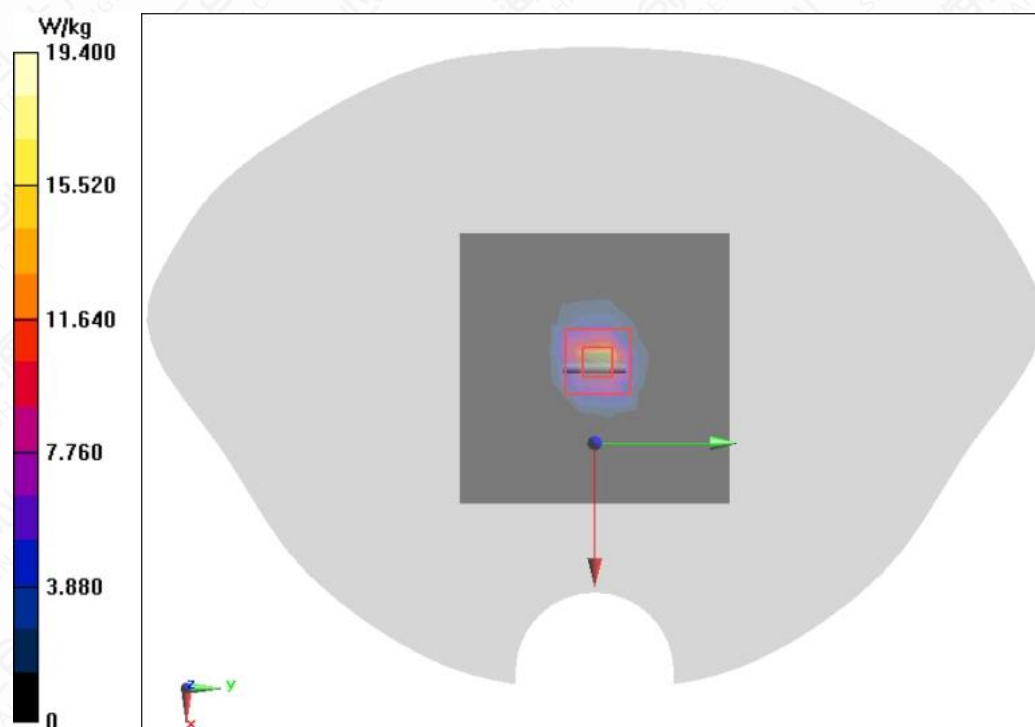
Figure A.2-2 System Check 5200MHz
