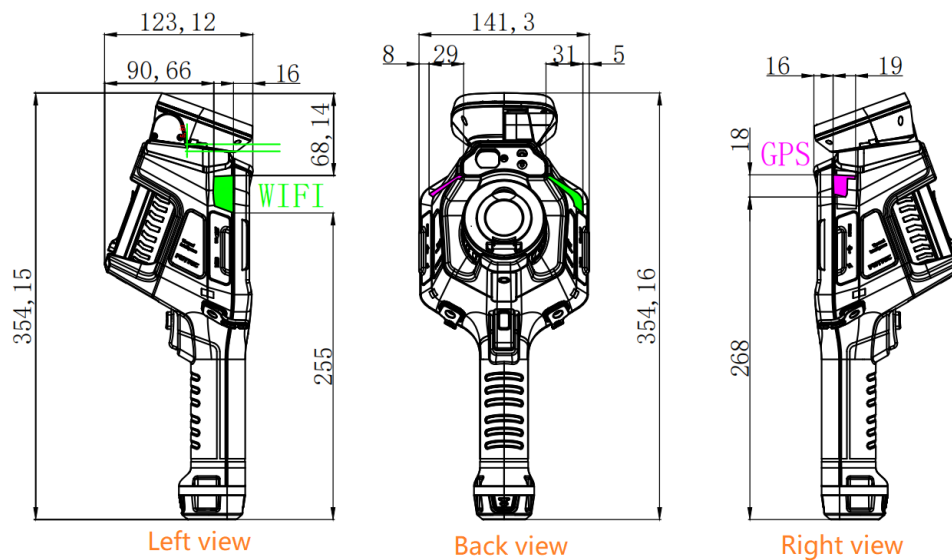
Figure 12.2-1 Antenna Locations
