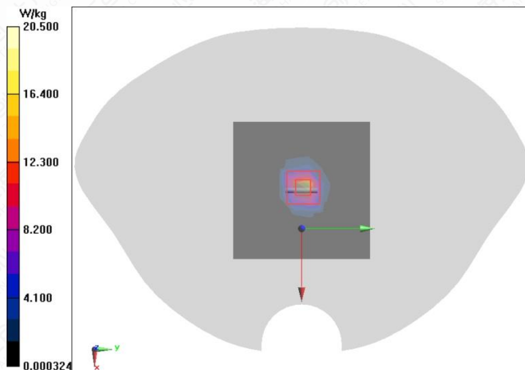
Figure A.2-3 System Check 5300MHz
