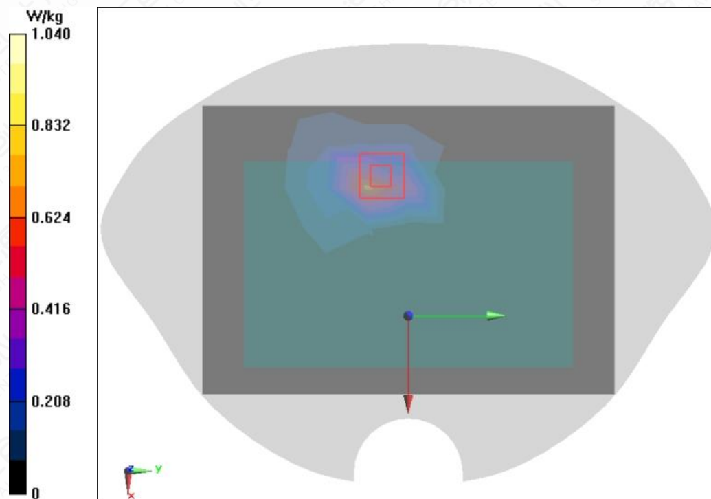
Figure A.1-4 Wi-Fi 5G 802.11a Left Side-2 Mode High 0mm
