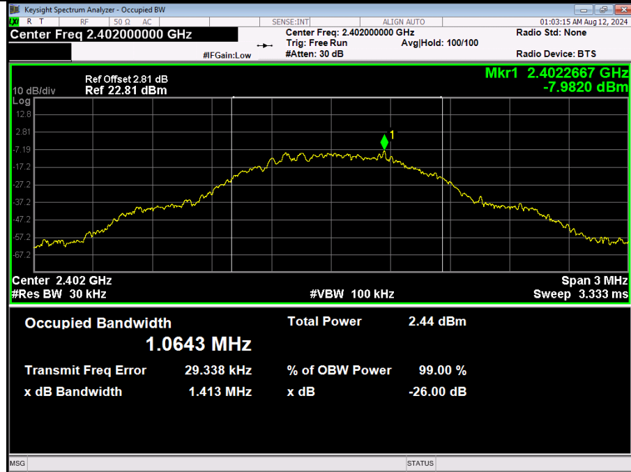
99% Occupied Bandwidth NVNT ANT1 1Mbps 2402
