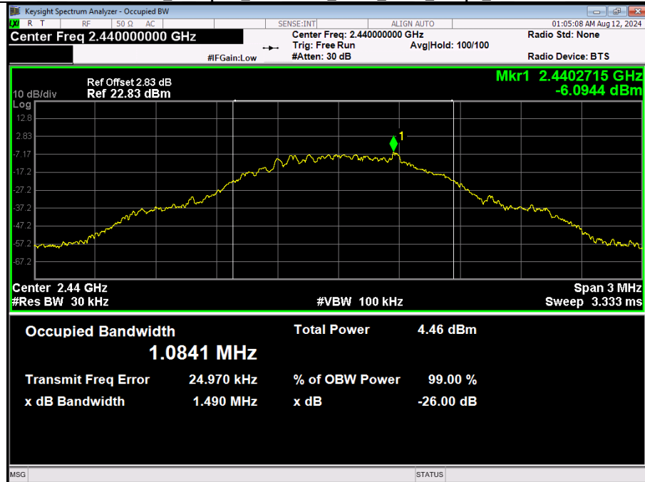
99% Occupied Bandwidth NVNT ANT1 1Mbps 2440
