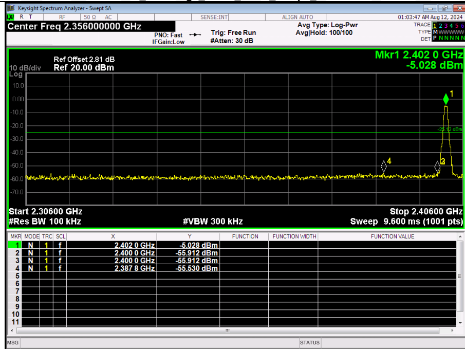
2 Bandedge_NVNT_ANT1_1Mbps_2402
