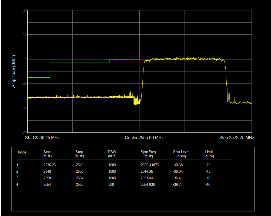
Band41 QAM16 BW=15MHz Channel=40315 RB Size=1 Position=#Max
