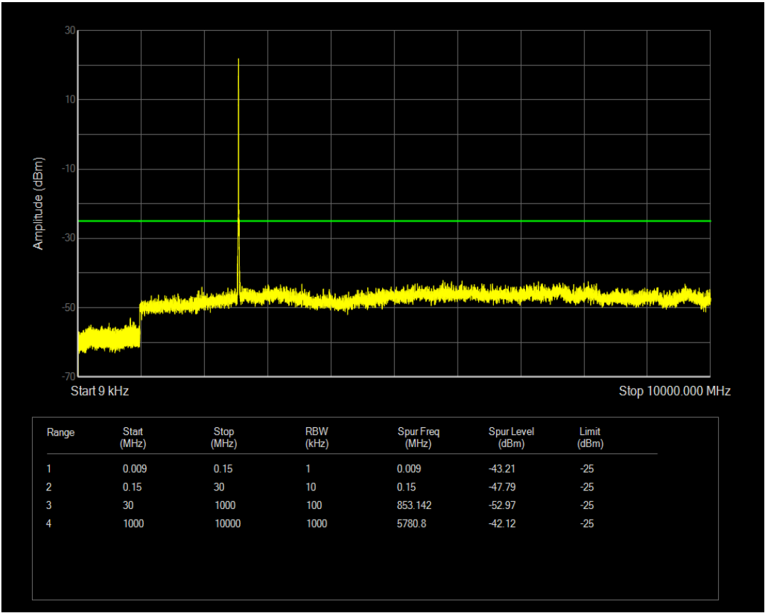
Band41 QAM16 BW=5MHz Channel=40265 RB Size=1 Position=#0
