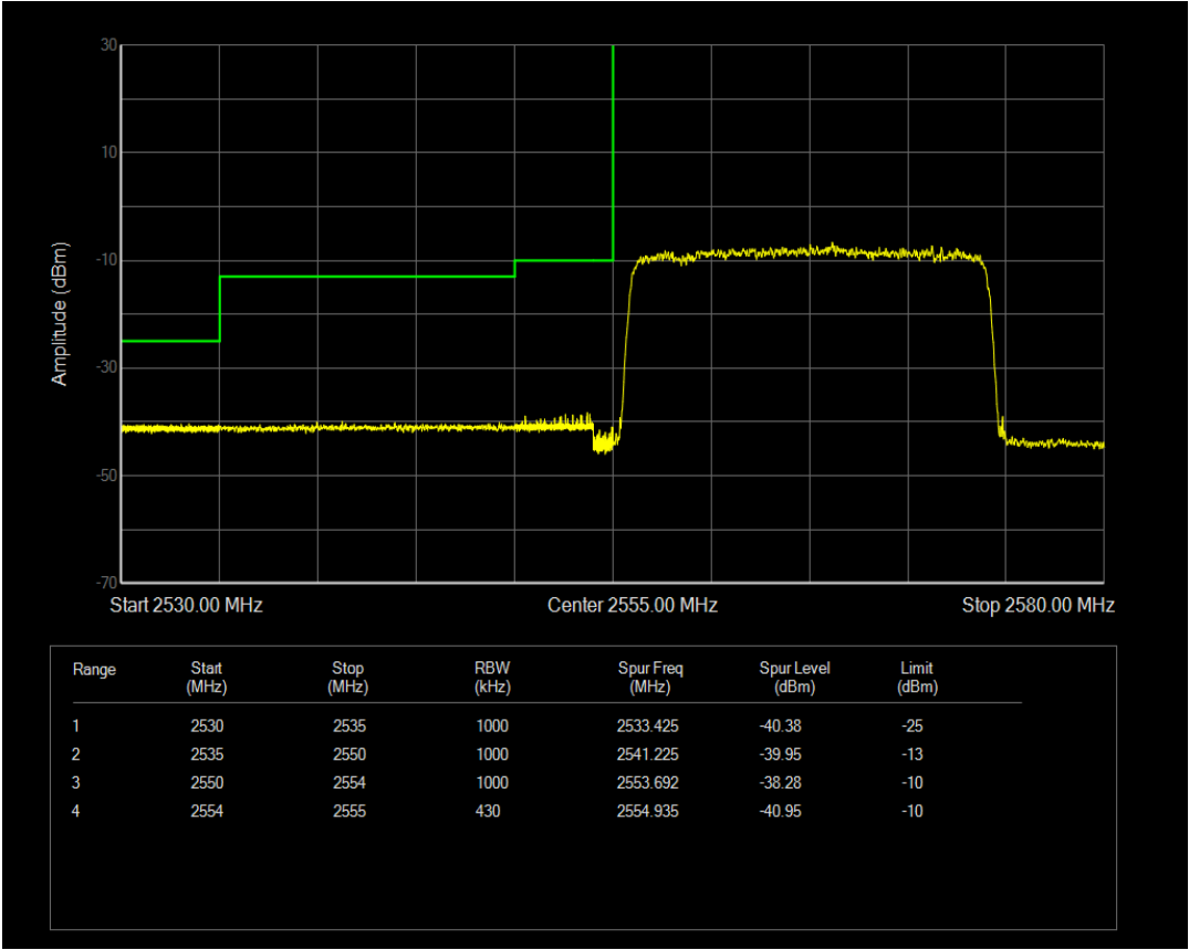
Band41 QAM16 BW=20MHz Channel=40340 RB Size=1 Position=#Max
