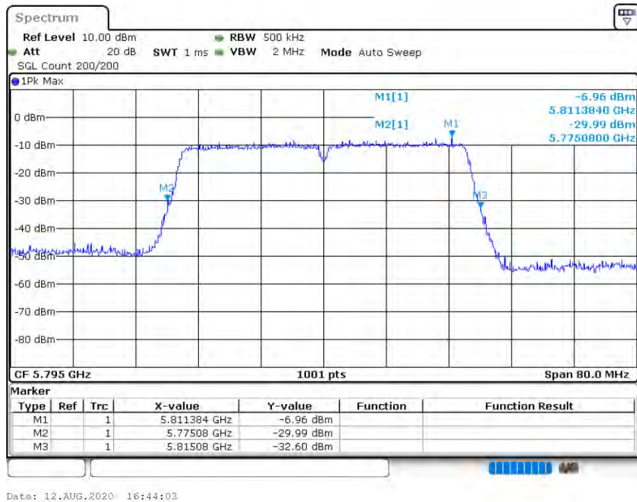
-26 dB BW NVNT 802.11n(HT40) 5795MHz Ant 1
