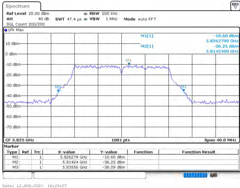
-26 dB BW NVNT 802.11a 5825MHz Ant 1
