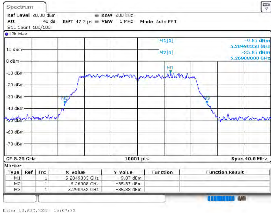
-26 dB BW NVNT 802.11ac20 5280MHz Ant 2
