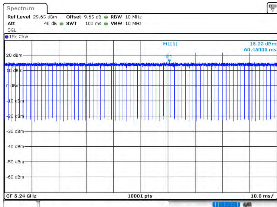
Duty Cycle NVNT 802.11ac20 5240MHz Ant 2
