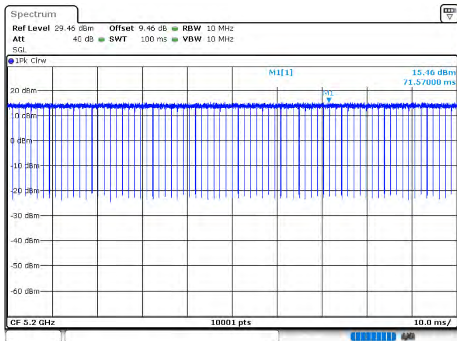
Duty Cycle NVNT 802.11ac20 5200MHz Ant 2
