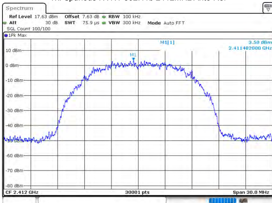
Tx. Spurious NVNT 802.11b 2412MHz Ant3 Ref
