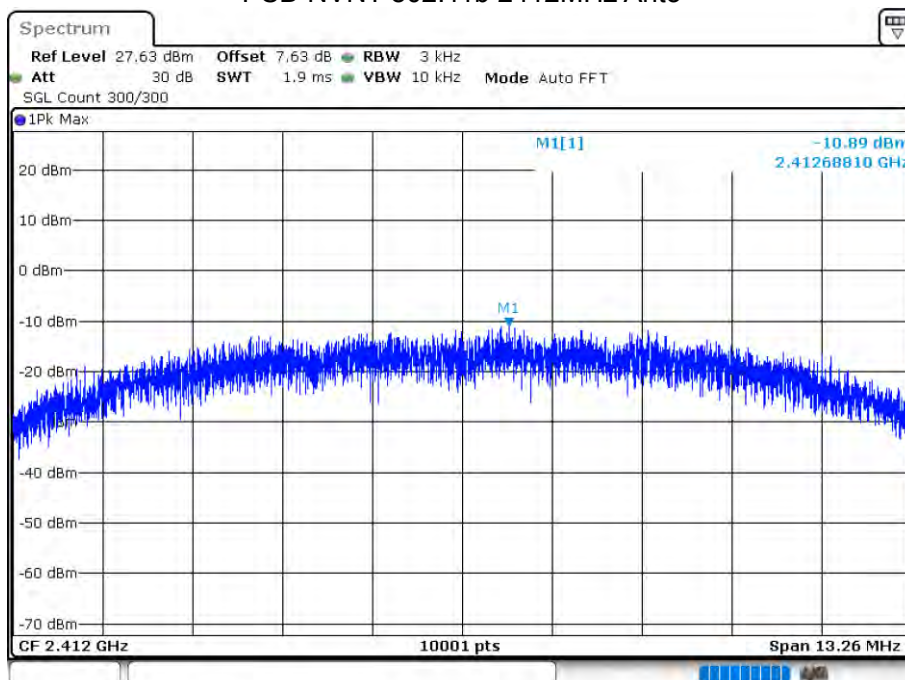
PSD NVNT 802.11b 2412MHz Ant3
