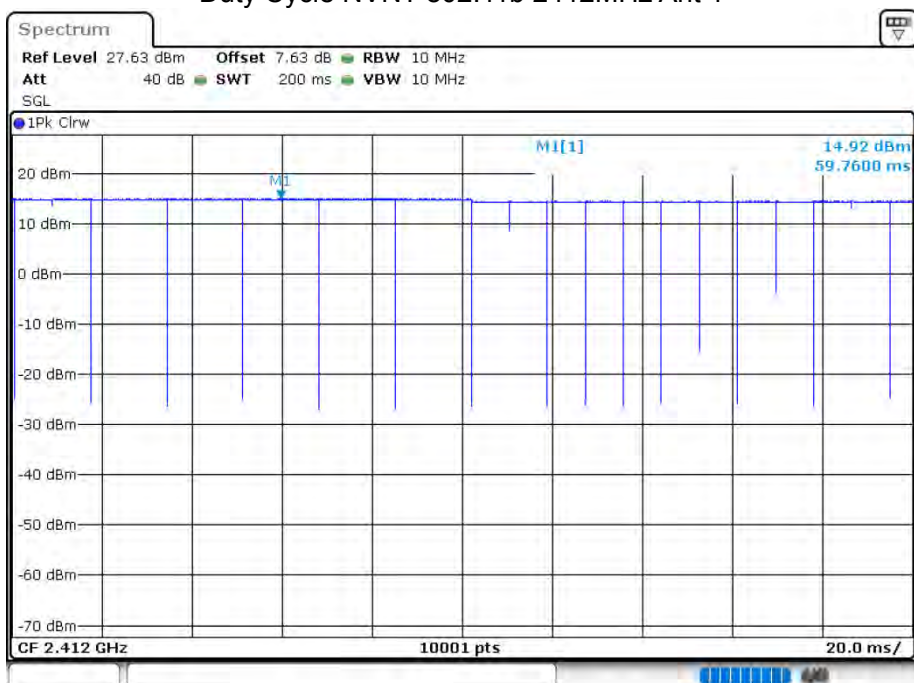
Duty Cycle NVNT 802.11b 2412MHz Ant 1
