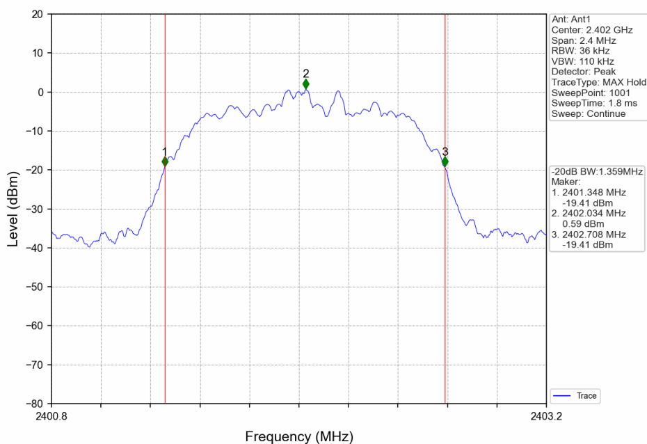
Pi/4DQPSK_2DH5_LCH_2402MHz_Ant1_NTN
