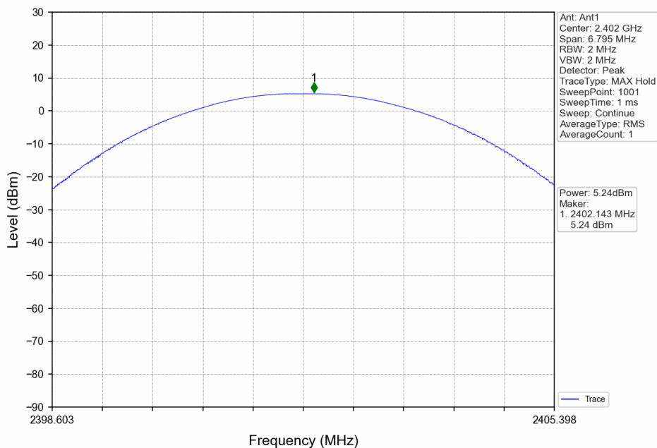
Pi/4DQPSK_2DH5_LCH_2402MHz_Ant1_NTN
