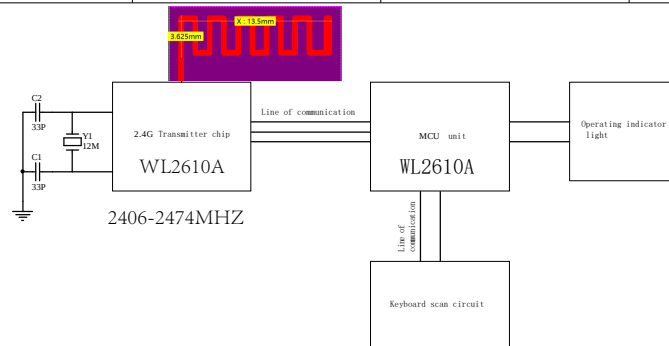
Remote control block diagram
