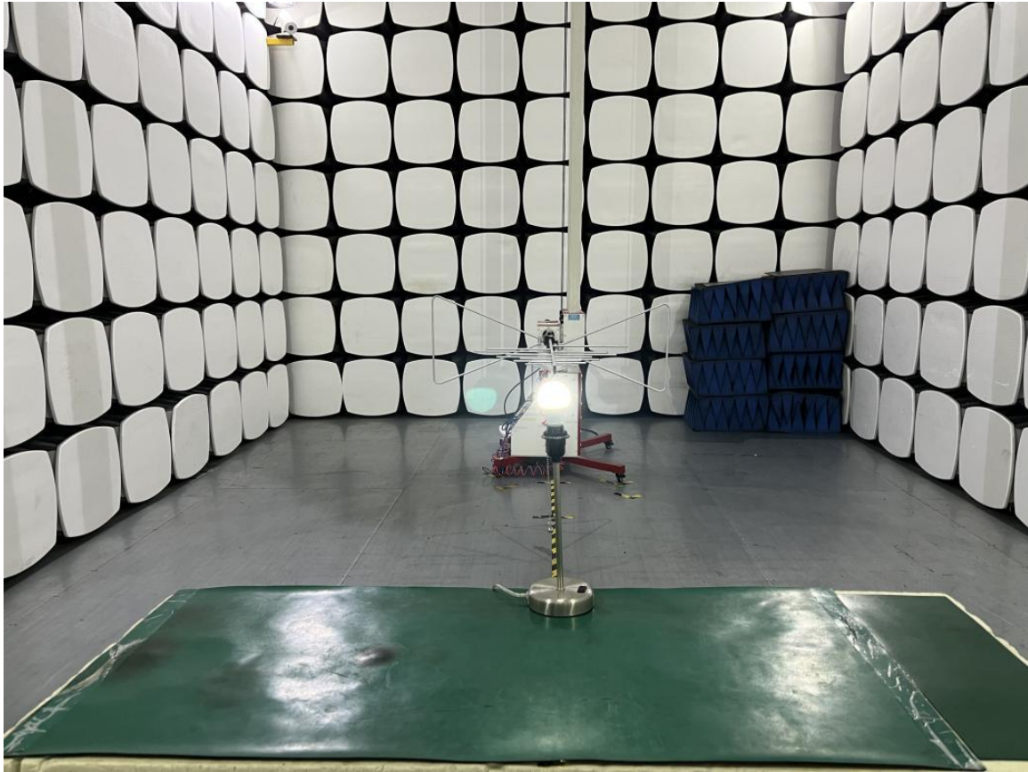
30MHz~1GHz Radiated Emission Test setup
