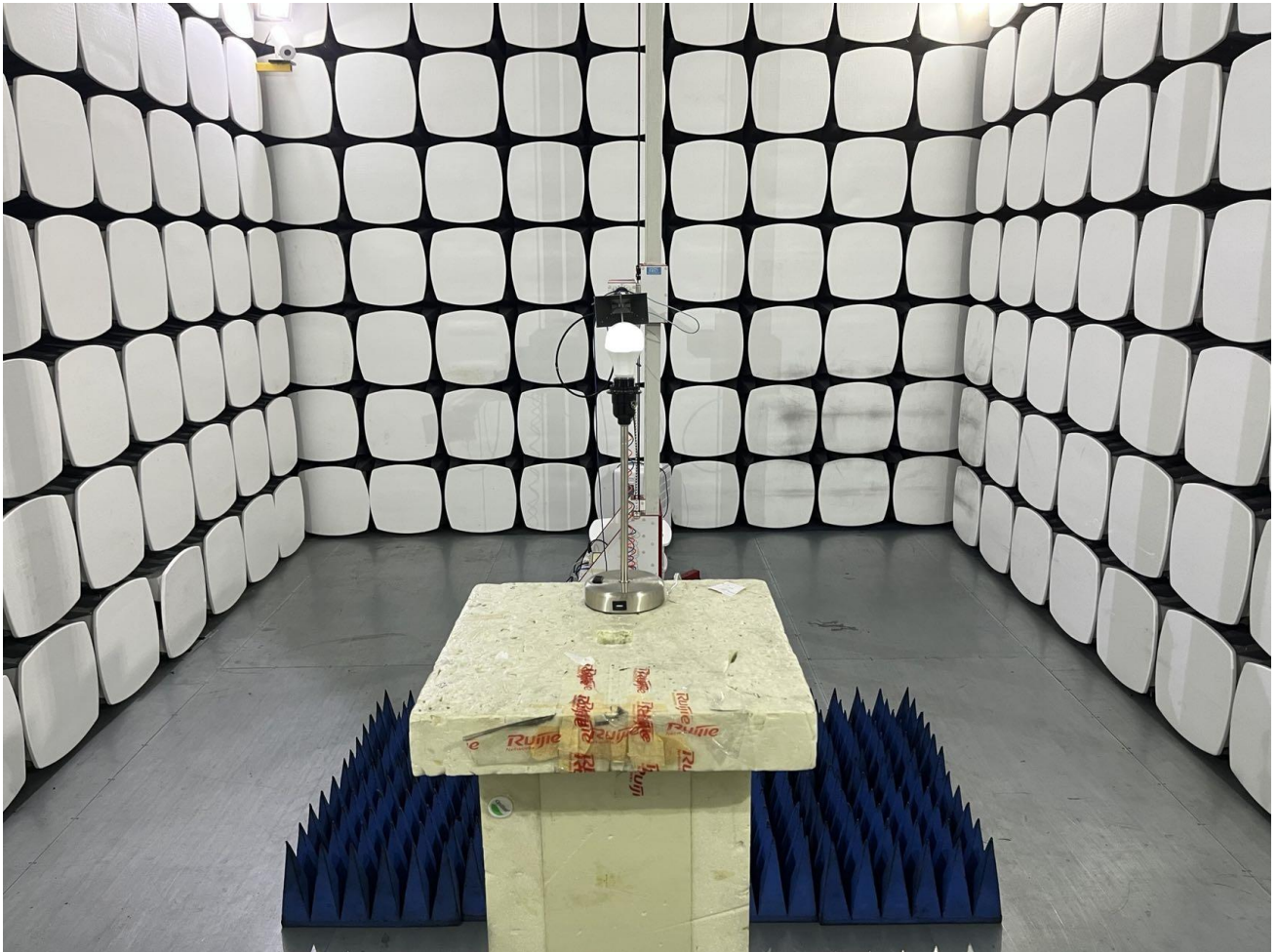
Above 1G Radiated Emission Test setup
