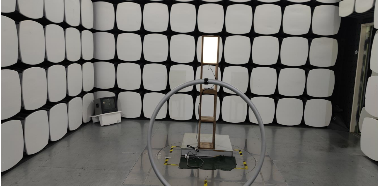
Radiated emission Test Setup (Below 30 MHz)
