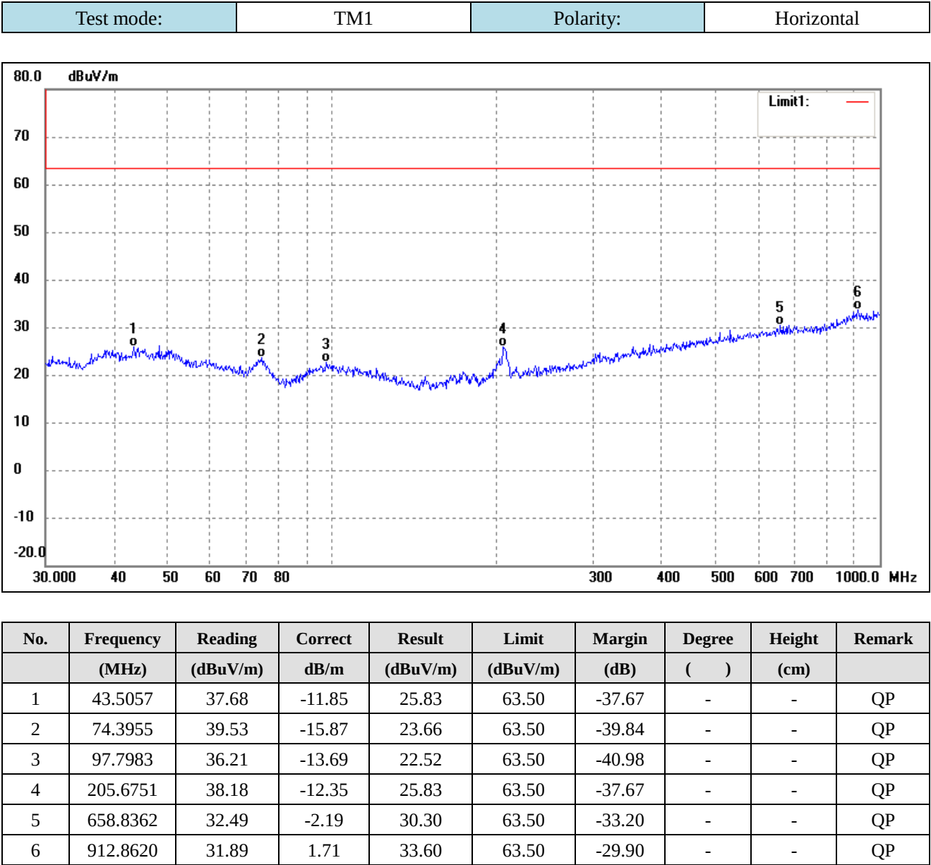
Plot of Radiated Emissions Test Data ( Above 30MHz)
