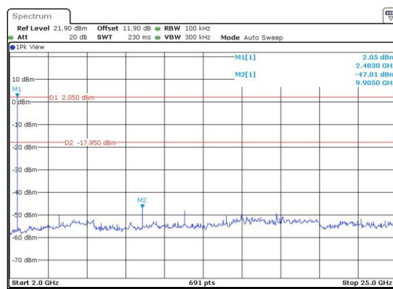
CSE Plot on CH 78 between 2 GHz ~ 25 GHz
