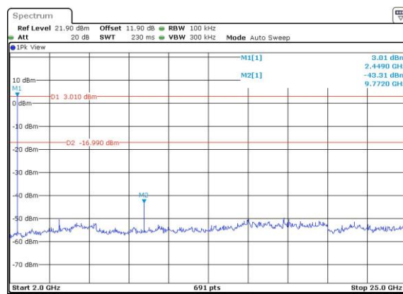
CSE Plot on CH 39 between 2 GHz ~ 25 GHz
