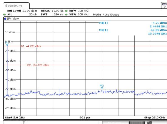
CSE Plot on CH 39 between 2 GHz ~ 25 GHz
