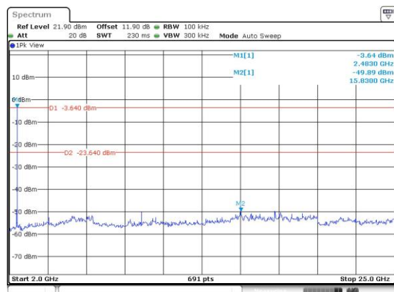
CSE Plot on CH 78 between 2 GHz ~ 25 GHz
