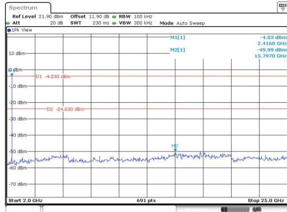
CSE Plot on CH 00 between 2 GHz ~ 25 GHz
