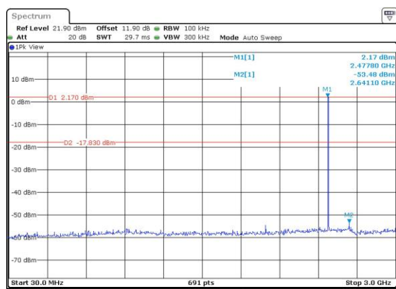
CSE Plot on CH 78 between 30 MHz ~ 3 GHz
