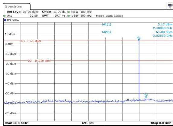
CSE Plot on CH 00 between 30 MHz ~ 3 GHz
