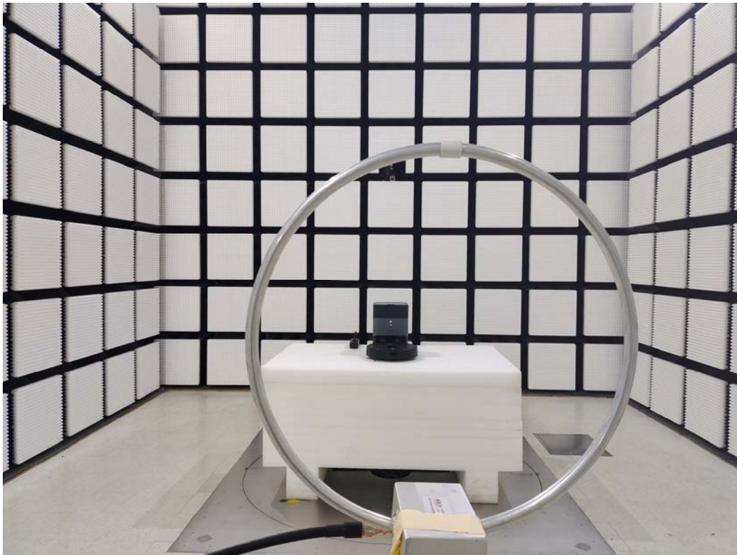
Radiated Emission Below 30MHz Parallel View
