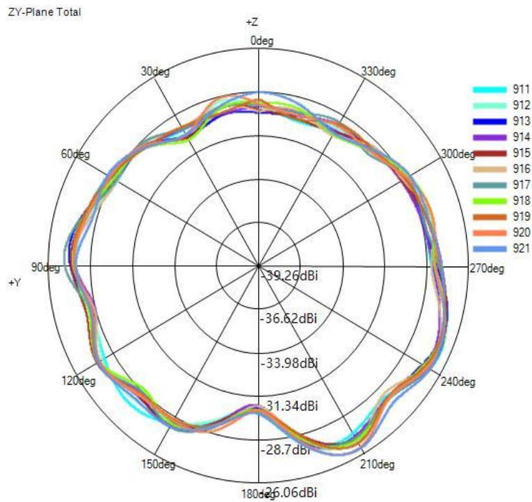
(2) Y-Z Plane(unit:dBi):
