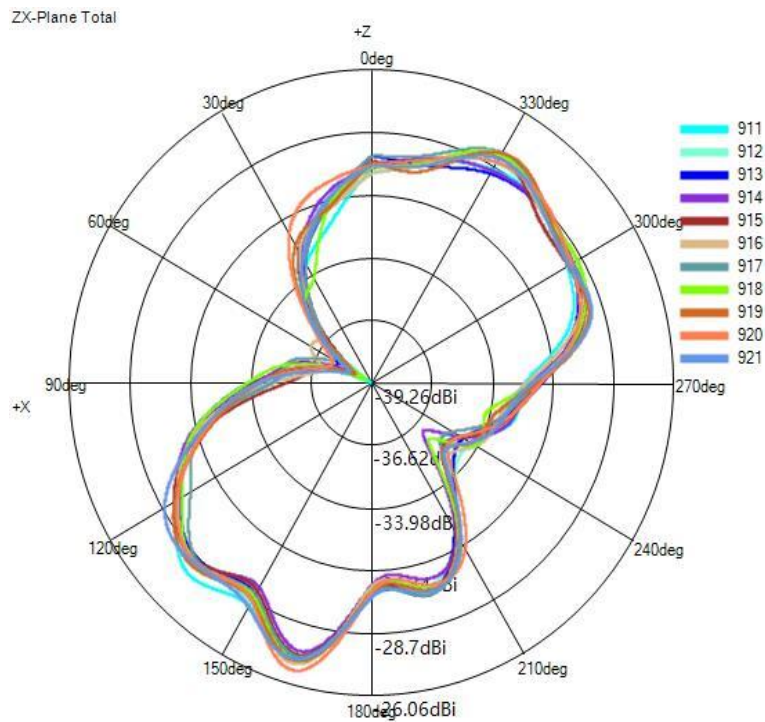
(1) X-Z Plane(unit:dBi):
