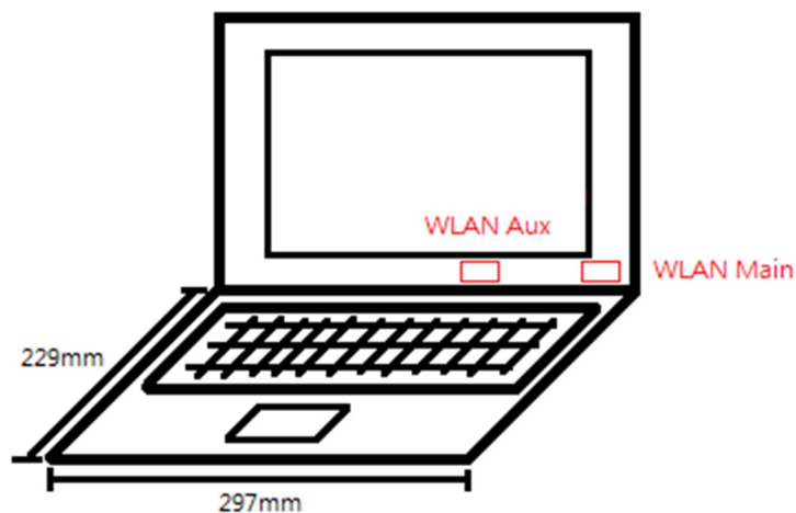
Photograph 5. Antenna position of EUT
