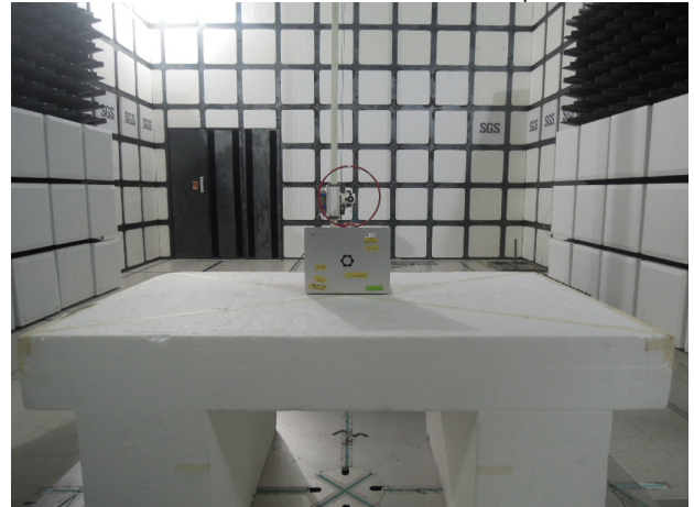
FCC_15_247_WLAN_Radiated_Setup
