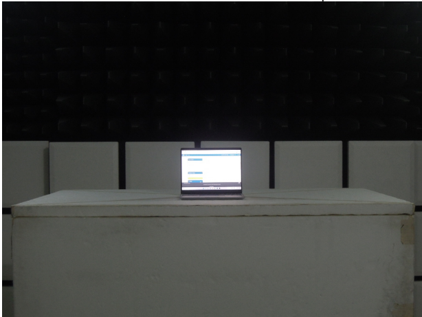
FCC_15_247_WLAN_Radiated_Setup
