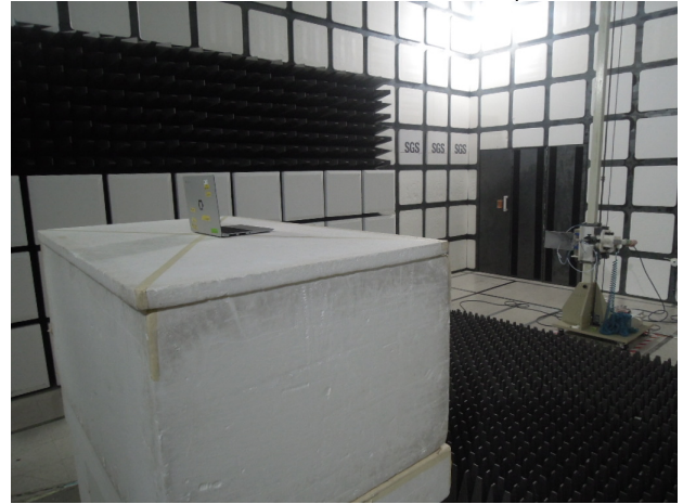
FCC_15_247_WLAN_Radiated_Setup
