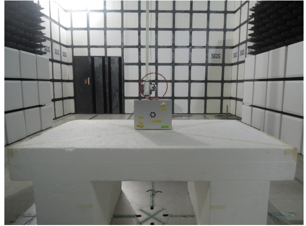
FCC_15_247_BT_Radiated_Setup
