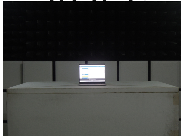
FCC_15_407_WLAN_6E_Radiated_Setup
