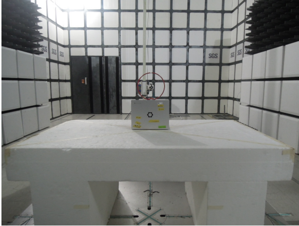
FCC_15_247_WLAN_Radiated_Setup
