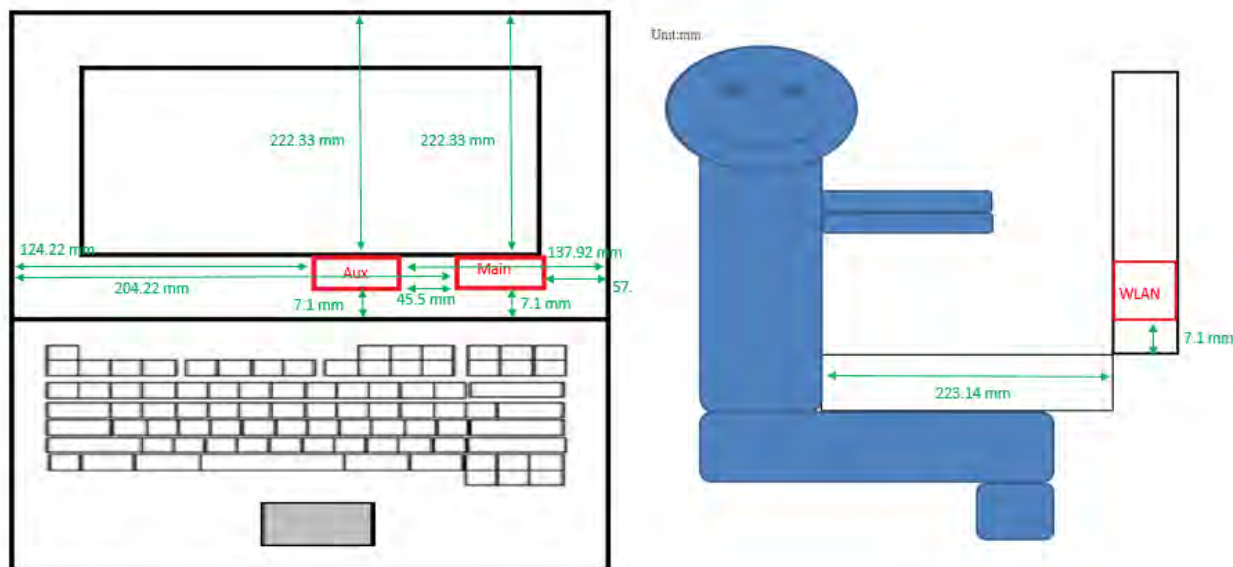
Photograph 13. Antenna position of EUT
