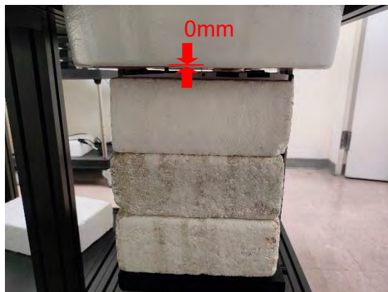
Photograph 2. Body, Bottom Surface, 0mm_#1
