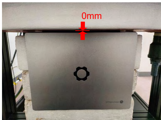
Photograph 1. Body, Bottom Surface, 0mm_#1
