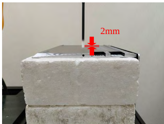
Photograph 8. PD, Bottom Surface, 2mm_#2
