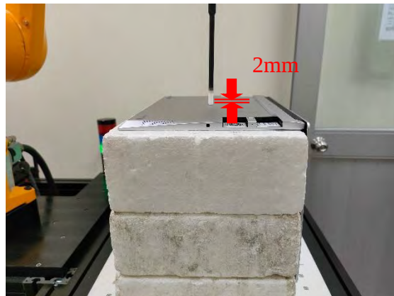
Photograph 6. PD, Bottom Surface, 2mm_#1
