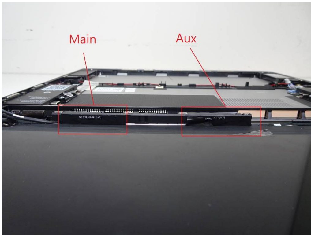
Antenna_BT/WLAN
