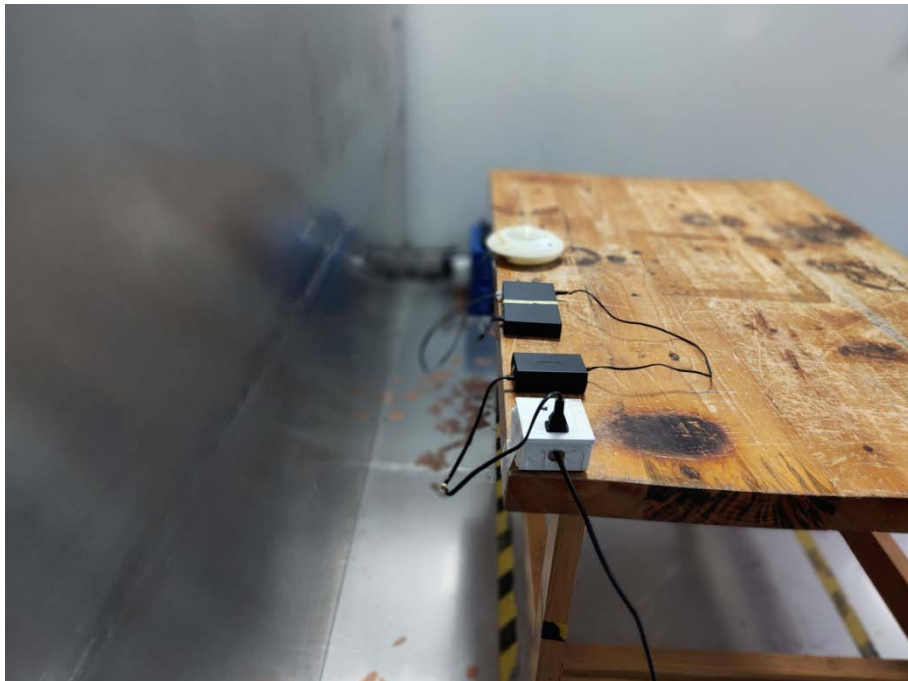
Conducted Emissions –POE- Side View
