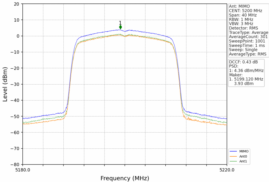
802.11ax(HEW20)_MCH_5200MHz_RU242_Left_MIMO_NTNV
