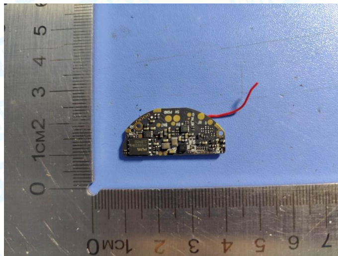
Photo 8 Appearance of PCB
