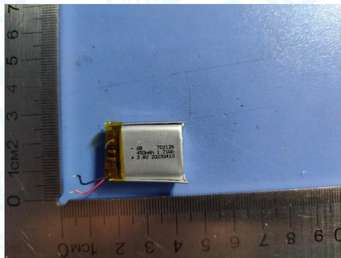
Photo 10 Battery appearance
