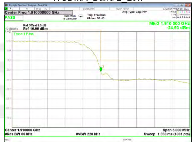
WCDMA_Band 2_High
