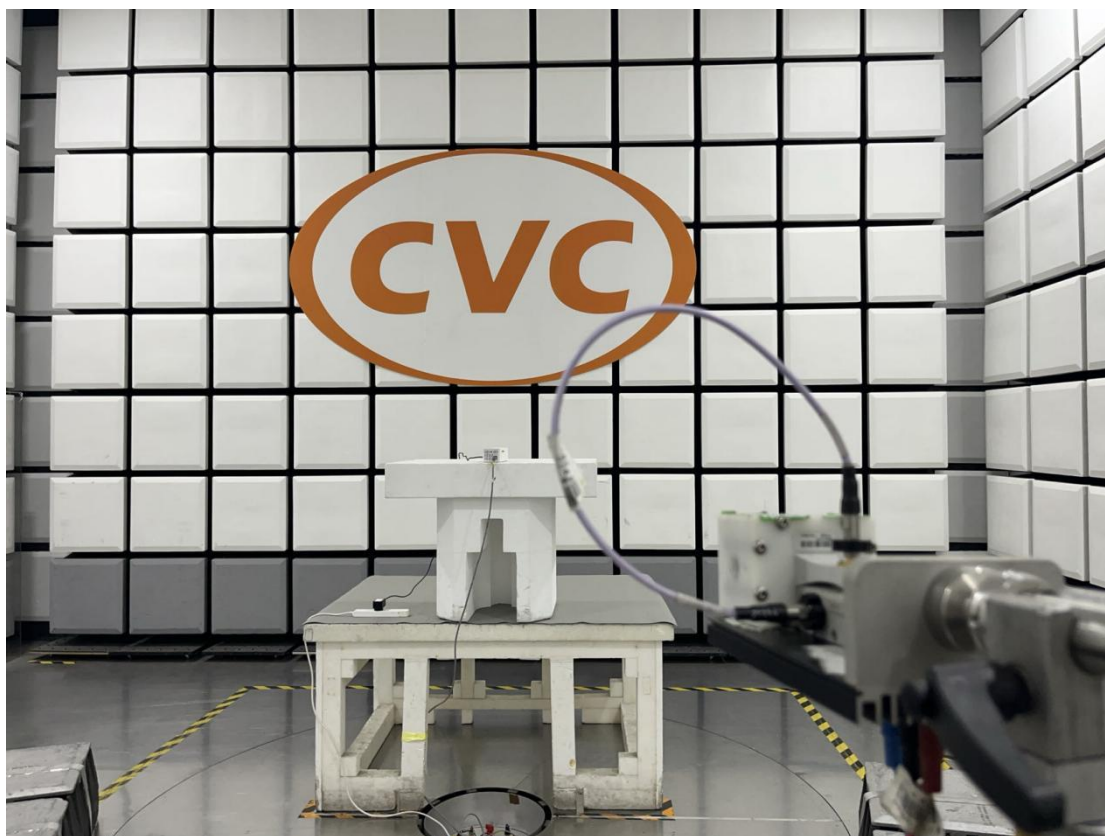
Radiated Test Setup(frequency range:18GHz-40GHz)
