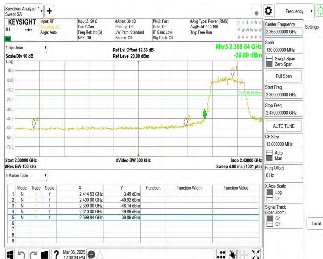
11N20SISO_Ant1_Low_2412
