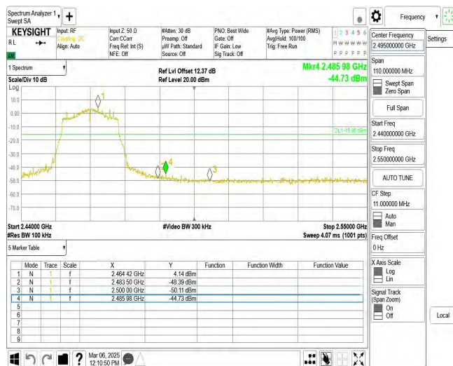
11N20SISO_Ant1_High_2462
