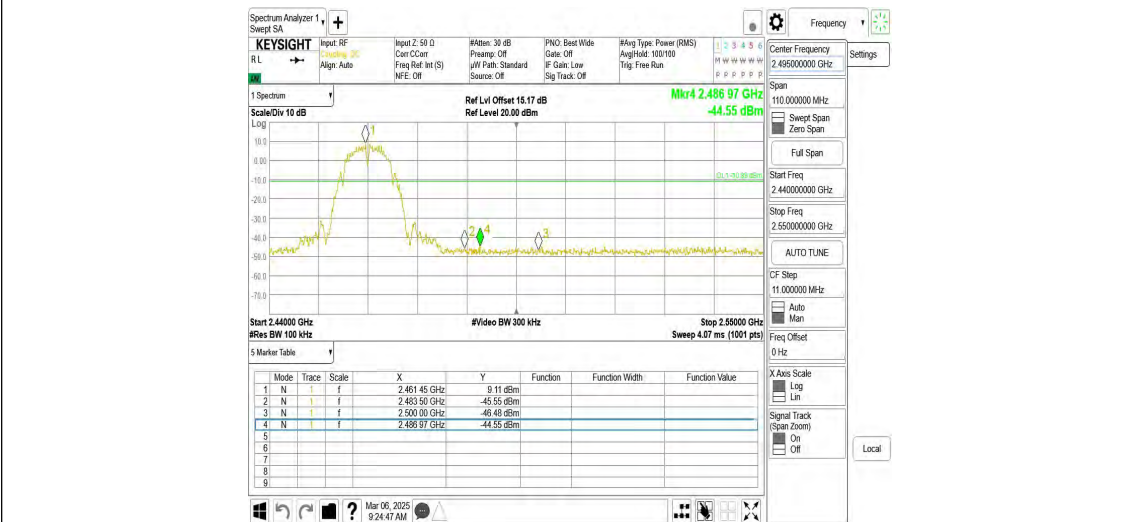
11B_Ant1_High_2462
