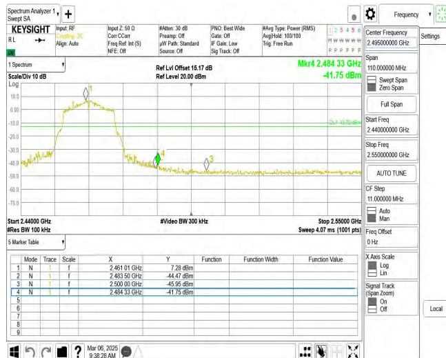
11G_Ant1_High_2462
