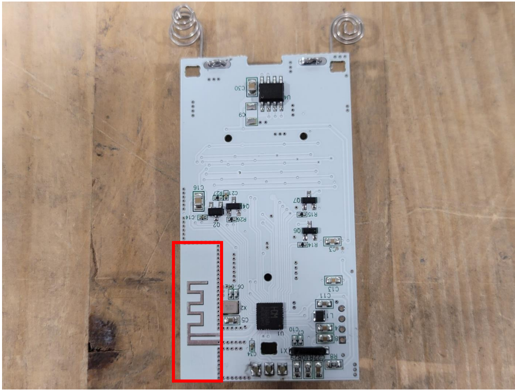
2402-2480MHz Antenna
