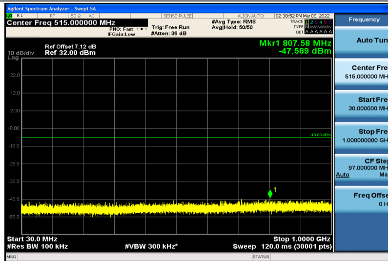
Band2-20MHz-64QAM-18700-1RB#0-30~1000MHz
