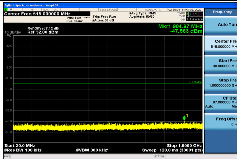
Band4-3MHz-64QAM-19965-1RB#0-30~1000MHz
