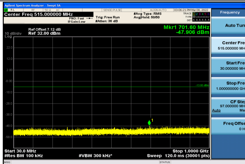
Band4-5MHz-64QAM-20175-1RB#0-30~1000MHz
