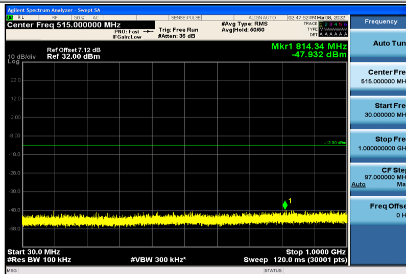
Band4-1.4MHz-64QAM-20393-1RB#0-30~1000MHz
