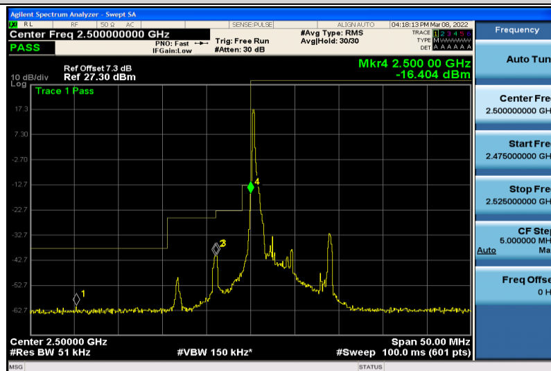
Band7-5MHz-64QAM-20775-1RB#0
