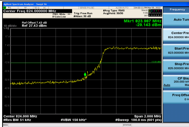
Band5-5MHz-64QAM-20425-25RB#0
