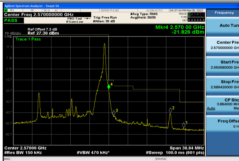
Band7-15MHz-64QAM-21375-1RB#74
