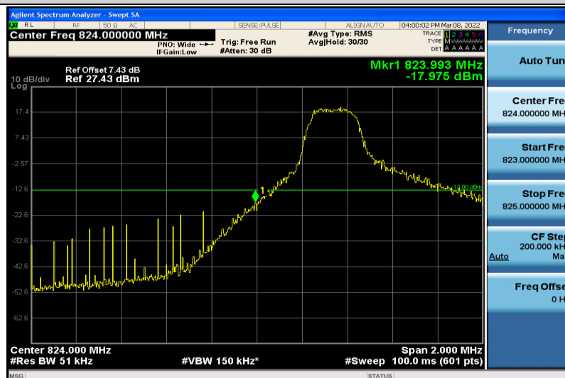
Band5-5MHz-64QAM-20425-1RB#0
