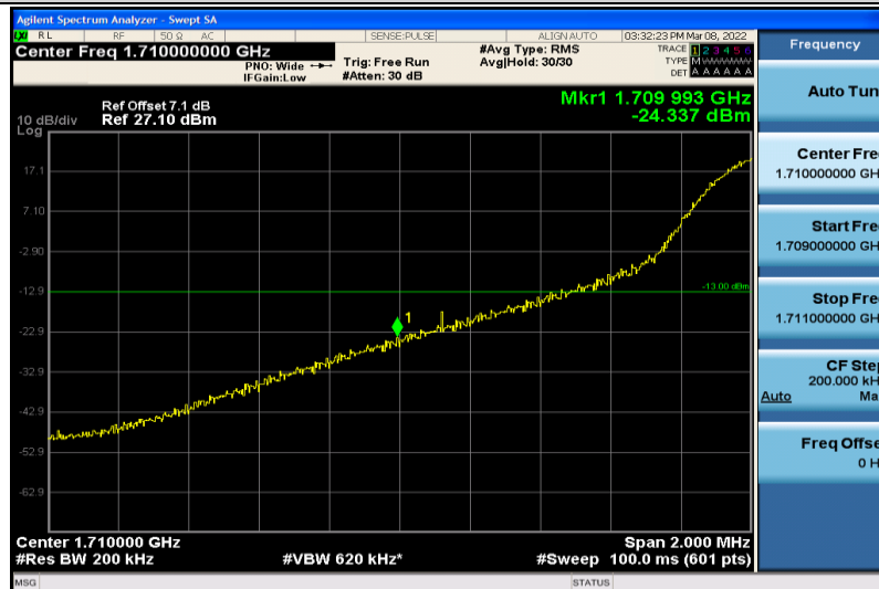
Band4-20MHz-64QAM-20050-1RB#0
