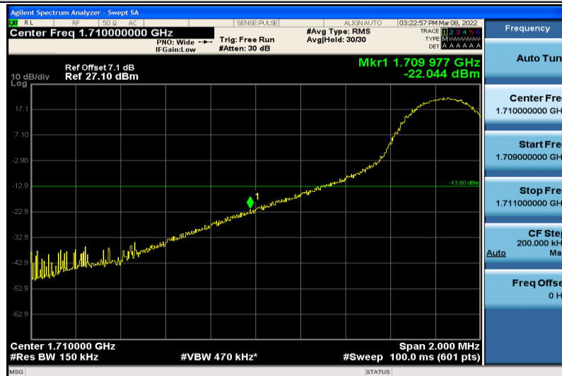
Band4-15MHz-64QAM-20025-1RB#0
