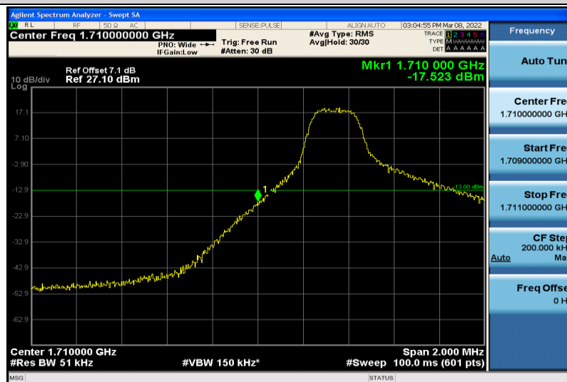
Band4-5MHz-64QAM-19975-1RB#0
