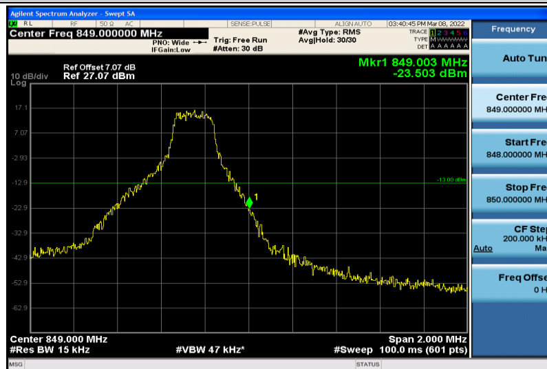
Band5-1.4MHz-64QAM-20643-1RB#5
