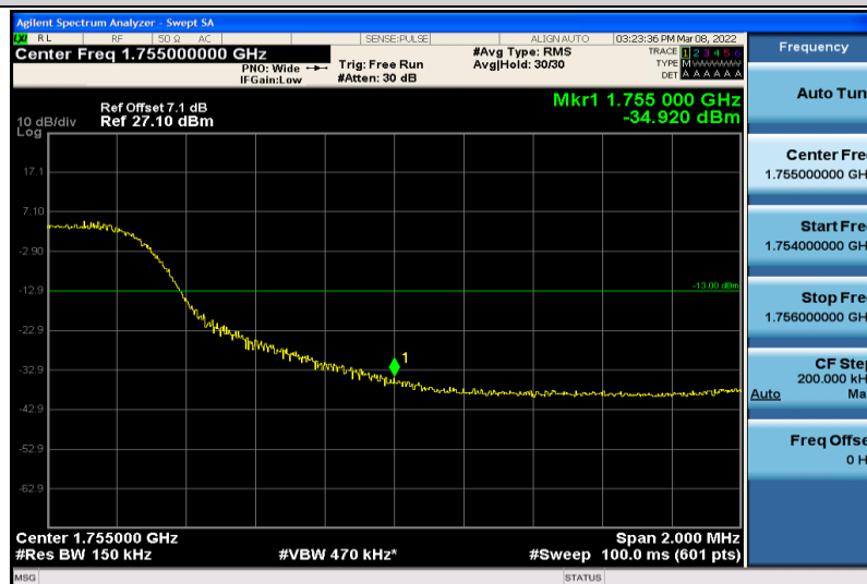
Band4-15MHz-64QAM-20325-75RB#0
