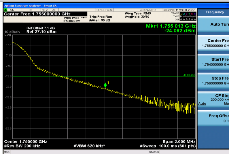
Band4-20MHz-64QAM-20300-1RB#99
