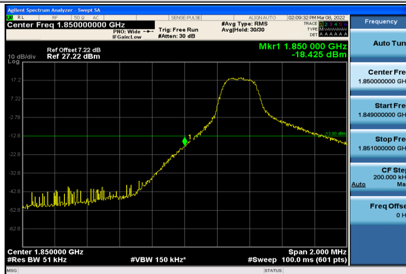
Band2-5MHz-64QAM-18625-1RB#0
