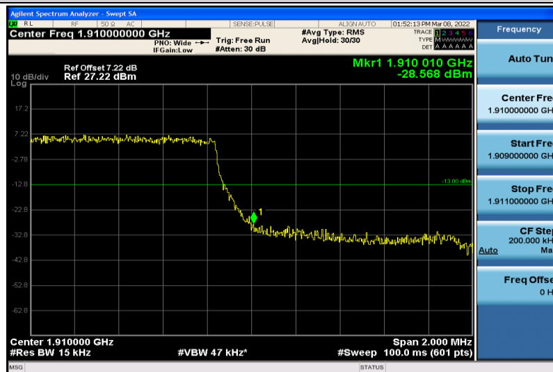
Band2-1.4MHz-64QAM-19193-6RB#0
