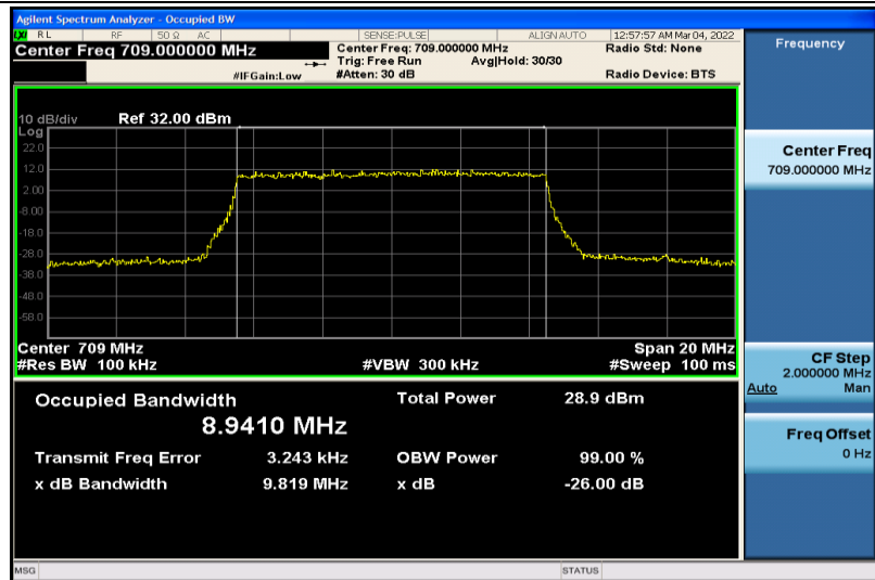
Band17-10MHz-16QAM-23780-50RB#0-8.9410
