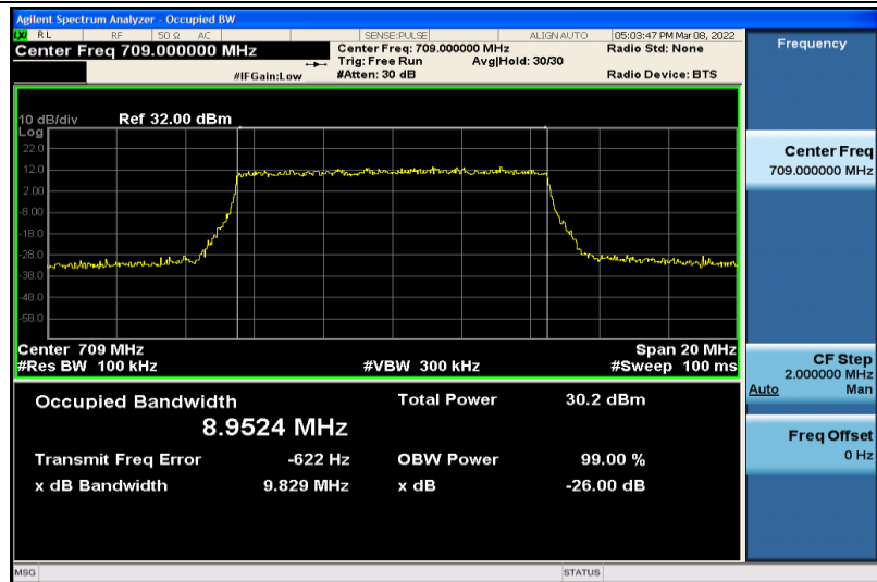
Band17-10MHz-64QAM-23780-50RB#0-8.9524
