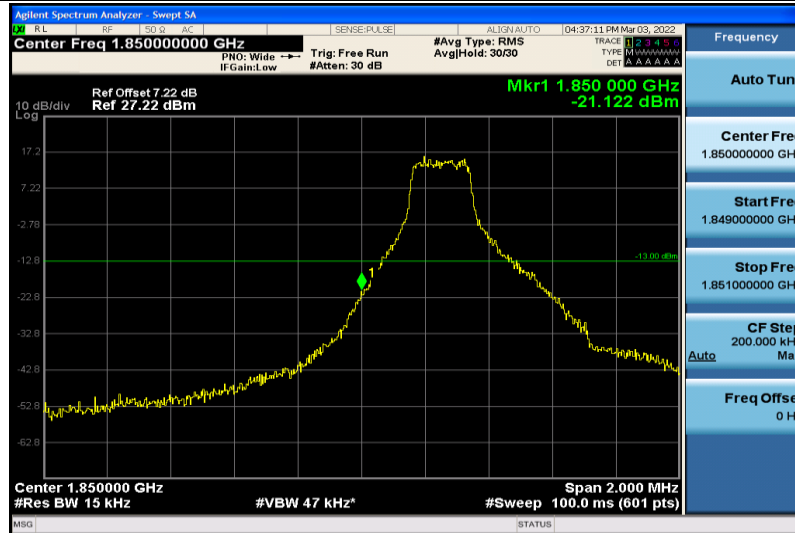
Band2-1.4MHz-QPSK-18607-1RB#0
