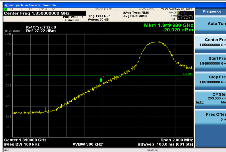
Band2-10MHz-16QAM-18650-1RB#0
