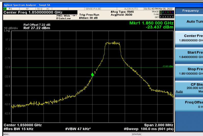
Band2-1.4MHz-64QAM-18607-1RB#0
