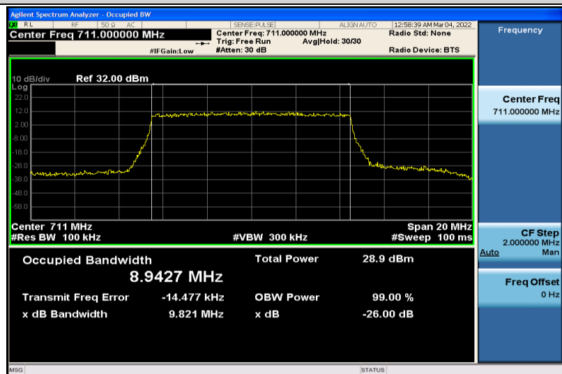
Band17-10MHz-16QAM-23800-50RB#0-8.9427
