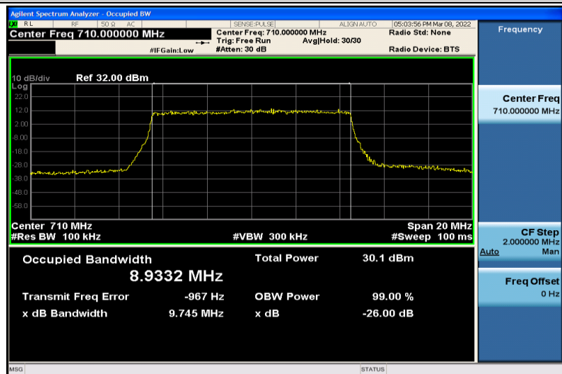
Band17-10MHz-64QAM-23790-50RB#0-8.9332
