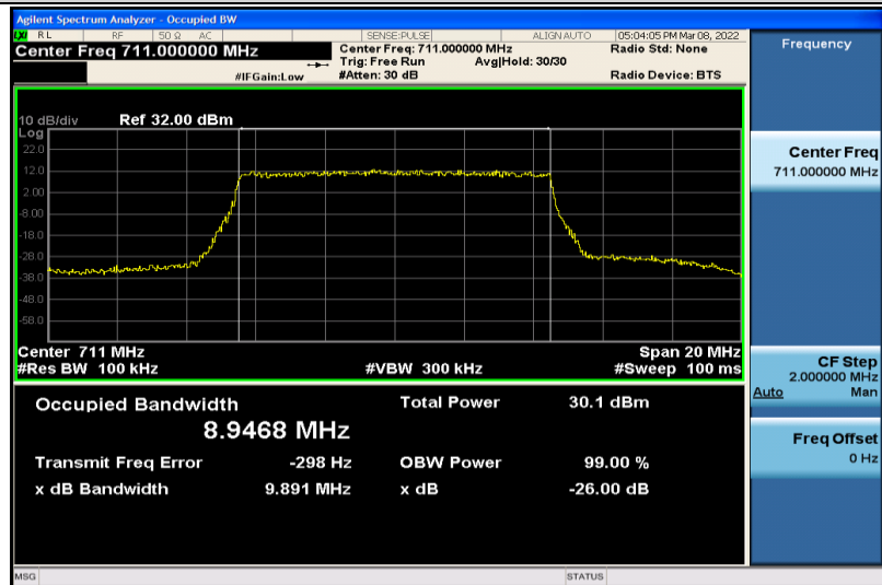
Band17-10MHz-64QAM-23800-50RB#0-8.9468
