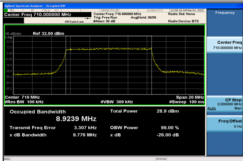
Band17-10MHz-16QAM-23790-50RB#0-8.9239
