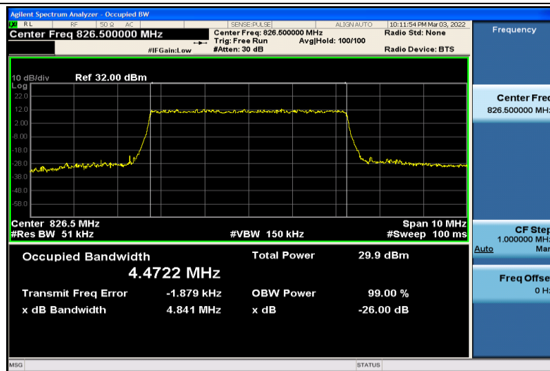
Band5-5MHz-QPSK-20425-25RB#0-4.4722
