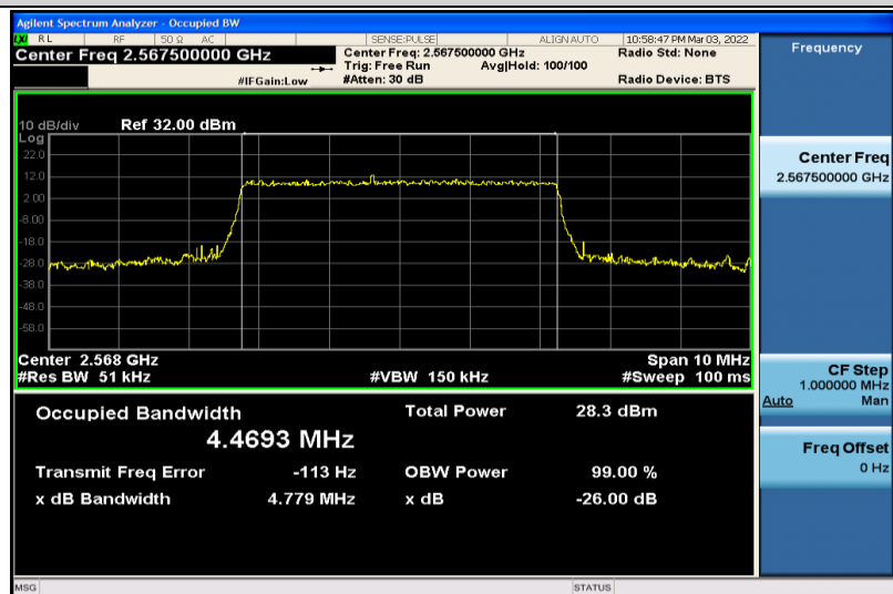
Band7-5MHz-16QAM-21425-25RB#0-4.4693
