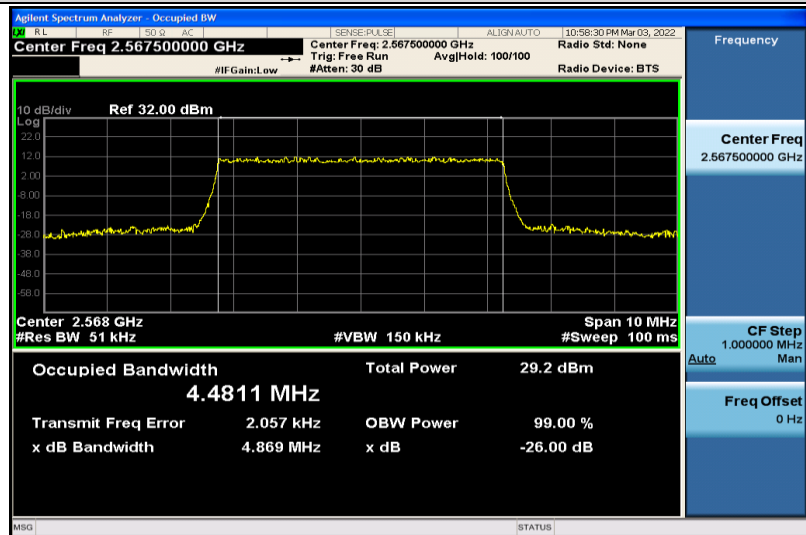
Band7-5MHz-QPSK-21425-25RB#0-4.4811
