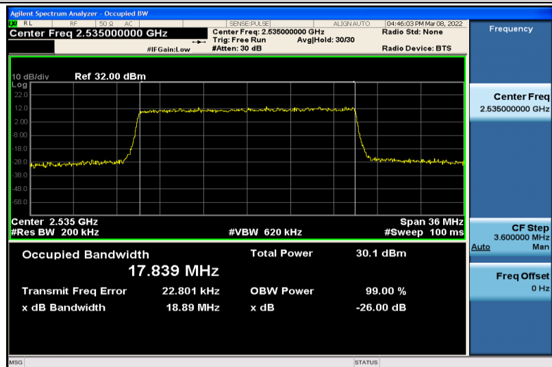
Band7-20MHz-64QAM-21100-100RB#0-17.839
