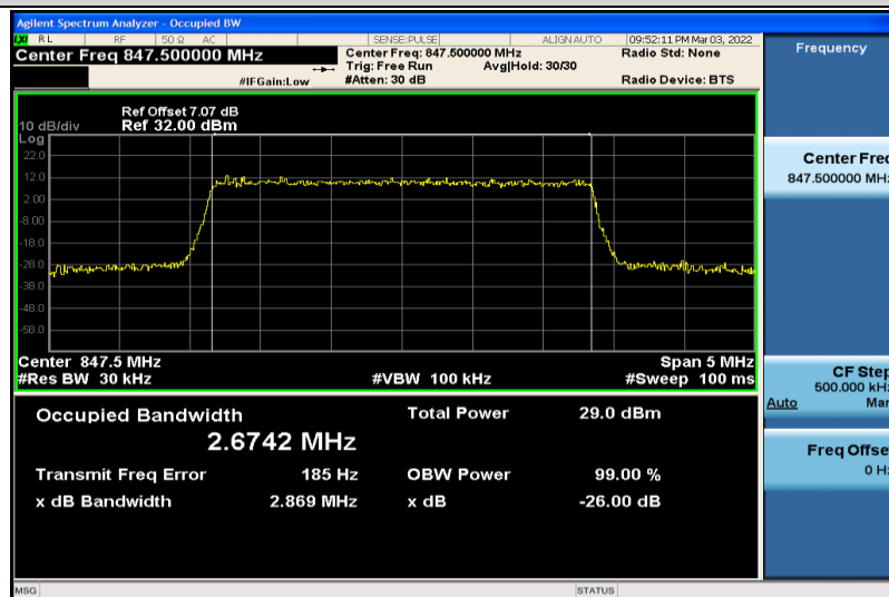
Band5-3MHz-QPSK-20635-15RB#0-2.6742
