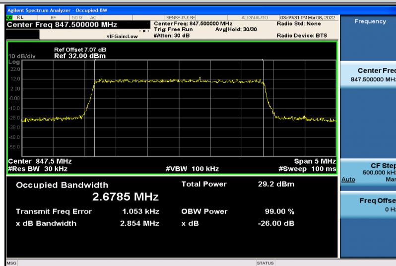
Band5-3MHz-64QAM-20635-15RB#0-2.6785
