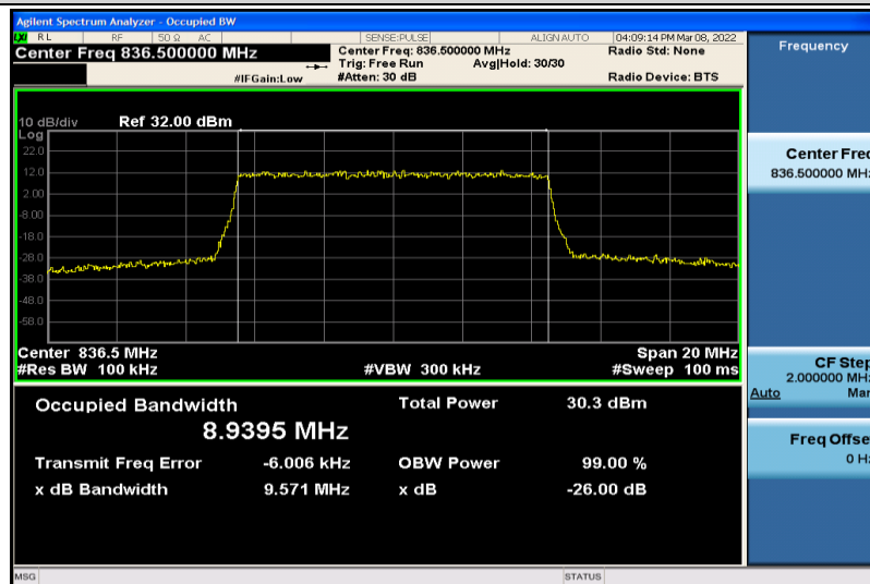
Band5-10MHz-64QAM-20525-50RB#0-8.9395
