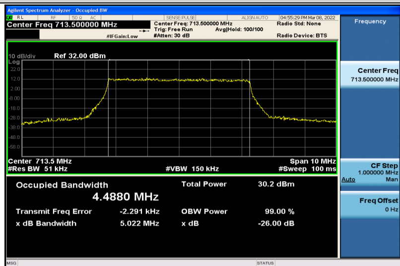
Band17-5MHz-64QAM-23825-25RB#0-4.4880
