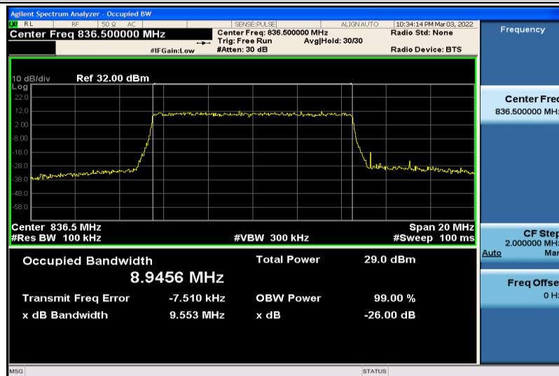
Band5-10MHz-16QAM-20525-50RB#0-8.9456
