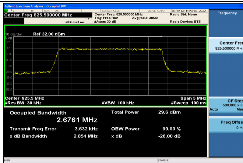
Band5-3MHz-64QAM-20415-15RB#0-2.6761
