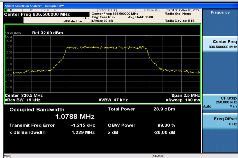
Band5-1.4MHz-QPSK-20525-6RB#0-1.0788
