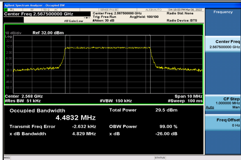
Band7-5MHz-64QAM-21425-25RB#0-4.4832
