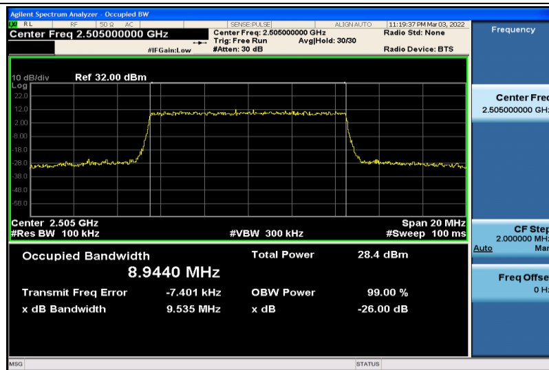
Band7-10MHz-16QAM-20800-50RB#0-8.9440
