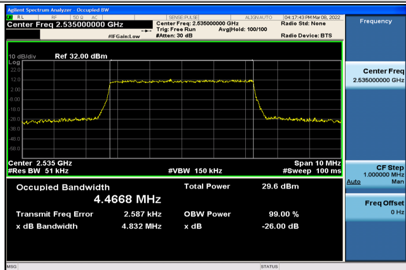
Band7-5MHz-64QAM-21100-25RB#0-4.4668
