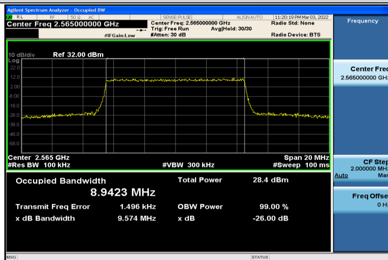
Band7-10MHz-16QAM-21400-50RB#0-8.9423
