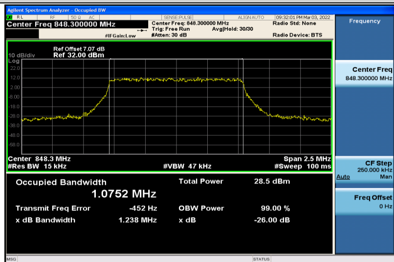
Band5-1.4MHz-QPSK-20643-6RB#0-1.0752
