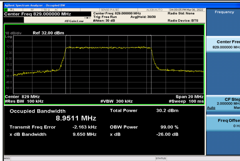
Band5-10MHz-64QAM-20450-50RB#0-8.9511
