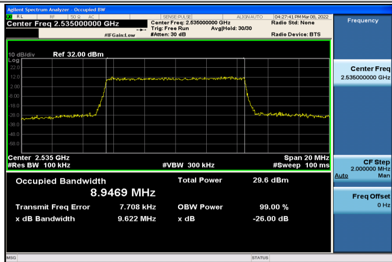
Band7-10MHz-64QAM-21100-50RB#0-8.9469
