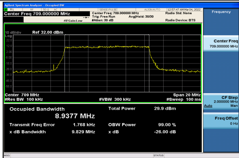
Band17-10MHz-QPSK-23780-50RB#0-8.9377
