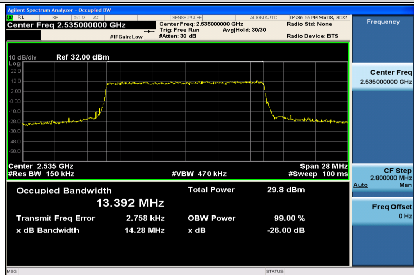
Band7-15MHz-64QAM-21100-75RB#0-13.392
