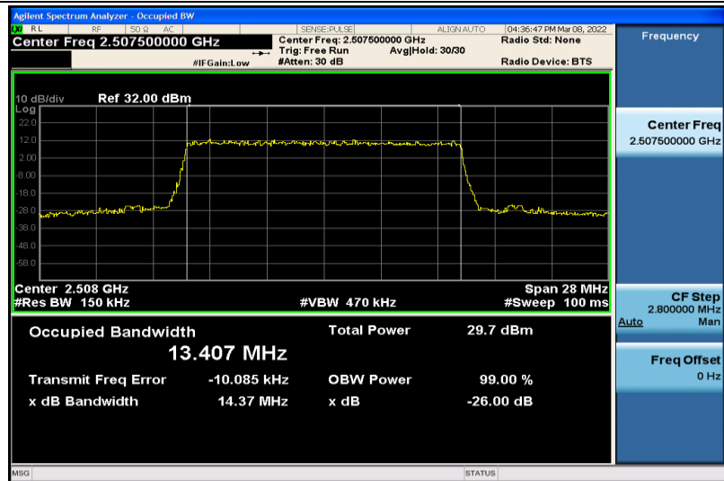
Band7-15MHz-64QAM-20825-75RB#0-13.407
