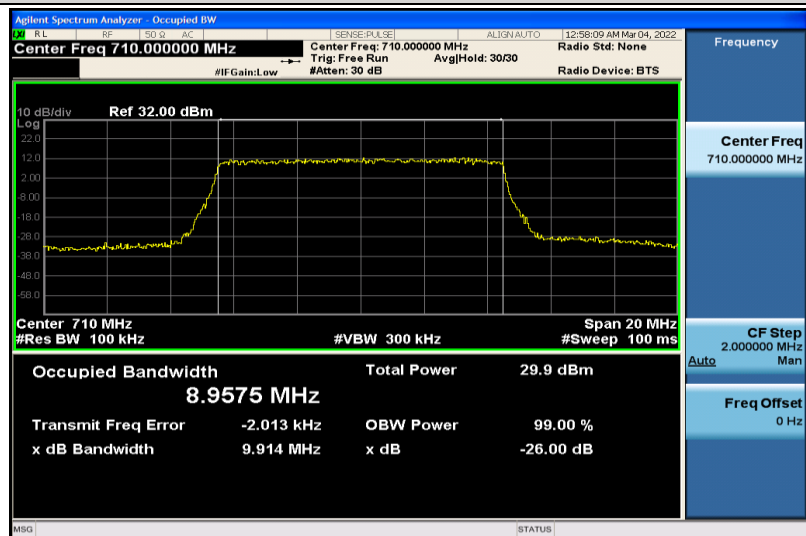
Band17-10MHz-QPSK-23790-50RB#0-8.9575
