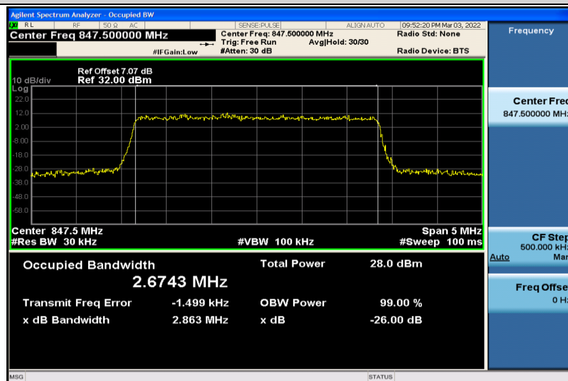
Band5-3MHz-16QAM-20635-15RB#0-2.6743
