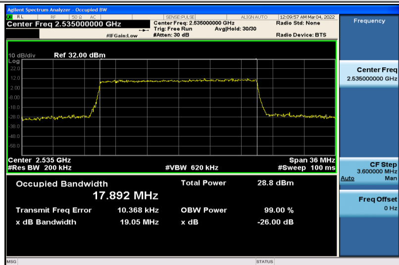
Band7-20MHz-16QAM-21100-100RB#0-17.892
