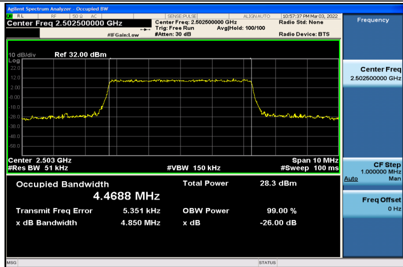
Band7-5MHz-16QAM-20775-25RB#0-4.4688
