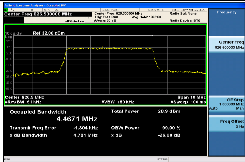
Band5-5MHz-16QAM-20425-25RB#0-4.4671
