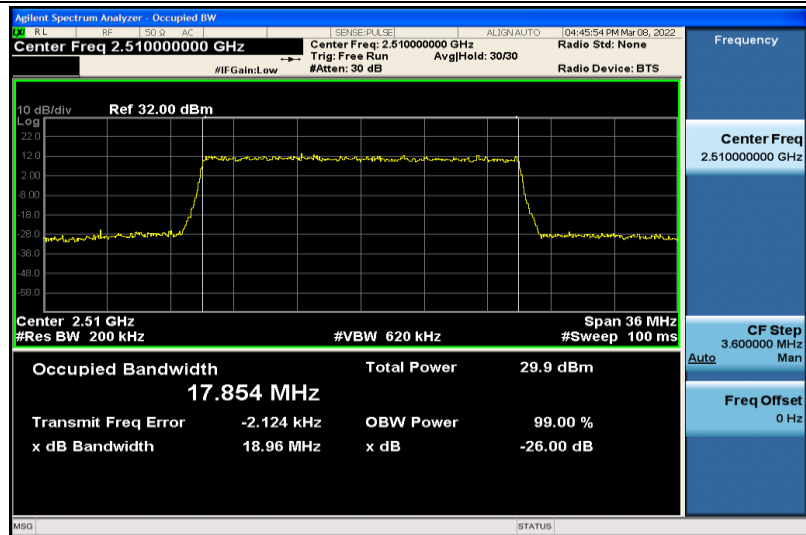
Band7-20MHz-64QAM-20850-100RB#0-17.854
