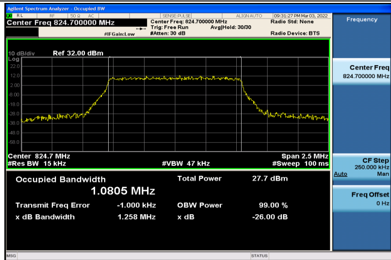
Band5-1.4MHz-16QAM-20407-6RB#0-1.0805
