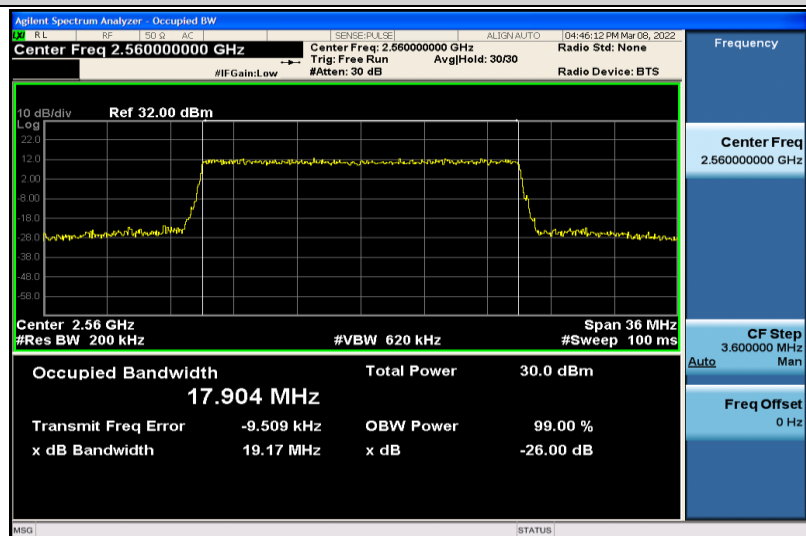
Band7-20MHz-64QAM-21350-100RB#0-17.904
