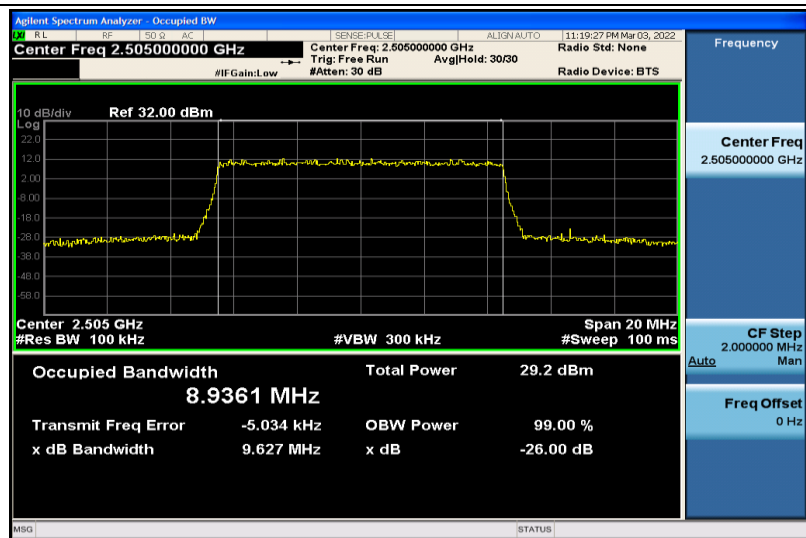
Band7-10MHz-QPSK-20800-50RB#0-8.9361
