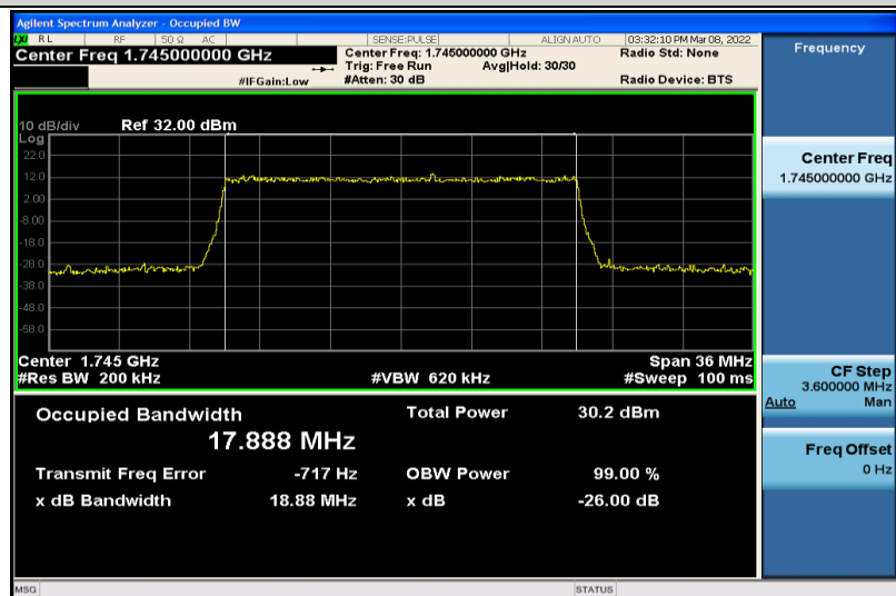
Band4-20MHz-64QAM-20300-100RB#0-17.888
