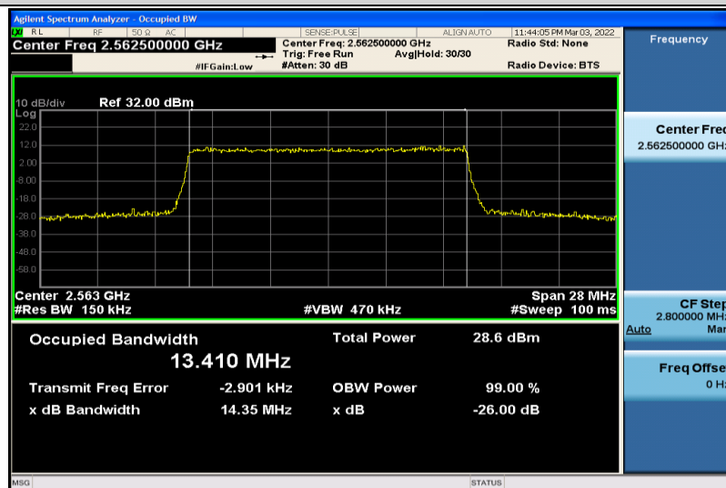
Band7-15MHz-16QAM-21375-75RB#0-13.410
