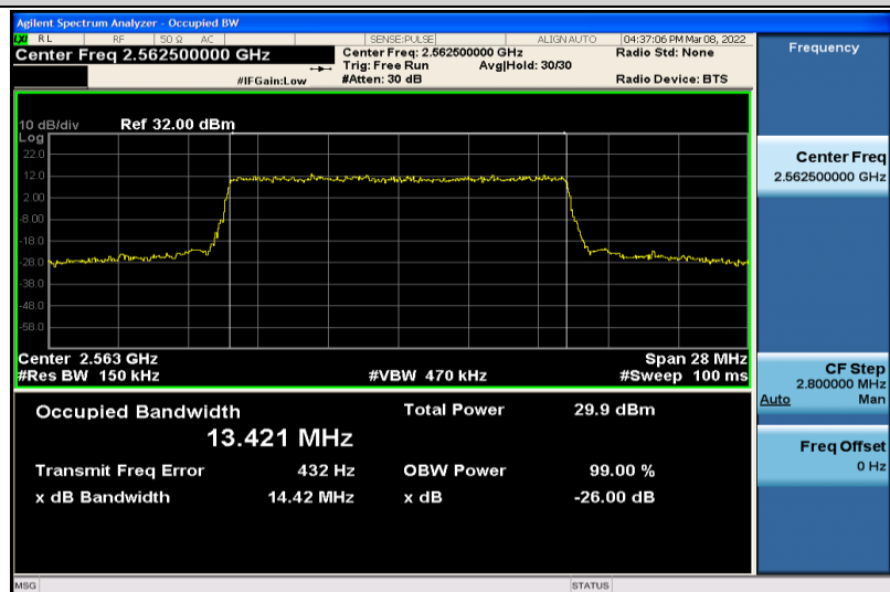
Band7-15MHz-64QAM-21375-75RB#0-13.421
