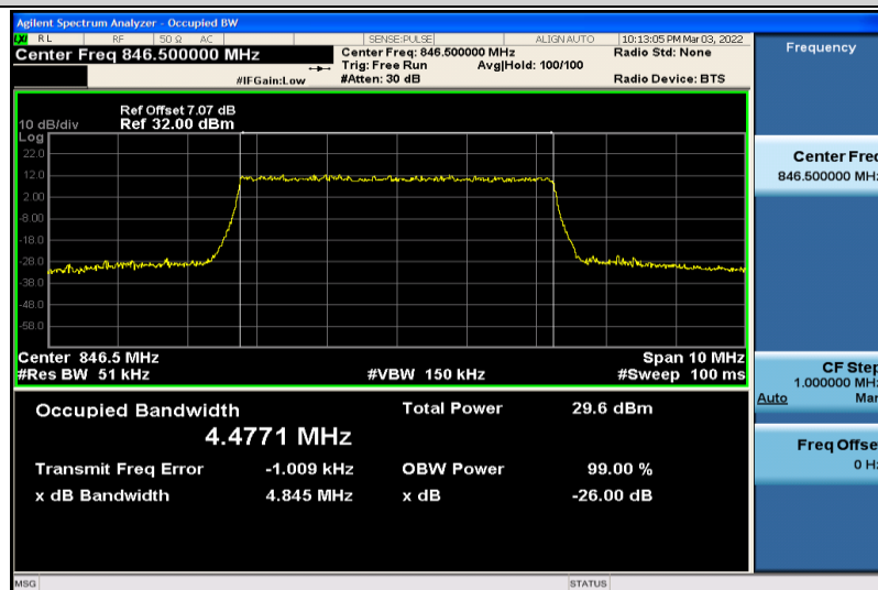
Band5-5MHz-QPSK-20625-25RB#0-4.4771
