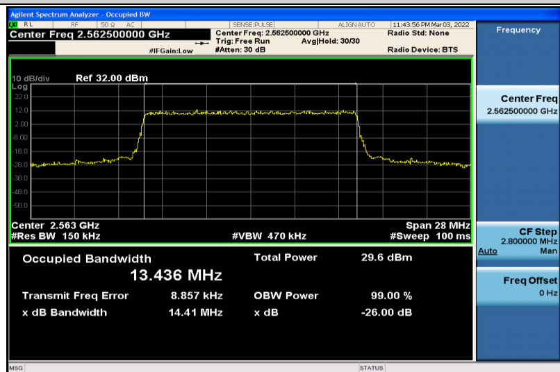
Band7-15MHz-QPSK-21375-75RB#0-13.436
