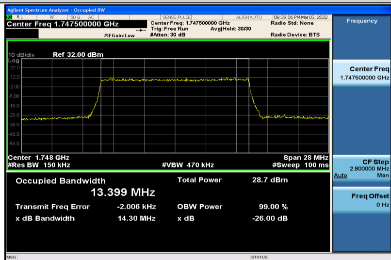
Band4-15MHz-16QAM-20325-75RB#0-13.399
