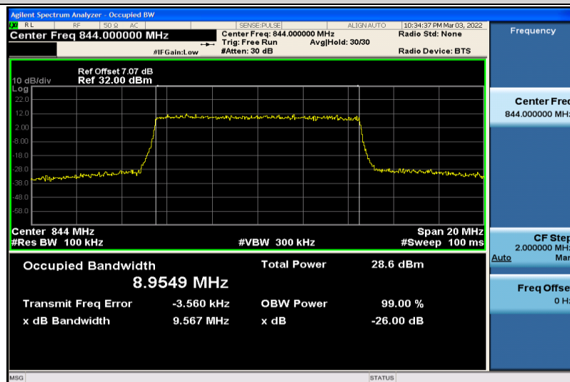
Band5-10MHz-16QAM-20600-50RB#0-8.9549
