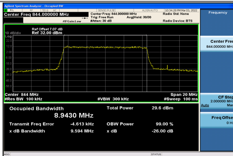
Band5-10MHz-QPSK-20600-50RB#0-8.9430
