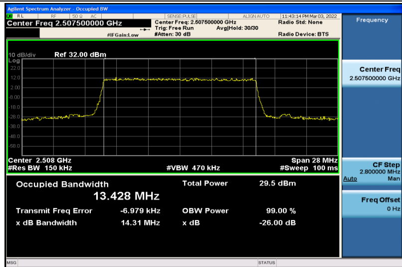
Band7-15MHz-QPSK-20825-75RB#0-13.428
