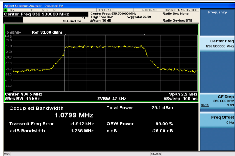
Band5-1.4MHz-64QAM-20525-6RB#0-1.0799
