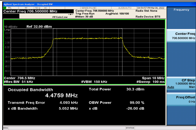
Band17-5MHz-64QAM-23755-25RB#0-4.4759
