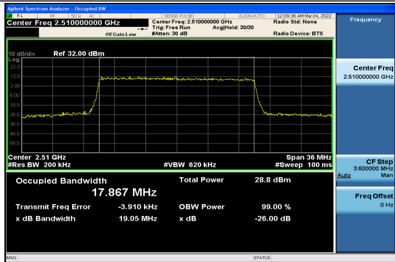
Band7-20MHz-16QAM-20850-100RB#0-17.867
