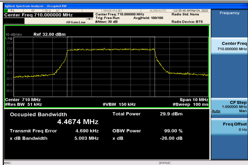
Band17-5MHz-QPSK-23790-25RB#0-4.4674
