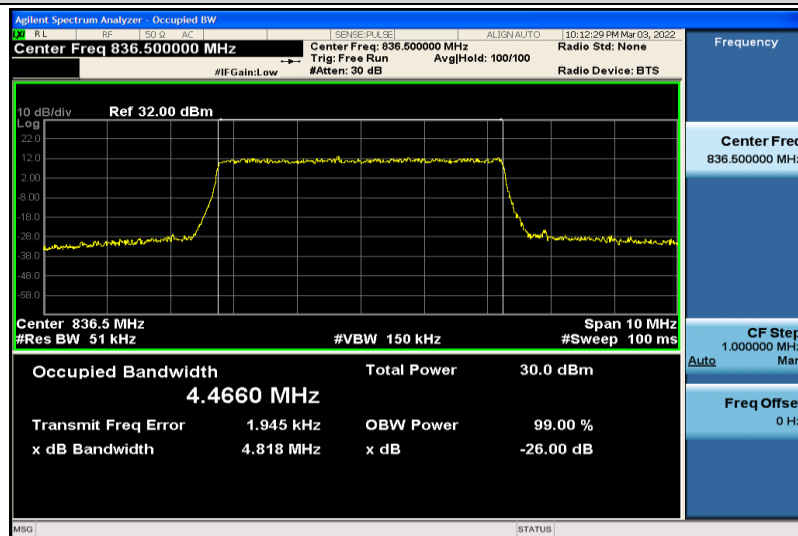
Band5-5MHz-QPSK-20525-25RB#0-4.4660
