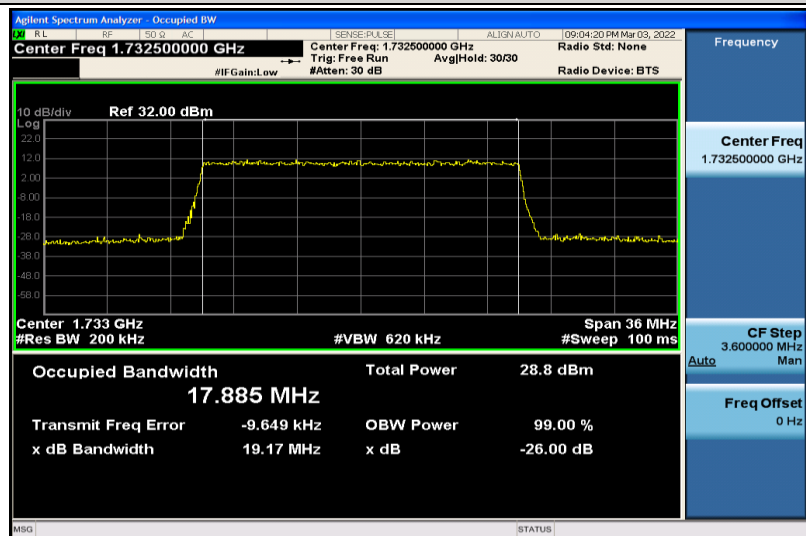
Band4-20MHz-16QAM-20175-100RB#0-17.885
