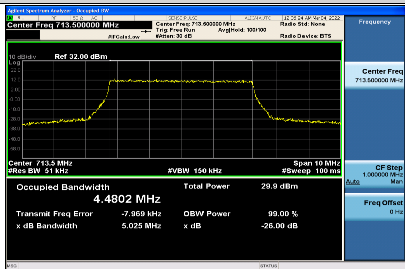
Band17-5MHz-QPSK-23825-25RB#0-4.4802
