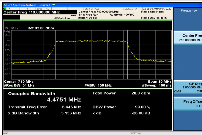
Band17-5MHz-16QAM-23790-25RB#0-4.4751
