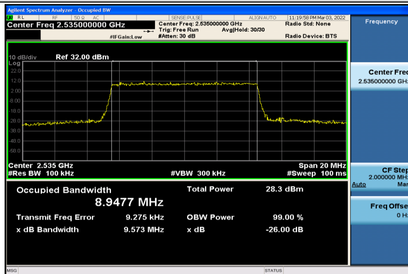
Band7-10MHz-16QAM-21100-50RB#0-8.9477
