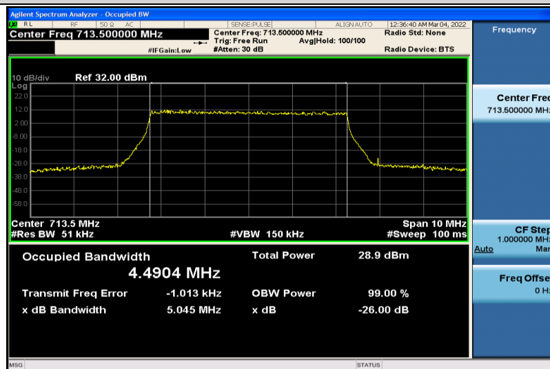
Band17-5MHz-16QAM-23825-25RB#0-4.4904
