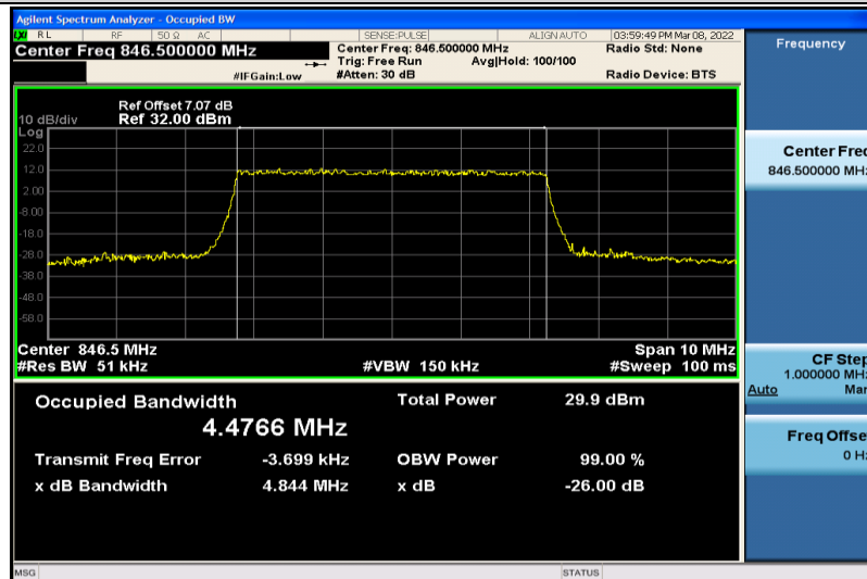
Band5-5MHz-64QAM-20625-25RB#0-4.4766
