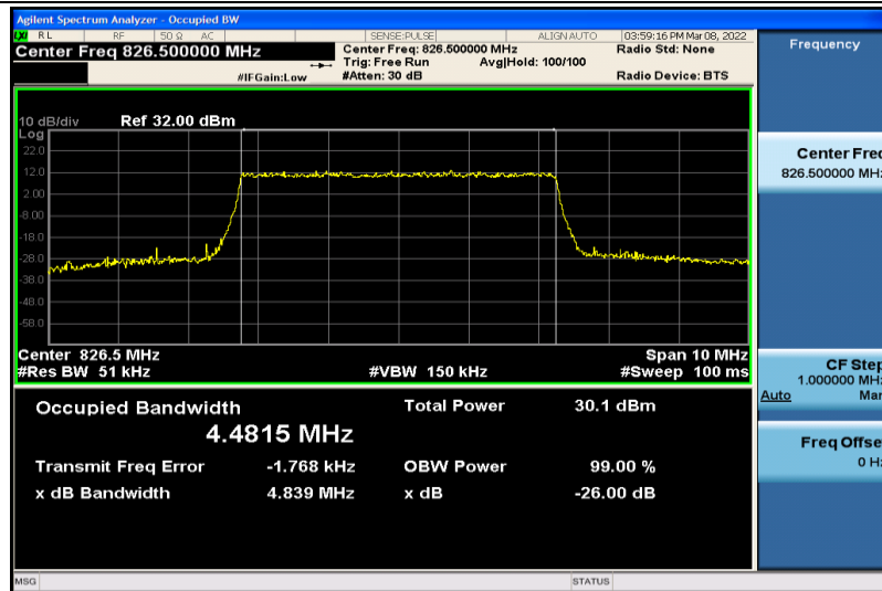
Band5-5MHz-64QAM-20425-25RB#0-4.4815
