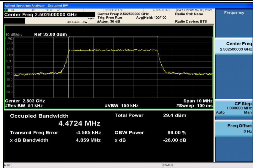
Band7-5MHz-64QAM-20775-25RB#0-4.4724
