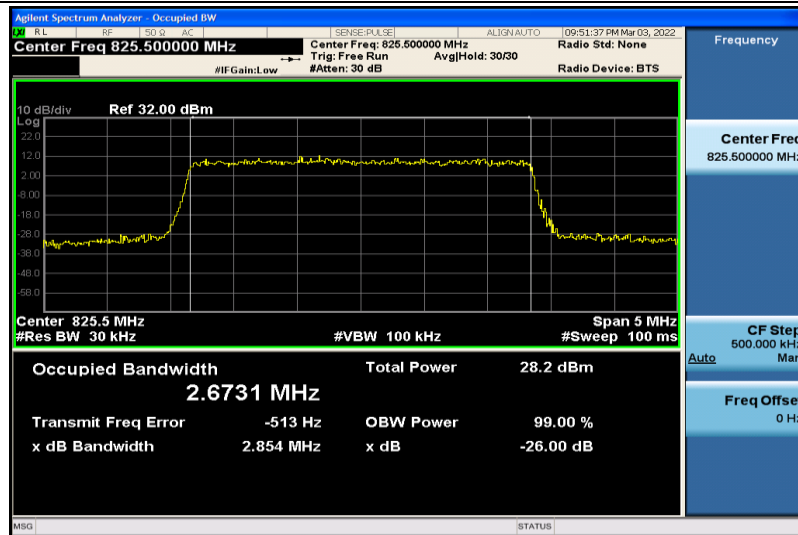
Band5-3MHz-16QAM-20415-15RB#0-2.6731
