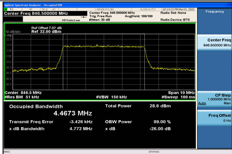
Band5-5MHz-16QAM-20625-25RB#0-4.4673
