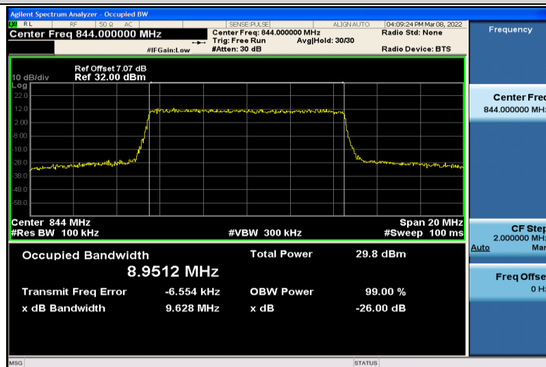
Band5-10MHz-64QAM-20600-50RB#0-8.9512
