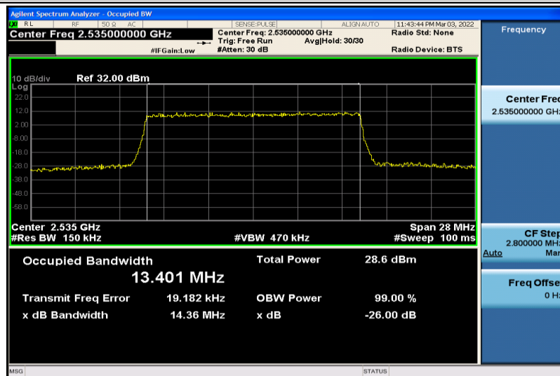
Band7-15MHz-16QAM-21100-75RB#0-13.401
