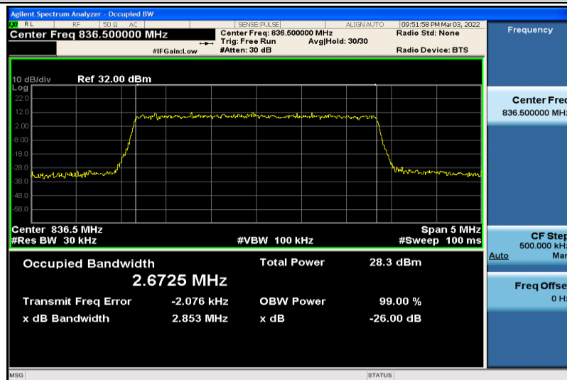
Band5-3MHz-16QAM-20525-15RB#0-2.6725
