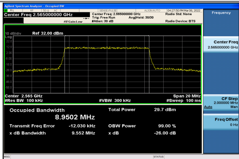
Band7-10MHz-64QAM-21400-50RB#0-8.9502
