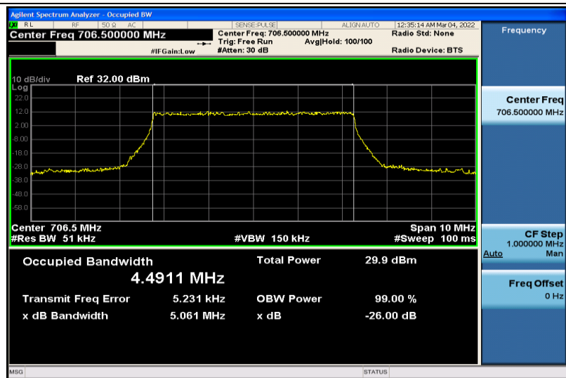
Band17-5MHz-QPSK-23755-25RB#0-4.4911
