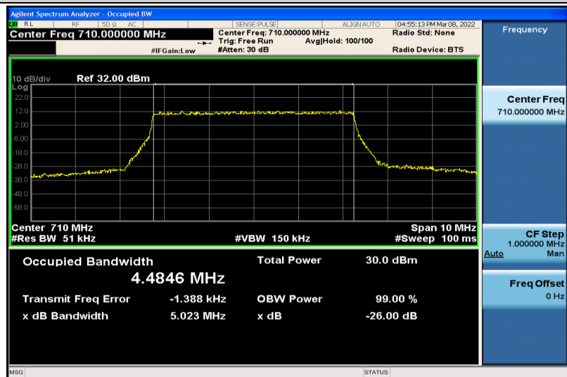
Band17-5MHz-64QAM-23790-25RB#0-4.4846
