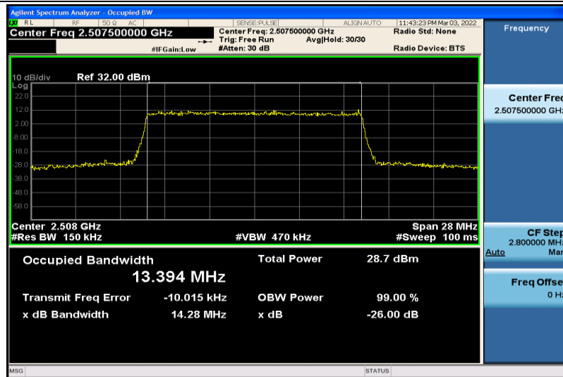
Band7-15MHz-16QAM-20825-75RB#0-13.394
