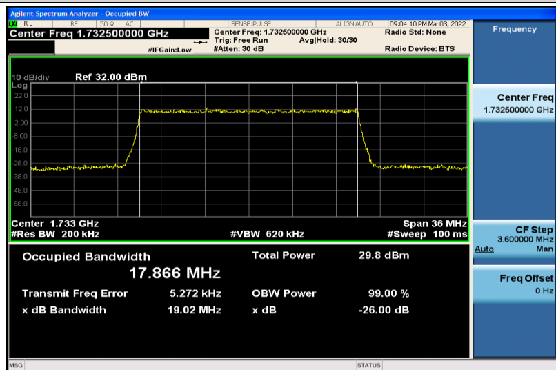
Band4-20MHz-QPSK-20175-100RB#0-17.866
