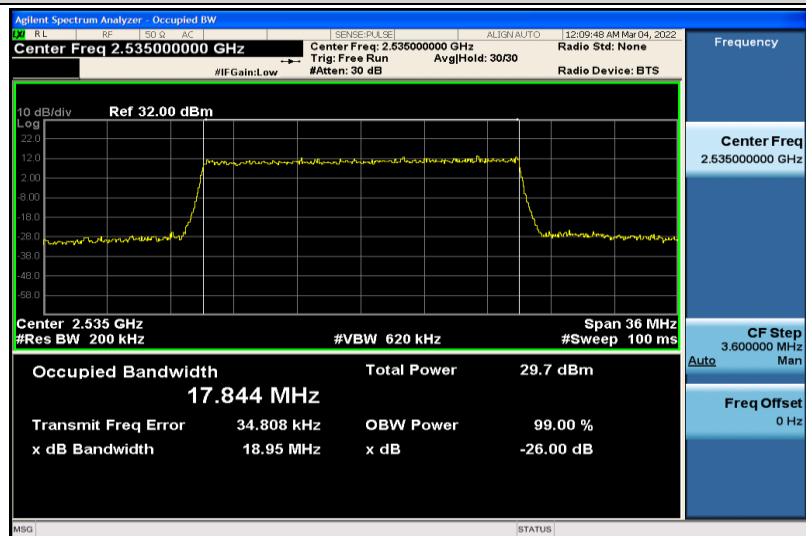
Band7-20MHz-QPSK-21100-100RB#0-17.844
