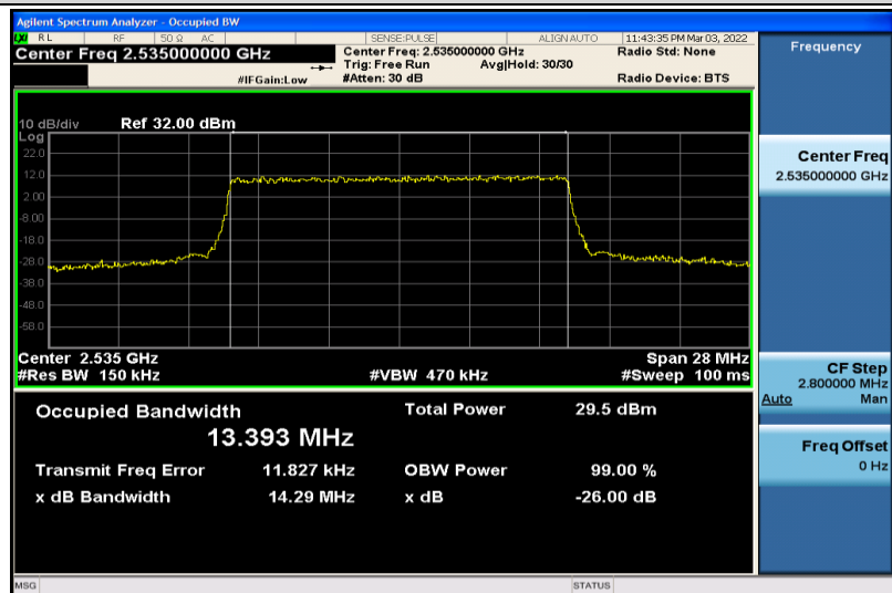
Band7-15MHz-QPSK-21100-75RB#0-13.393
