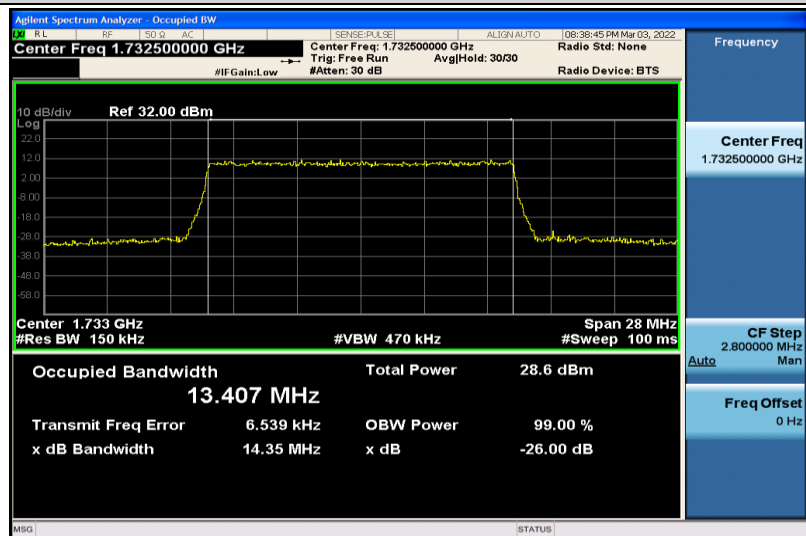
Band4-15MHz-16QAM-20175-75RB#0-13.407
