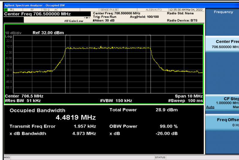
Band17-5MHz-16QAM-23755-25RB#0-4.4819
