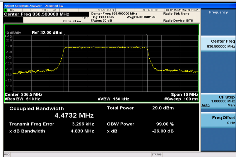
Band5-5MHz-16QAM-20525-25RB#0-4.4732
