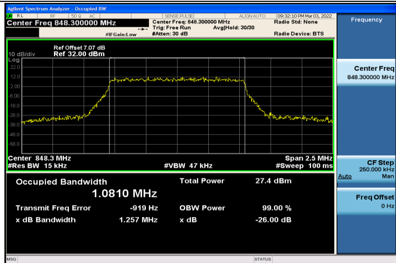
Band5-1.4MHz-16QAM-20643-6RB#0-1.0810
