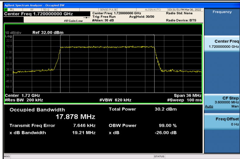
Band4-20MHz-64QAM-20050-100RB#0-17.878
