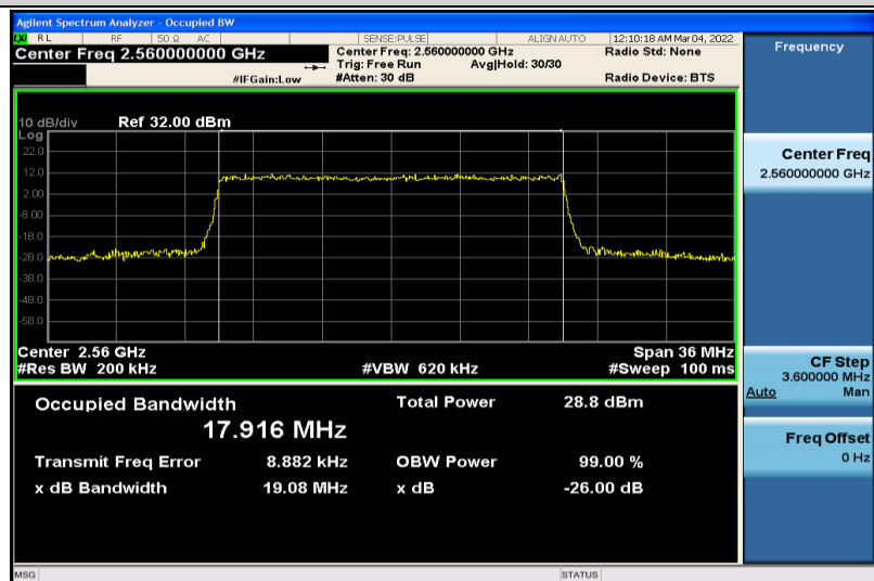
Band7-20MHz-16QAM-21350-100RB#0-17.916
