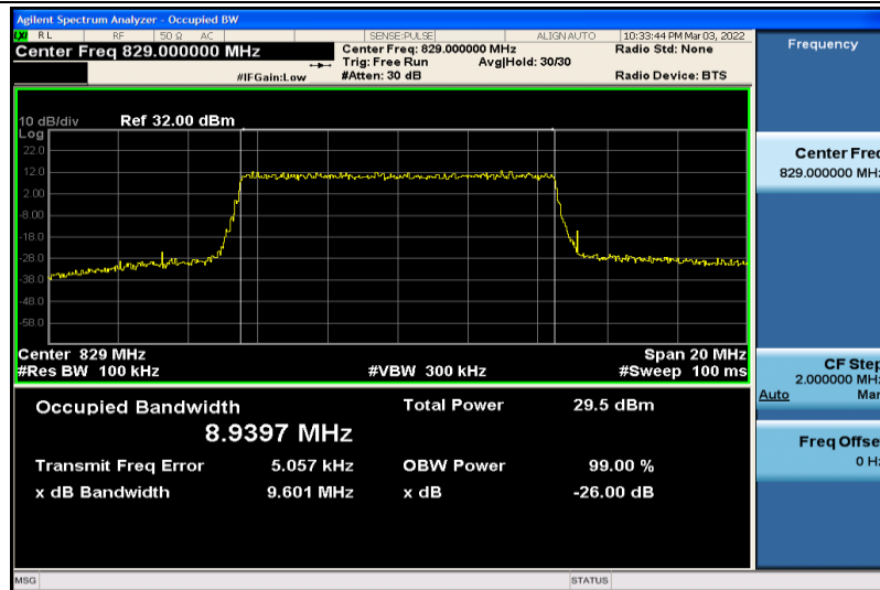
Band5-10MHz-QPSK-20450-50RB#0-8.9397
