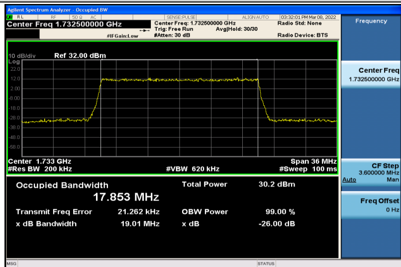
Band4-20MHz-64QAM-20175-100RB#0-17.853
