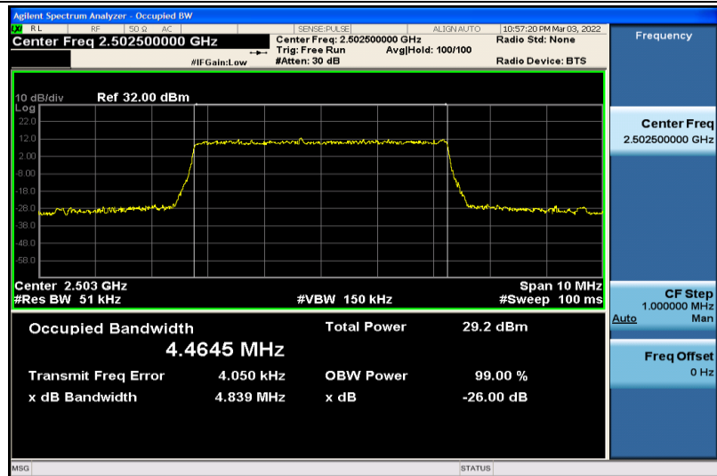
Band7-5MHz-QPSK-20775-25RB#0-4.4645
