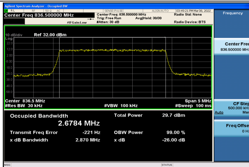
Band5-3MHz-64QAM-20525-15RB#0-2.6784
