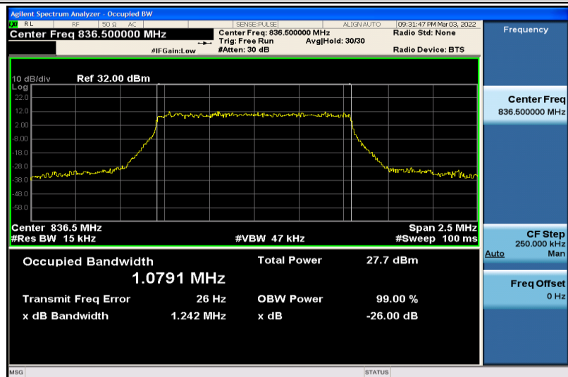
Band5-1.4MHz-16QAM-20525-6RB#0-1.0791
