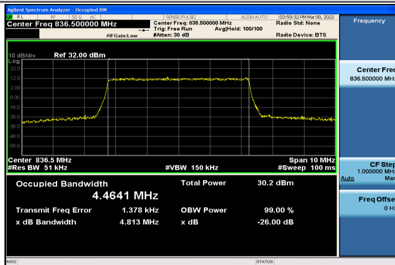
Band5-5MHz-64QAM-20525-25RB#0-4.4641
