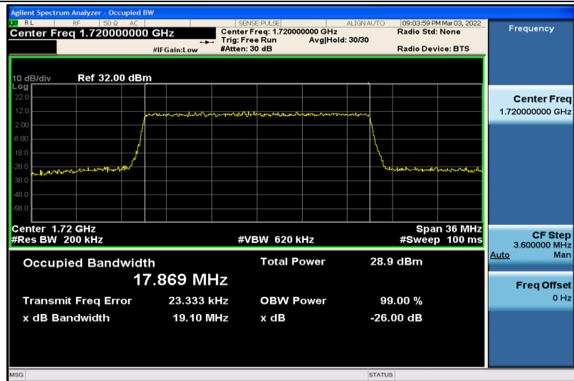
Band4-20MHz-16QAM-20050-100RB#0-17.869
