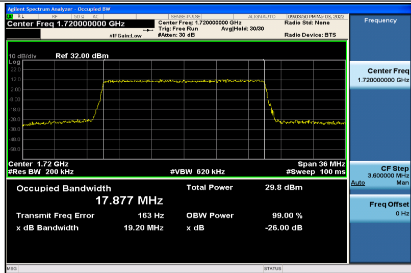
Band4-20MHz-QPSK-20050-100RB#0-17.877
