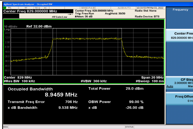
Band5-10MHz-16QAM-20450-50RB#0-8.9459
