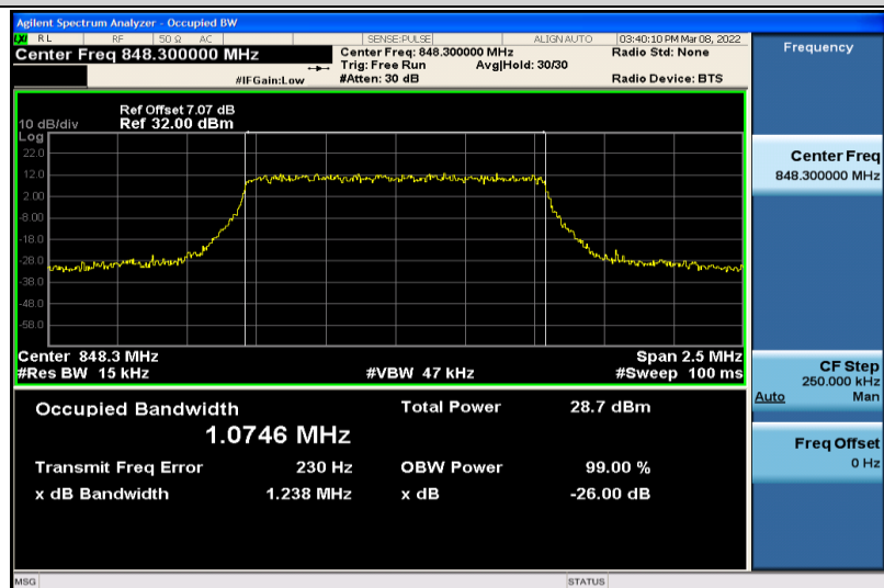
Band5-1.4MHz-64QAM-20643-6RB#0-1.0746
