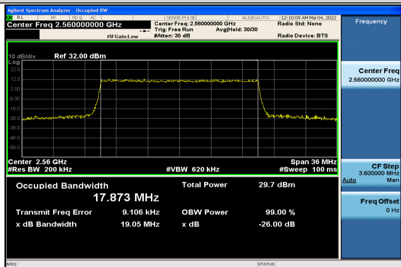
Band7-20MHz-QPSK-21350-100RB#0-17.873
