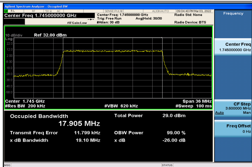
Band4-20MHz-16QAM-20300-100RB#0-17.905
