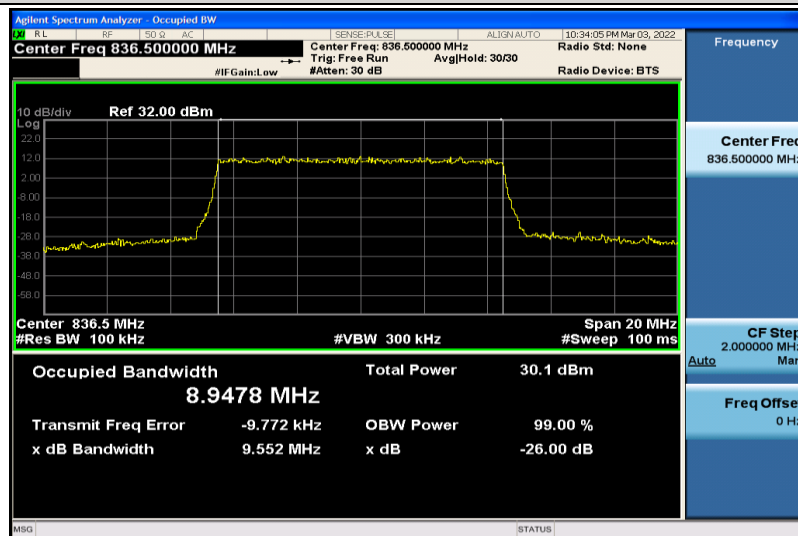
Band5-10MHz-QPSK-20525-50RB#0-8.9478
