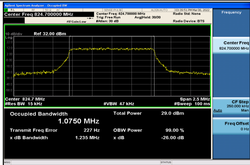
Band5-1.4MHz-64QAM-20407-6RB#0-1.0750
