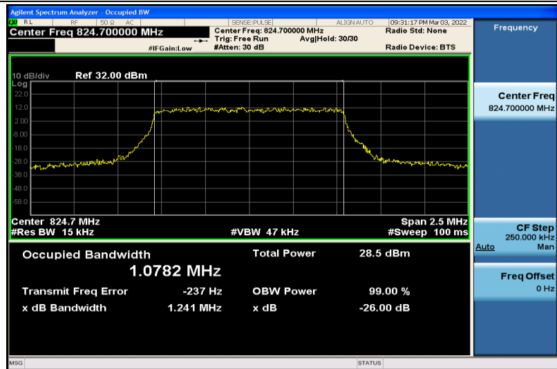
Band5-1.4MHz-QPSK-20407-6RB#0-1.0782
