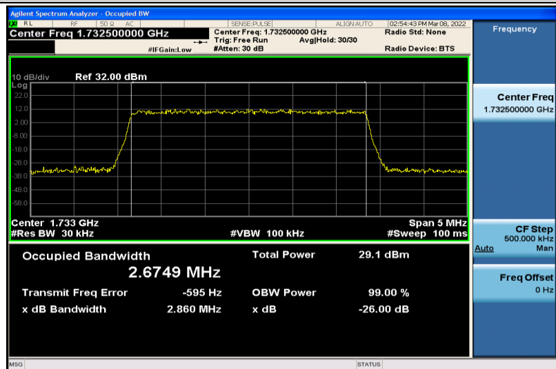
Band4-3MHz-64QAM-20175-15RB#0-2.6749
