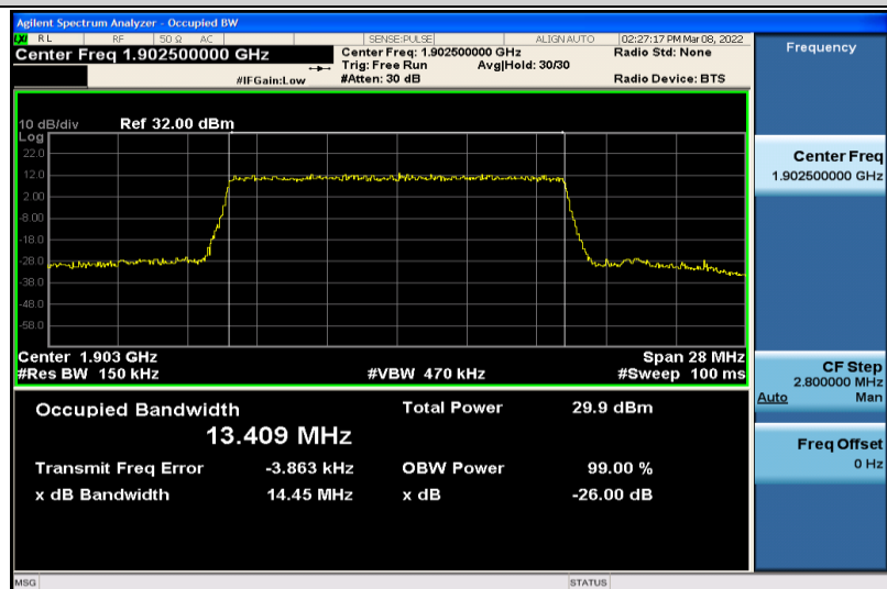
Band2-15MHz-64QAM-19125-75RB#0-13.409
