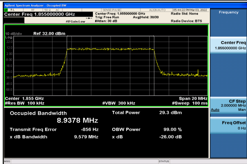
Band2-10MHz-QPSK-18650-50RB#0-8.9378
