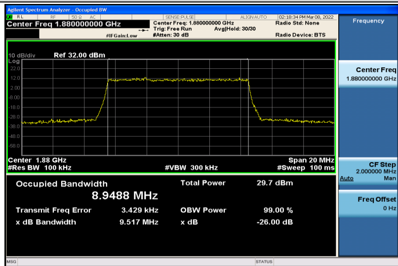
Band2-10MHz-64QAM-18900-50RB#0-8.9488
