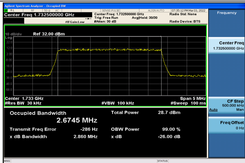
Band4-3MHz-QPSK-20175-15RB#0-2.6745
