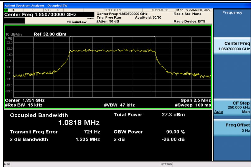
Band2-1.4MHz-64QAM-18607-6RB#0-1.0818
