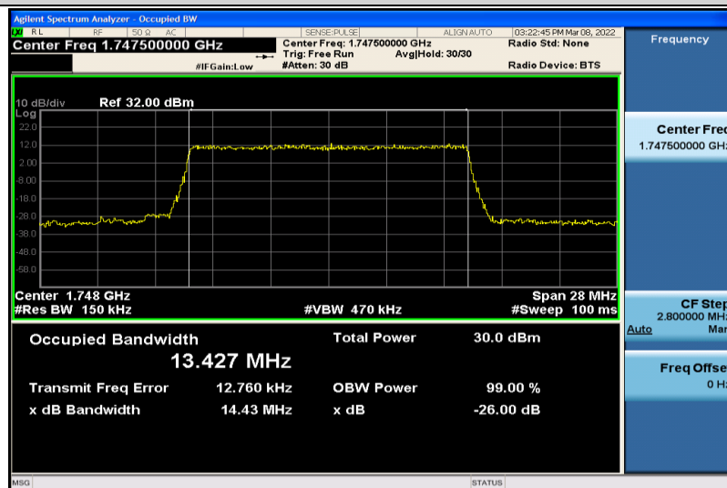
Band4-15MHz-64QAM-20325-75RB#0-13.427
