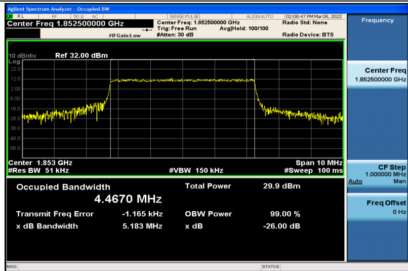
Band2-5MHz-64QAM-18625-25RB#0-4.4670
