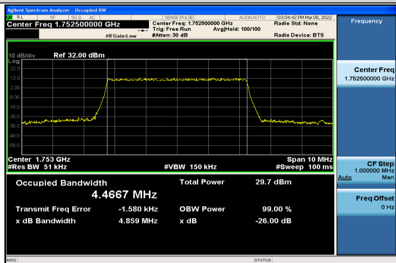
Band4-5MHz-64QAM-20375-25RB#0-4.4667
