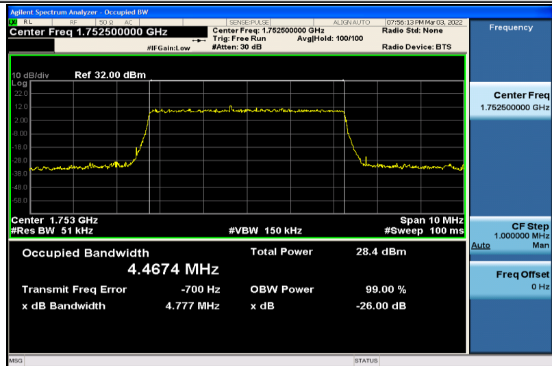
Band4-5MHz-16QAM-20375-25RB#0-4.4674
