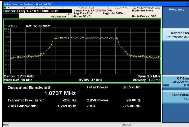
Band4-1.4MHz-64QAM-19957-6RB#0-1.0737
