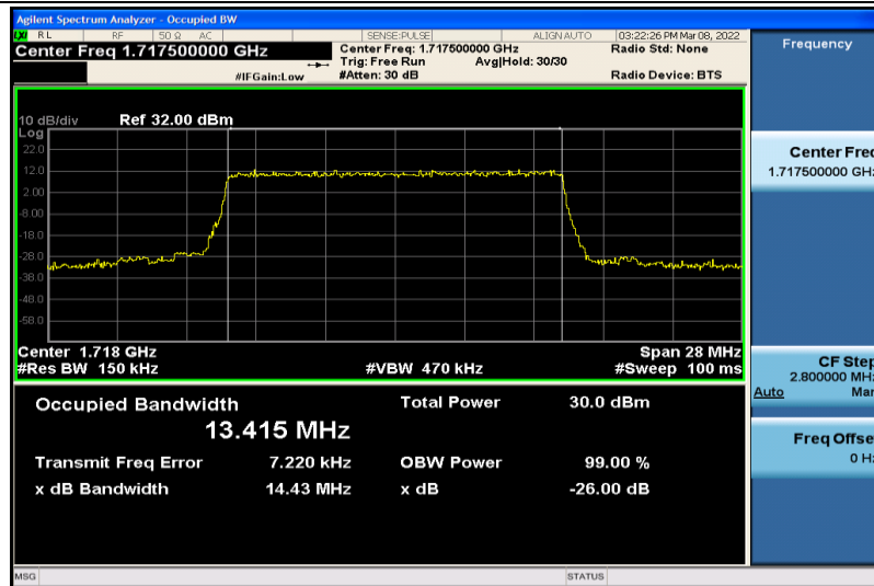
Band4-15MHz-64QAM-20025-75RB#0-13.415
