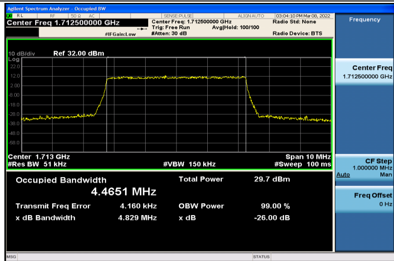
Band4-5MHz-64QAM-19975-25RB#0-4.4651
