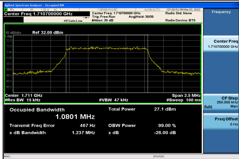
Band4-1.4MHz-16QAM-19957-6RB#0-1.0801
