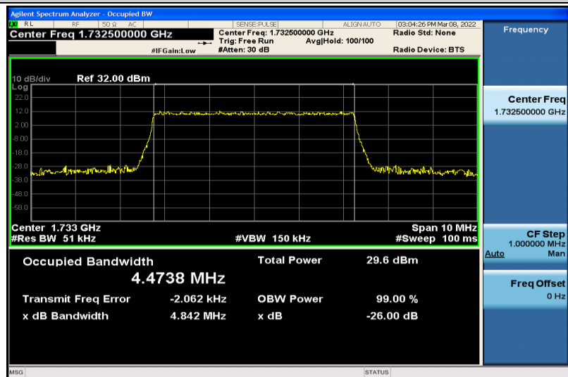
Band4-5MHz-64QAM-20175-25RB#0-4.4738
