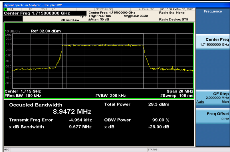
Band4-10MHz-QPSK-20000-50RB#0-8.9472
