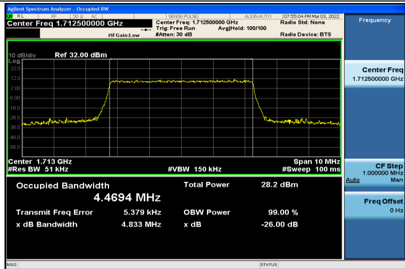
Band4-5MHz-16QAM-19975-25RB#0-4.4694
