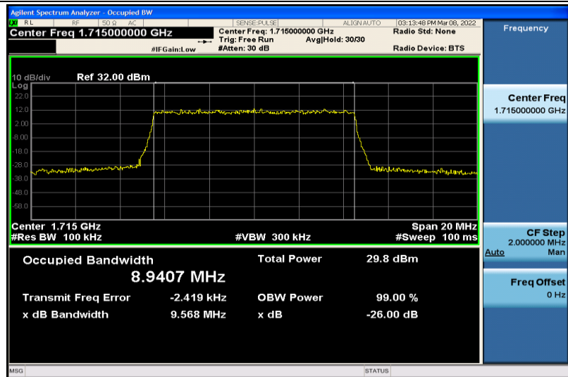
Band4-10MHz-64QAM-20000-50RB#0-8.9407
