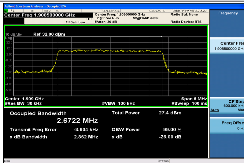
Band2-3MHz-16QAM-19185-15RB#0-2.6722
