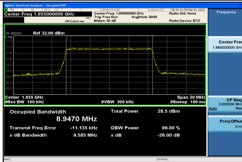
Band2-10MHz-16QAM-18650-50RB#0-8.9470
