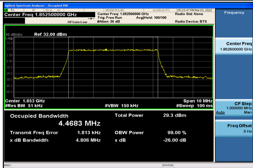
Band2-5MHz-QPSK-18625-25RB#0-4.4683
