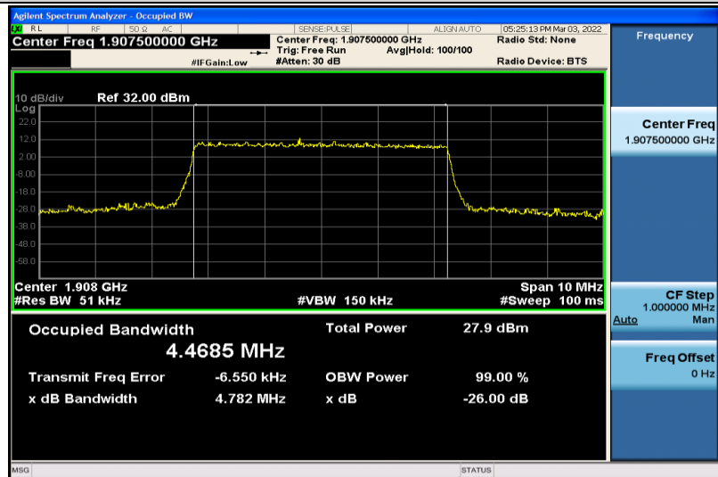
Band2-5MHz-16QAM-19175-25RB#0-4.4685
