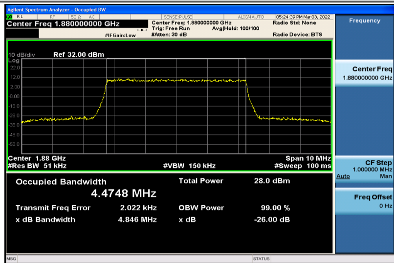
Band2-5MHz-16QAM-18900-25RB#0-4.4748
