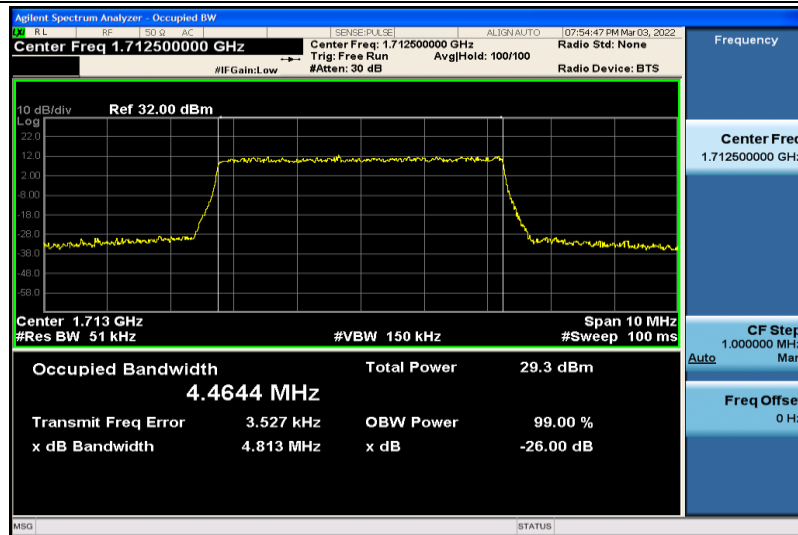
Band4-5MHz-QPSK-19975-25RB#0-4.4644
