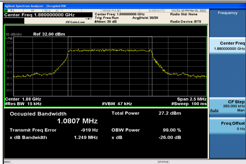
Band2-1.4MHz-64QAM-18900-6RB#0-1.0807
