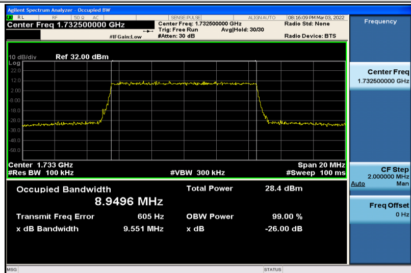
Band4-10MHz-16QAM-20175-50RB#0-8.9496
