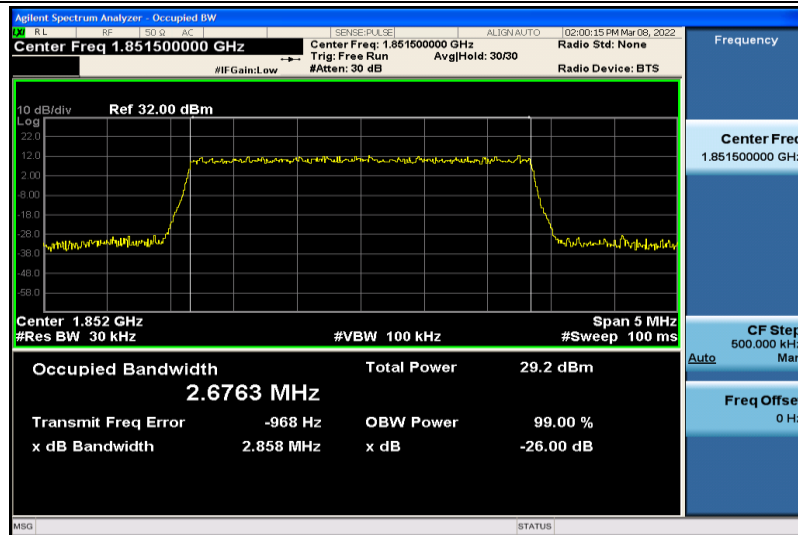
Band2-3MHz-64QAM-18615-15RB#0-2.6763
