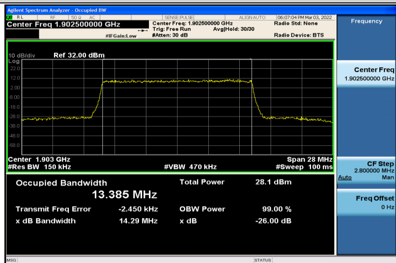
Band2-15MHz-16QAM-19125-75RB#0-13.385
