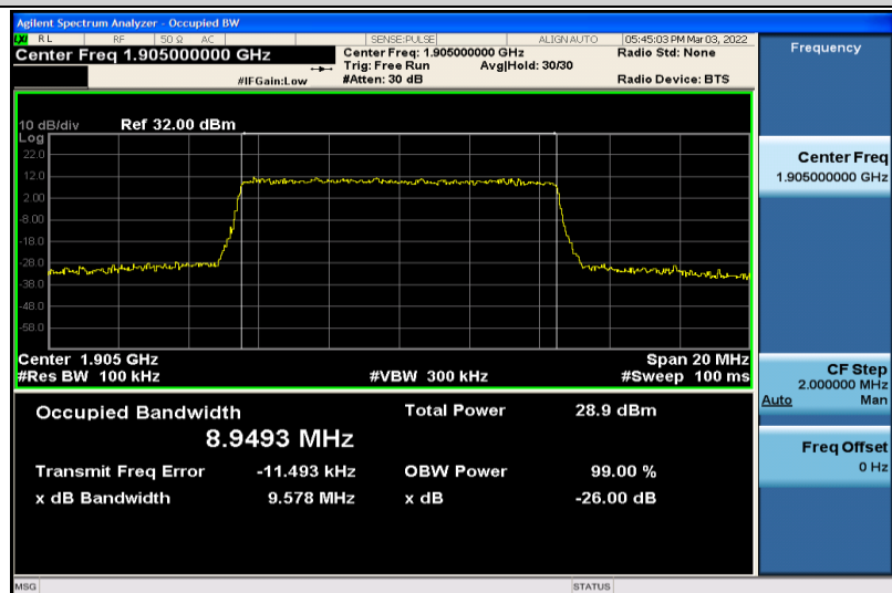
Band2-10MHz-QPSK-19150-50RB#0-8.9493
