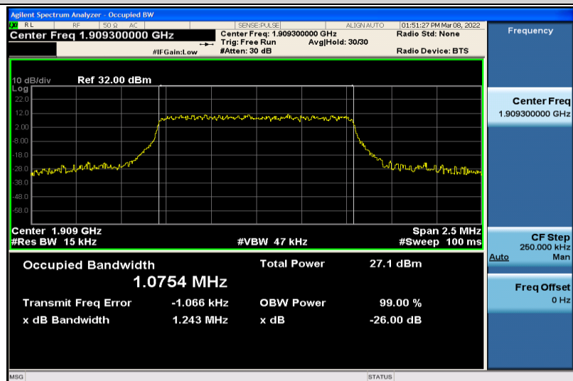
Band2-1.4MHz-64QAM-19193-6RB#0-1.0754
