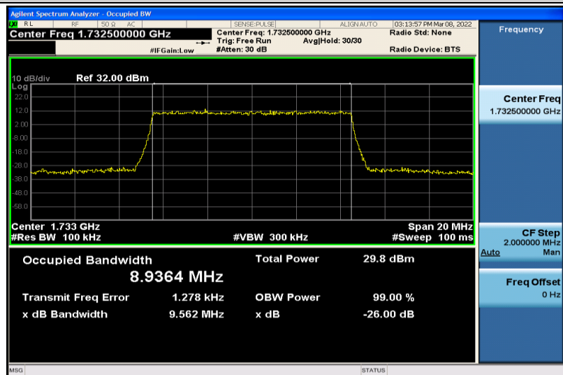
Band4-10MHz-64QAM-20175-50RB#0-8.9364
