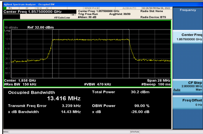
Band2-15MHz-64QAM-18675-75RB#0-13.416
