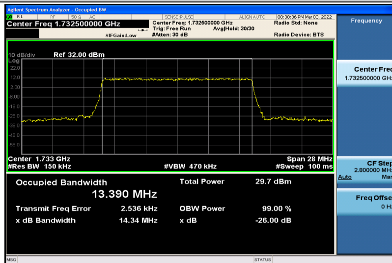
Band4-15MHz-QPSK-20175-75RB#0-13.390
