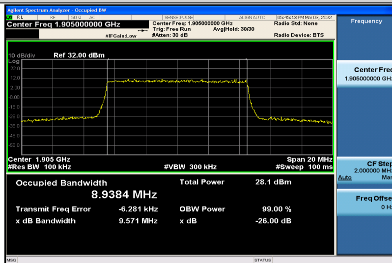
Band2-10MHz-16QAM-19150-50RB#0-8.9384
