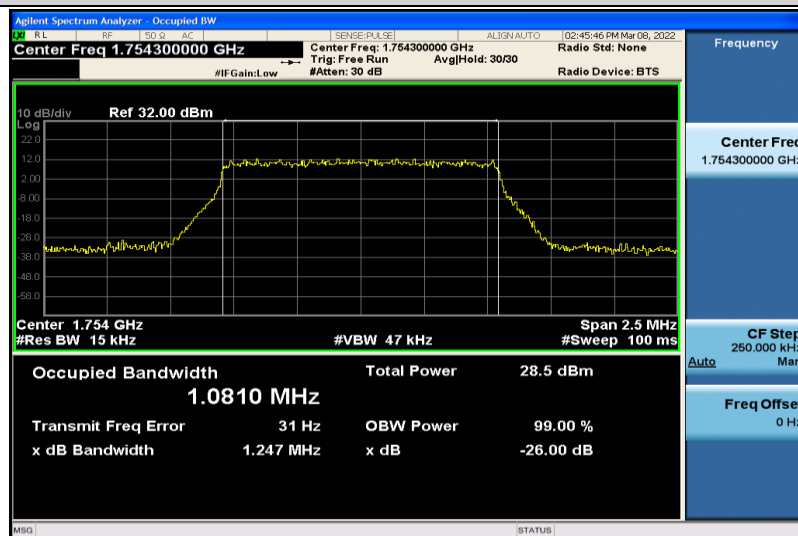
Band4-1.4MHz-64QAM-20393-6RB#0-1.0810
