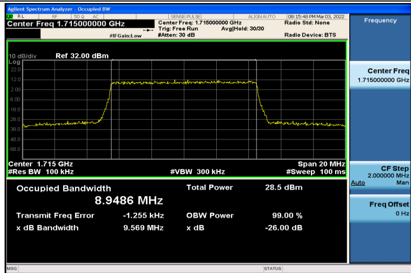
Band4-10MHz-16QAM-20000-50RB#0-8.9486
