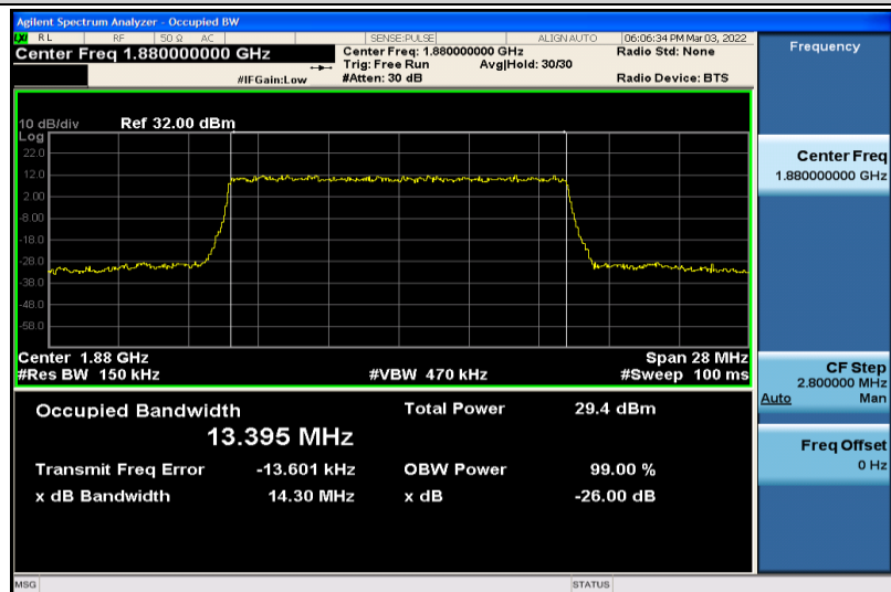
Band2-15MHz-QPSK-18900-75RB#0-13.395
