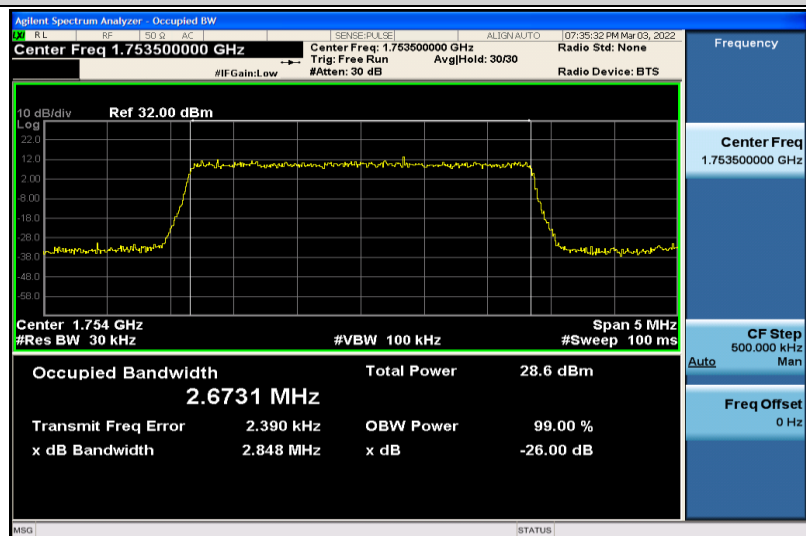
Band4-3MHz-QPSK-20385-15RB#0-2.6731
