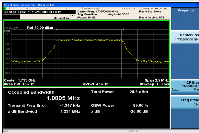
Band4-1.4MHz-64QAM-20175-6RB#0-1.0805
