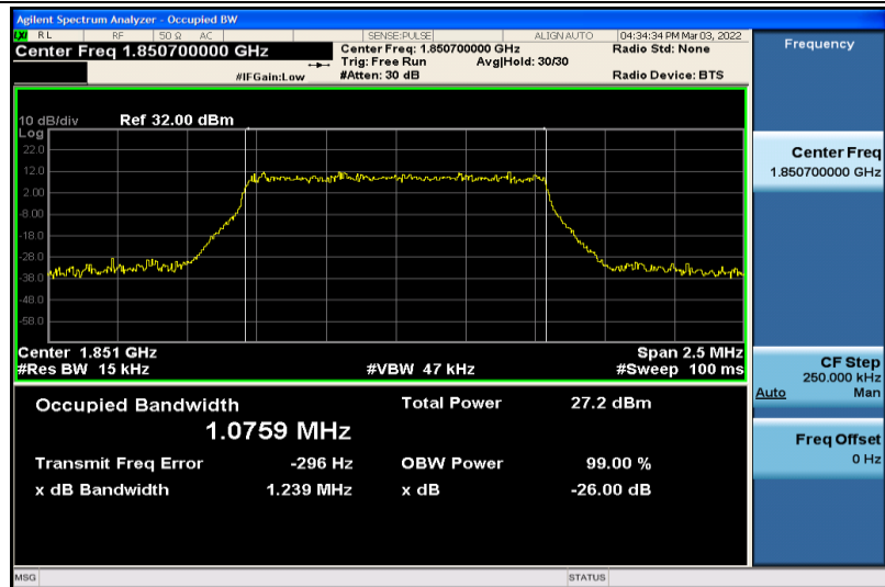
Band2-1.4MHz-16QAM-18607-6RB#0-1.0759
