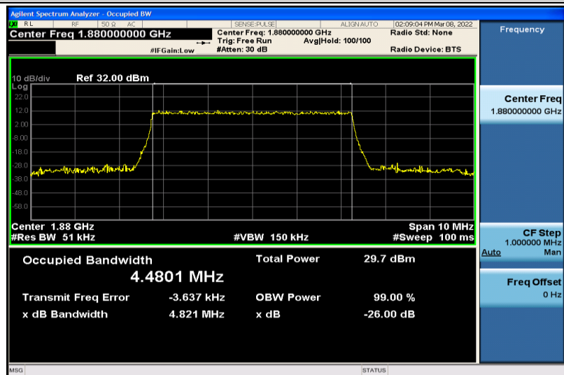
Band2-5MHz-64QAM-18900-25RB#0-4.4801
