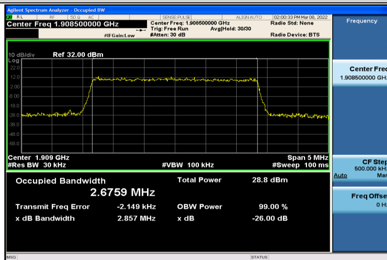
Band2-3MHz-64QAM-19185-15RB#0-2.6759
