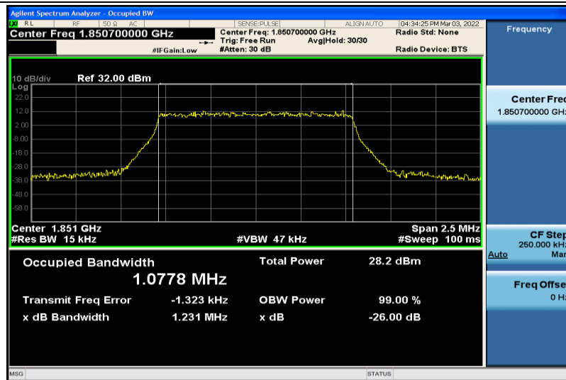
Band2-1.4MHz-QPSK-18607-6RB#0-1.0778
