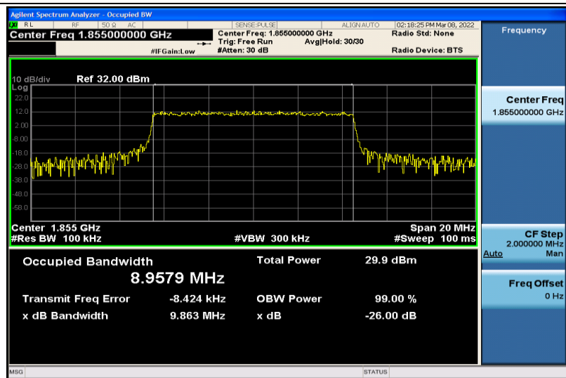
Band2-10MHz-64QAM-18650-50RB#0-8.9579
