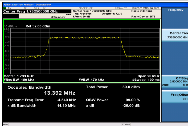
Band4-15MHz-64QAM-20175-75RB#0-13.392
