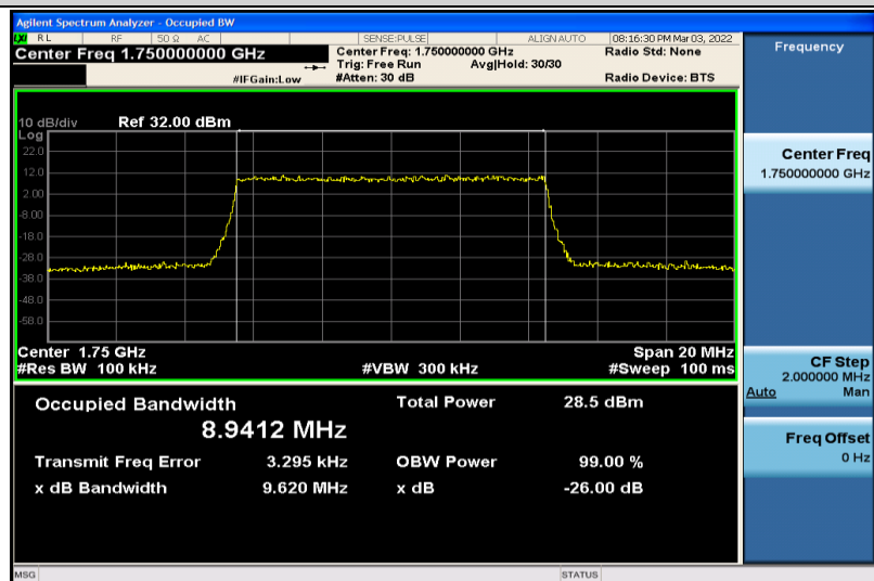
Band4-10MHz-16QAM-20350-50RB#0-8.9412
