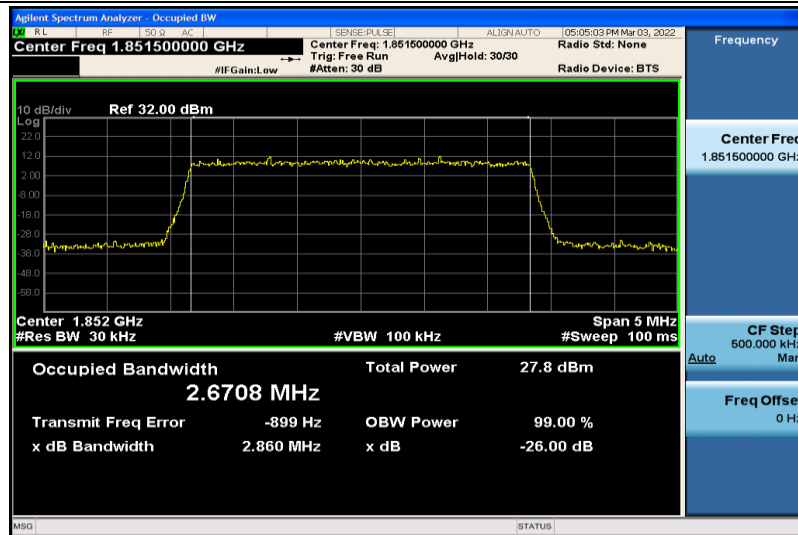
Band2-3MHz-16QAM-18615-15RB#0-2.6708
