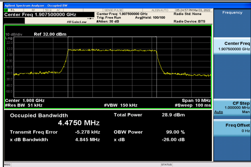
Band2-5MHz-QPSK-19175-25RB#0-4.4750
