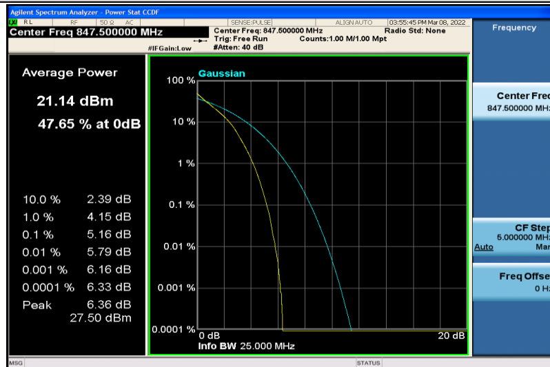
Band5-3MHz-64QAM-20635-15RB#0
