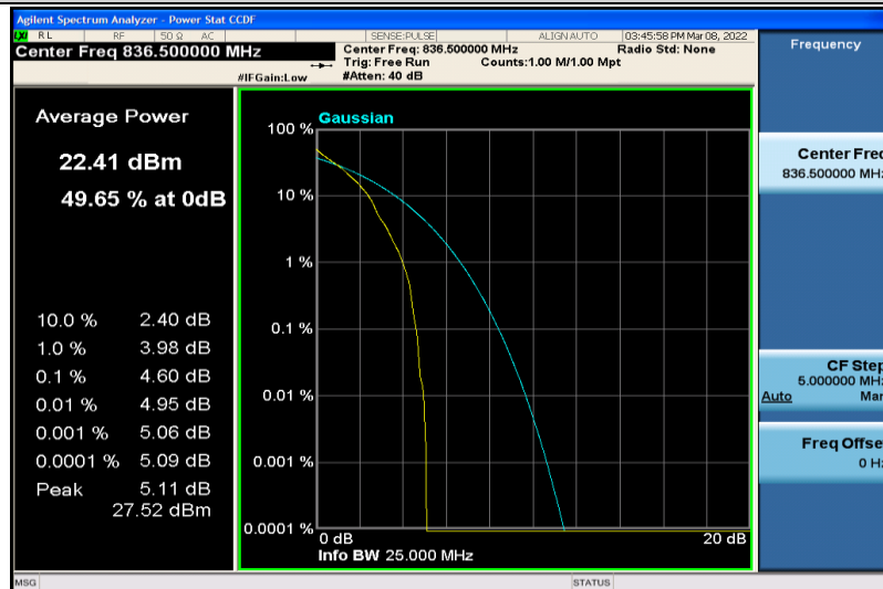
Band5-1.4MHz-64QAM-20525-1RB#0
