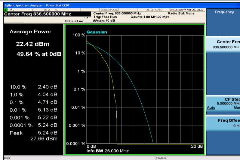
Band5-10MHz-64QAM-20525-1RB#0
