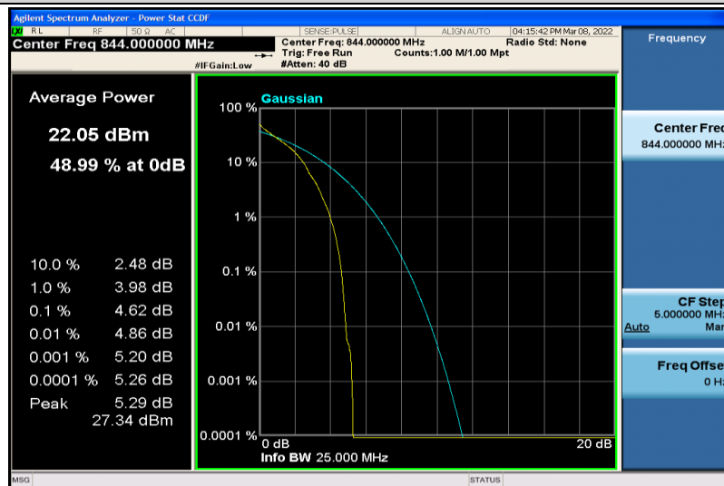
Band5-10MHz-64QAM-20600-1RB#0
