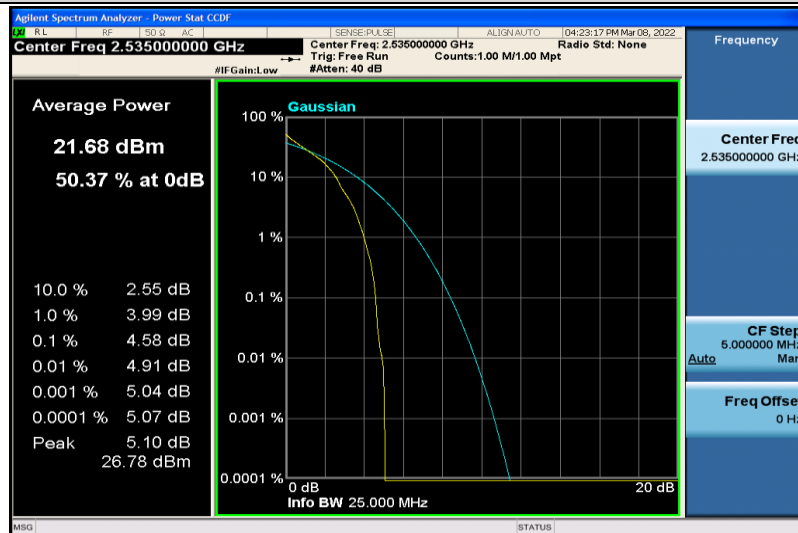
Band7-5MHz-64QAM-21100-1RB#0
