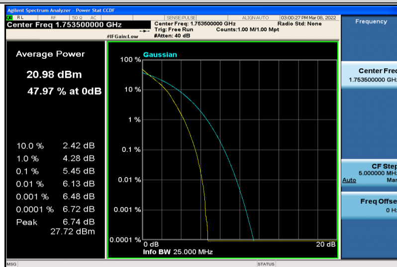
Band4-3MHz-64QAM-20385-15RB#0
