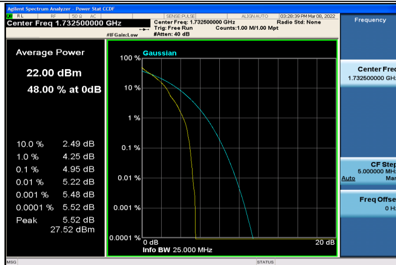
Band4-15MHz-64QAM-20175-1RB#0
