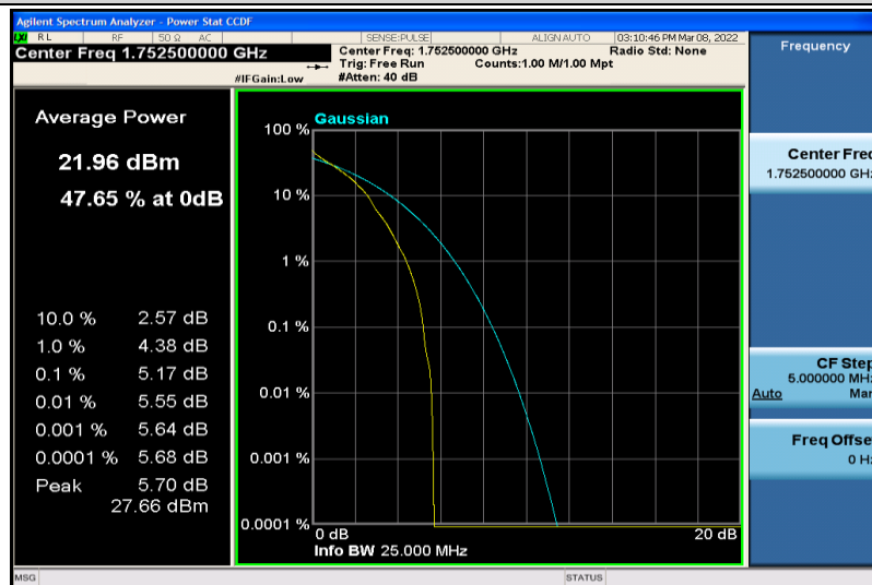
Band4-5MHz-64QAM-20375-1RB#0
