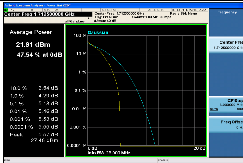
Band4-5MHz-64QAM-19975-1RB#0
