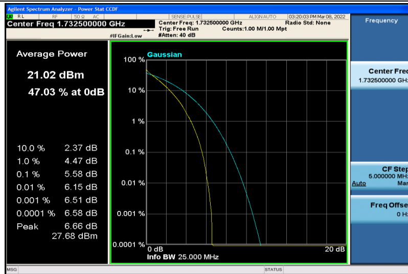
Band4-10MHz-64QAM-20175-50RB#0
