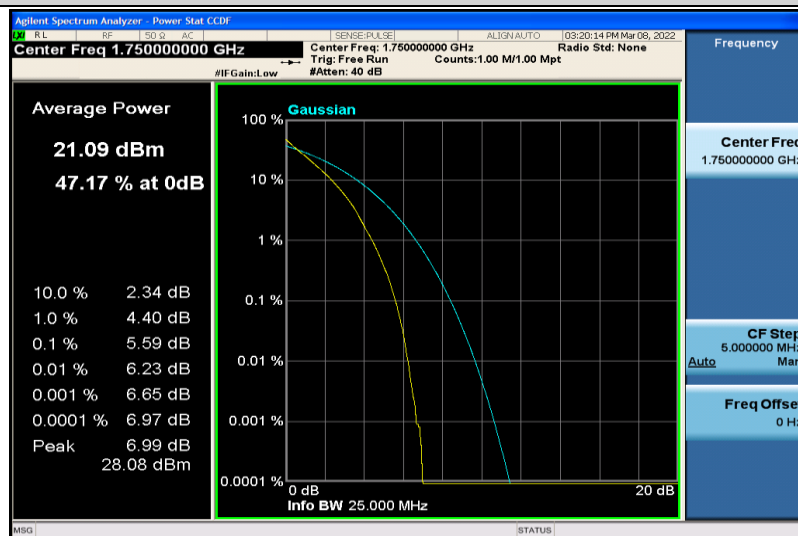
Band4-10MHz-64QAM-20350-50RB#0
