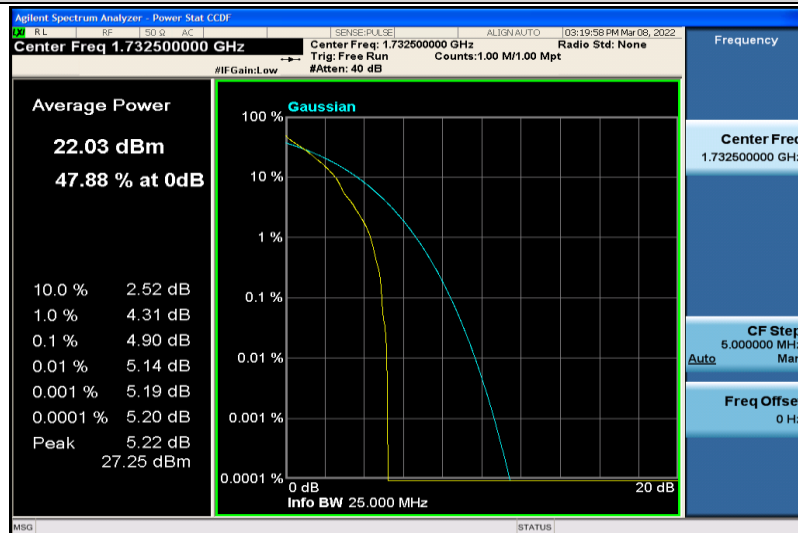
Band4-10MHz-64QAM-20175-1RB#0
