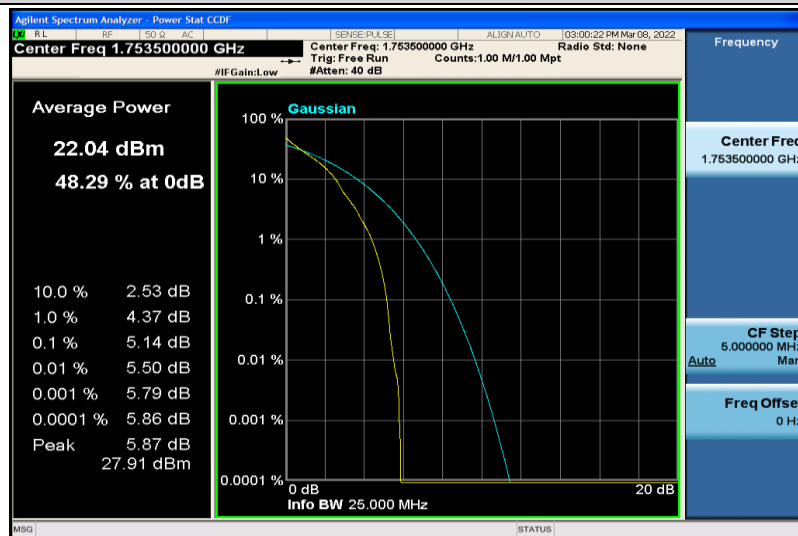
Band4-3MHz-64QAM-20385-1RB#0
