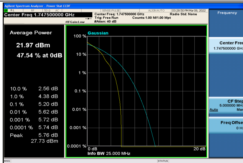
Band4-15MHz-64QAM-20325-1RB#0
