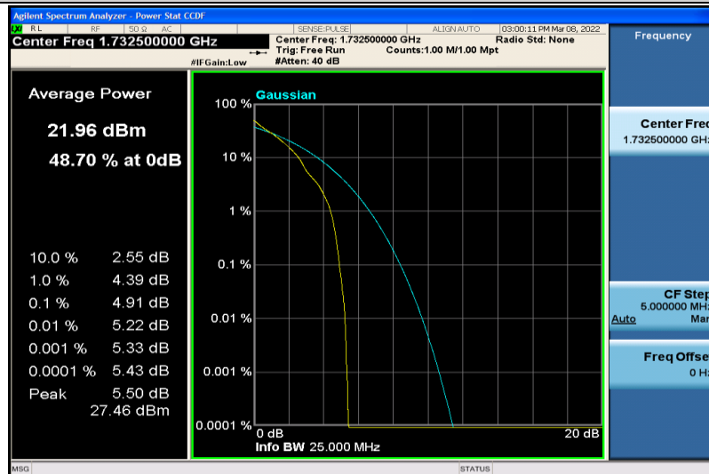
Band4-3MHz-64QAM-20175-1RB#0
