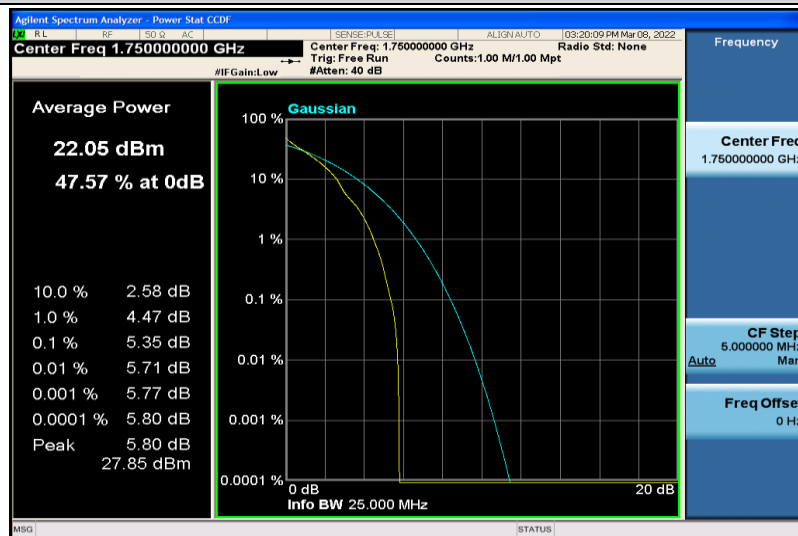
Band4-10MHz-64QAM-20350-1RB#0
