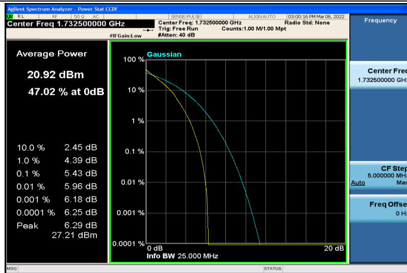
Band4-3MHz-64QAM-20175-15RB#0
