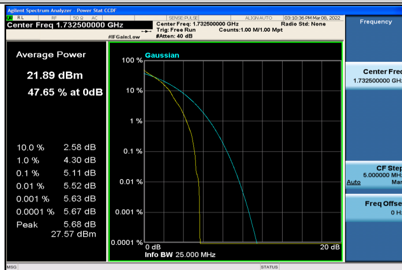
Band4-5MHz-64QAM-20175-1RB#0
