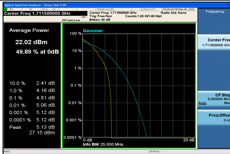
Band4-3MHz-64QAM-19965-1RB#0
