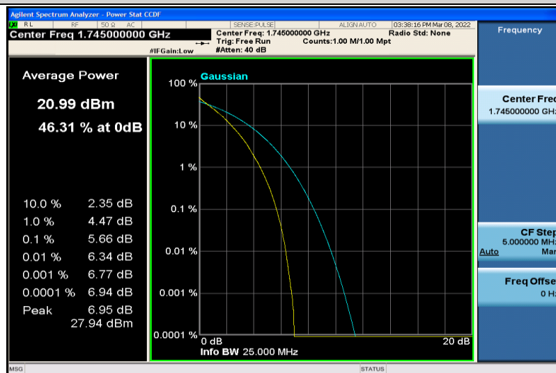
Band4-20MHz-64QAM-20300-100RB#0
