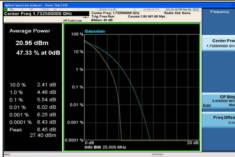
Band4-5MHz-64QAM-20175-25RB#0
