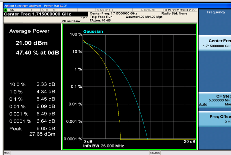
Band4-10MHz-64QAM-20000-50RB#0
