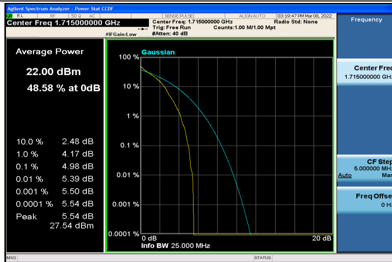
Band4-10MHz-64QAM-20000-1RB#0
