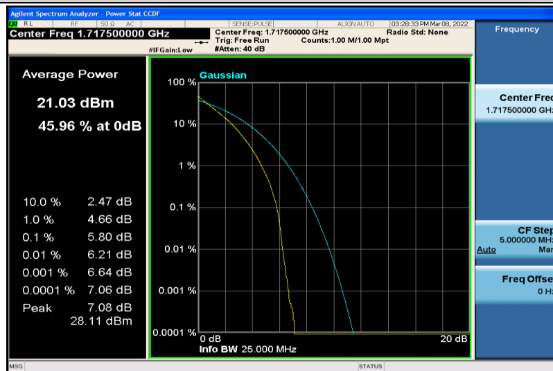
Band4-15MHz-64QAM-20025-75RB#0
