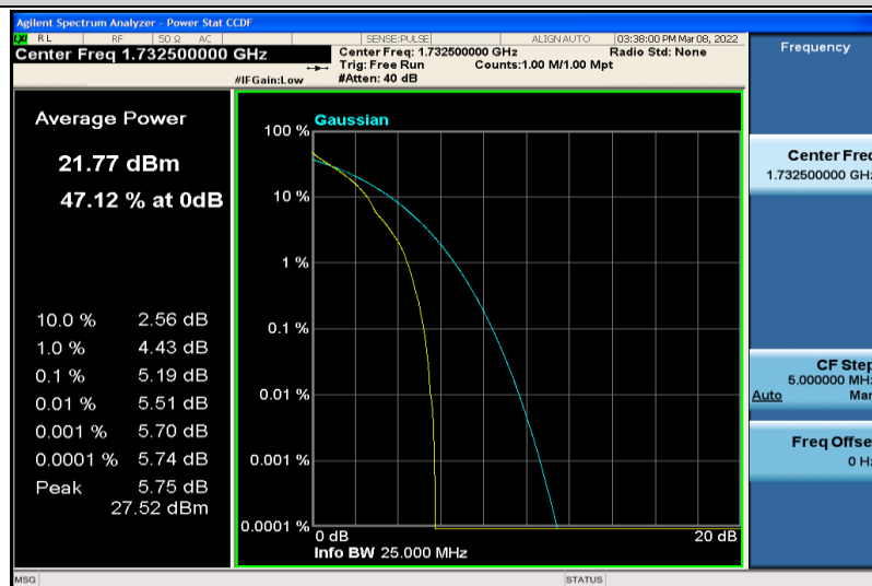
Band4-20MHz-64QAM-20175-1RB#0
